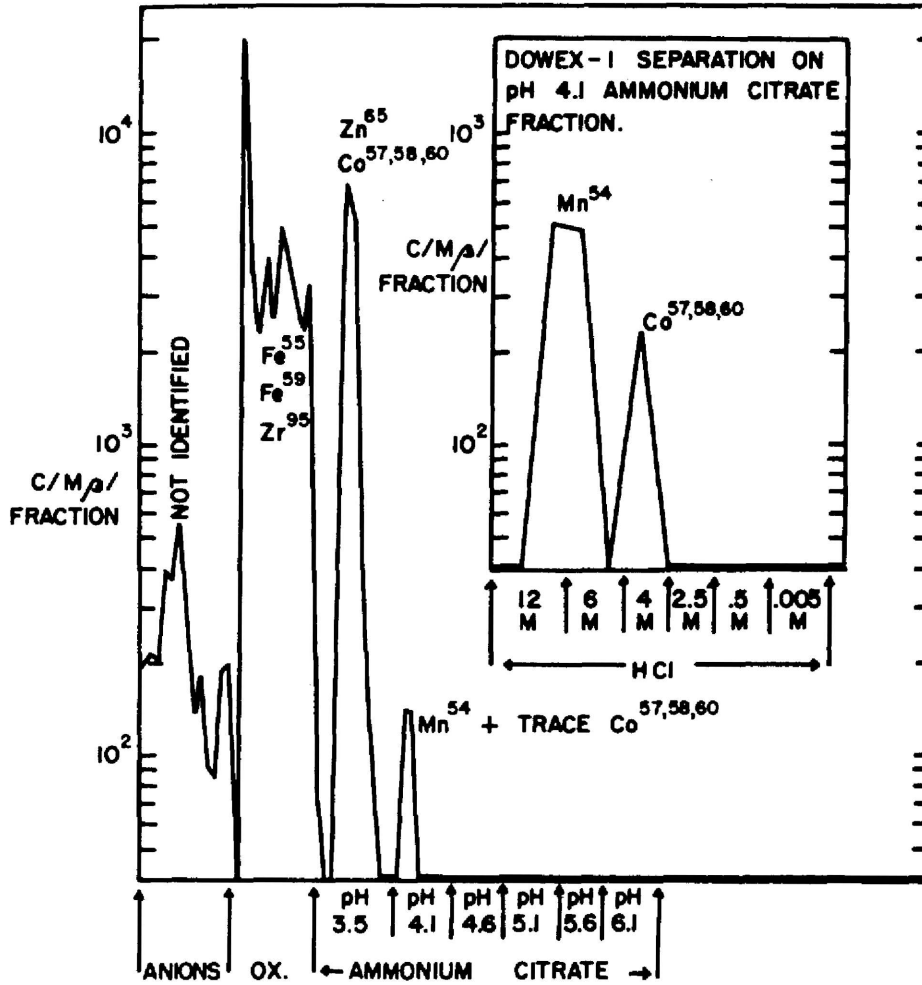
Fig. 6 Elution curve for bonito liver sample II, Fox Island, Bikini Atoll, September 23, 1956, from a Dowex 50 cationic resin column and the elution curve for a further elution of the pH 4.1 fraction from a Dowex 1 anionic resin column.
