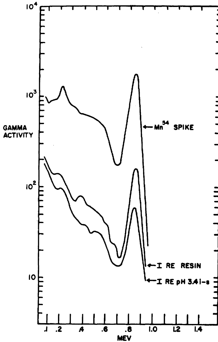
Fig. 5 Gamma spectrum curves on the I-RE 3.4 i-s fraction (second elution) and on the I-RE resin from clam kidney sample I eluted twice on Dowex-50. The gamma spectrum curve for a Mn 54 spike is also shown.
