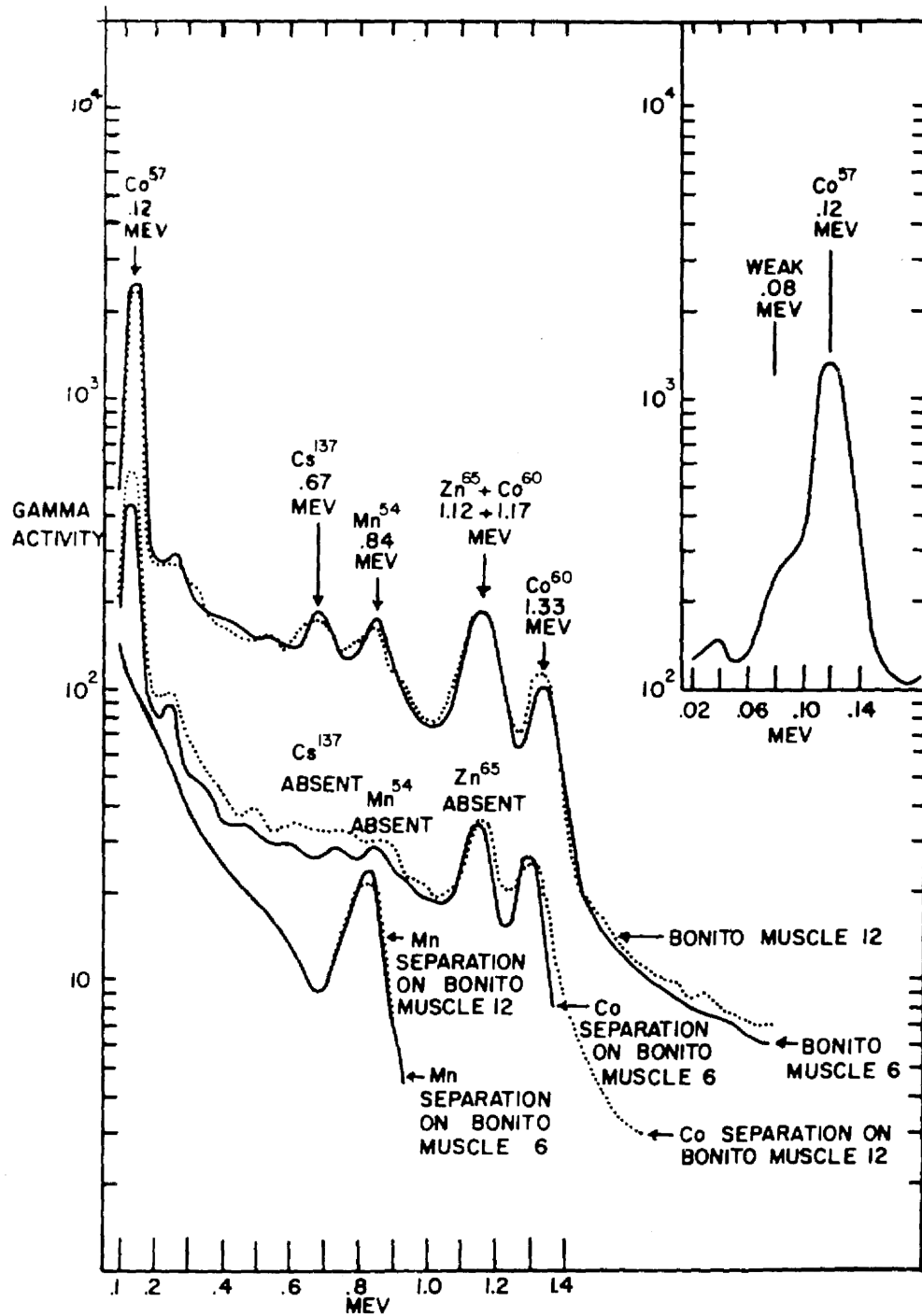
Fig. 8 Gamma spectrum curves on whole samples of bonito muscle from Eniwetok Atoll, November 26 and 27, 1954, and on cobalt and manganese chemical separations made on the muscle samples.
