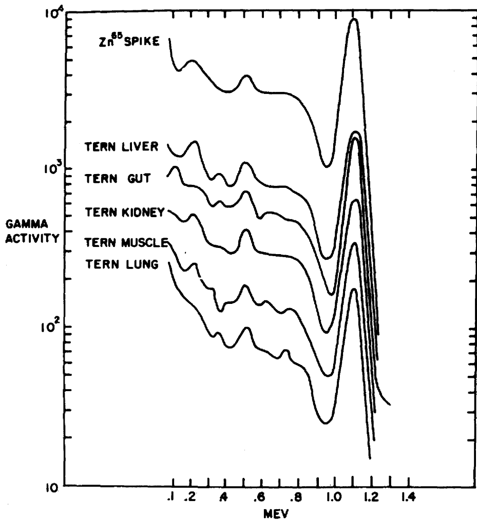
Fig. 14 Gamma spectrum curves for tern muscle, lung, kidney, liver and gut, Eniwetok Atoll, March, June, 1954. Gamma spectra made March 1957. A gamma spectrum curve for a Zn 65 spike is also shown.
