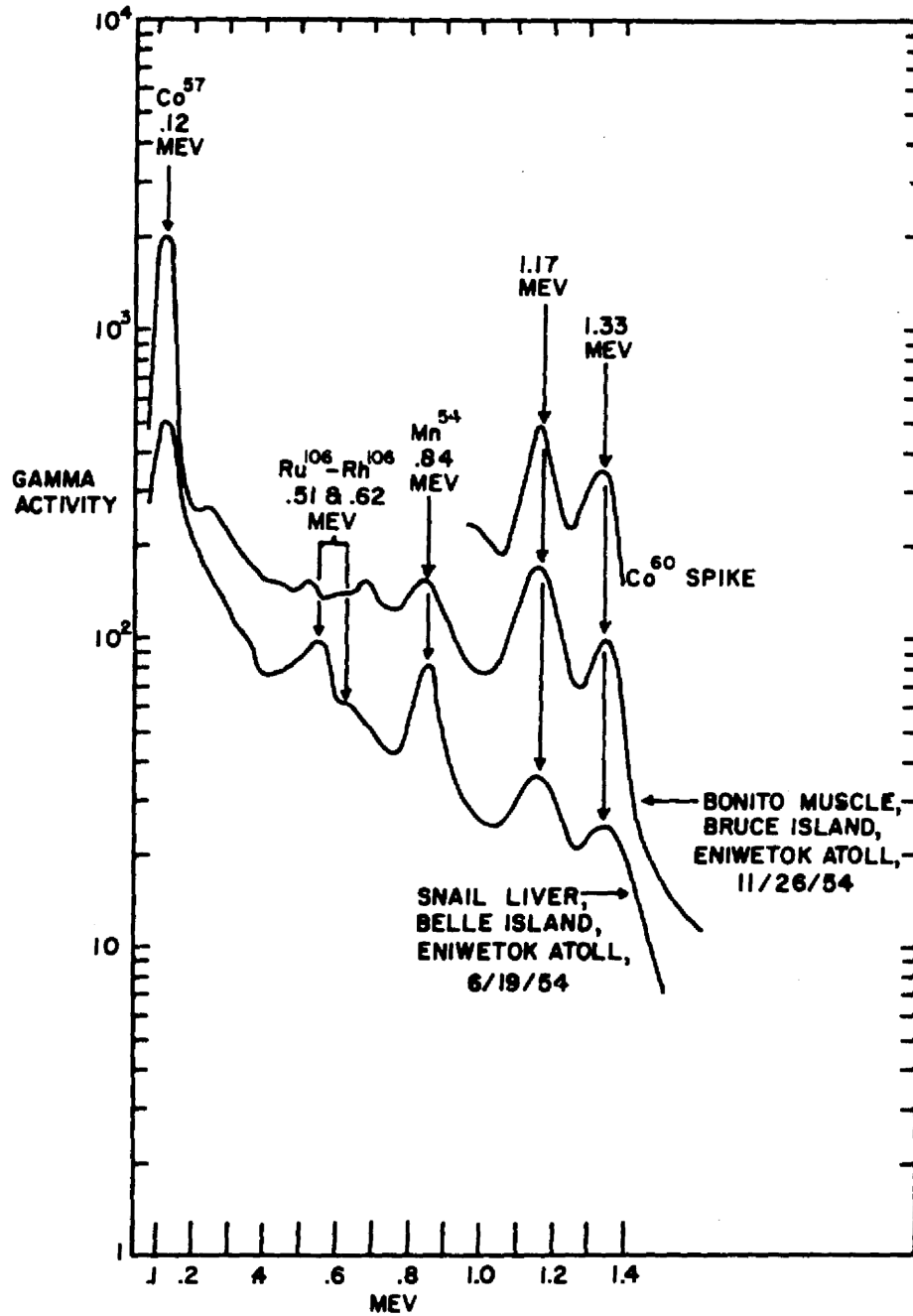
Fig. 10 Gamma spectra on bonito muscle and snail liver showing the gamma peaks of Mn 54 , Co 57 and Co 60 . The gamma peaks of Ru 106 -Rh 106 are present in the snail liver curve.
