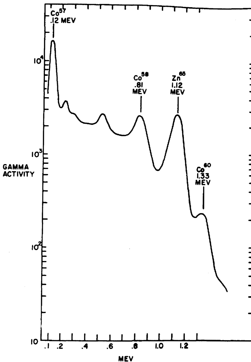
Fig. 13 Gamma spectrum curve on fish liver homogenate collected on How Island, Bikini Atoll, September 22, 1956.
