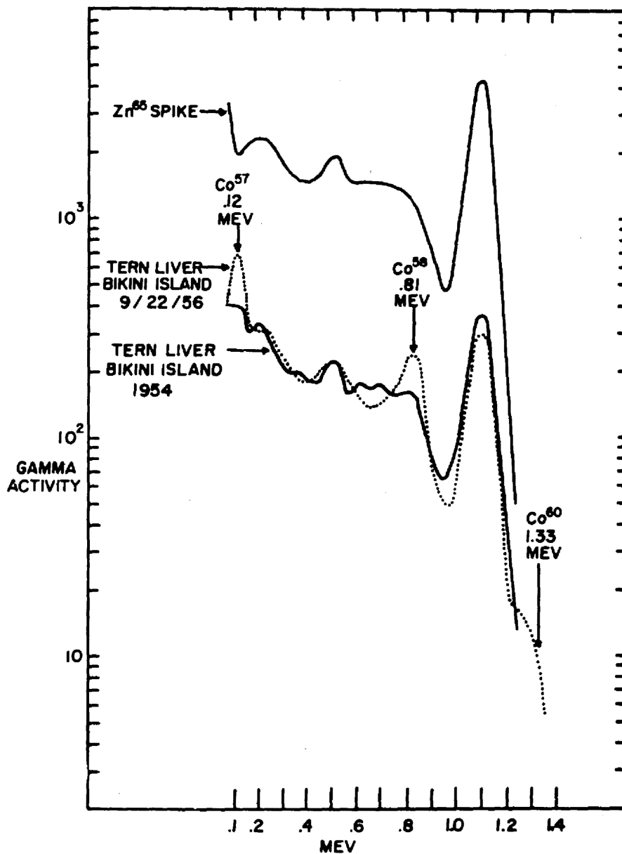
Fig. 15 Gamma spectra for tern livers collected at Bikini Atoll in 1954, and September 22, 1956. A gamma curve for a Zn 65 spike is shown for comparison.
