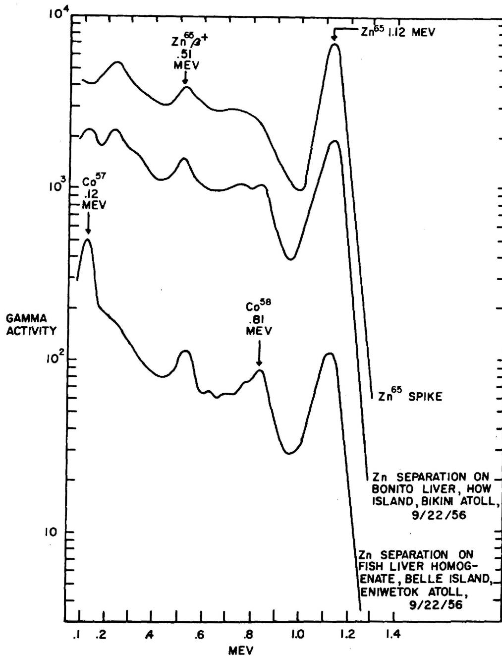
Fig. 9 Gamma spectrum curves from zinc chemical separations on fish livers collected at How Island, Bikini Atoll, and Belle Island, Eniwetok Atoll, on September 22, 1956. A gamma spectrum curve on a Zn 65 spike is shown for comparison.
