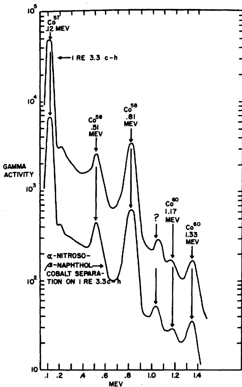
Fig. 4 Gamma spectrum curves of the pH 3.3 c-h ammonium citrate fraction from clam kidney sample I eluted on Dowex 50 and of an α-nitroso-β-naphthol cobalt separation done on the pH 3.3 c-h fraction.
