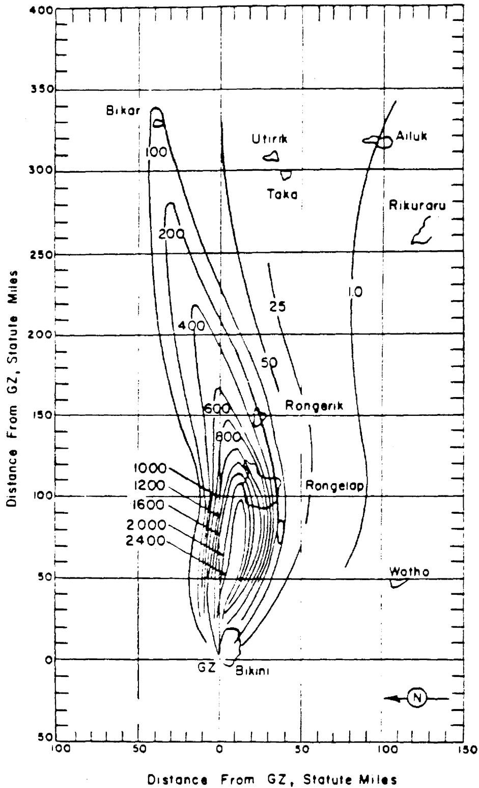
Operation CASTLE - Shot 1 - Bravo. Off-site dose rate contours in r/hr at H+1 hour (AFSWF).
