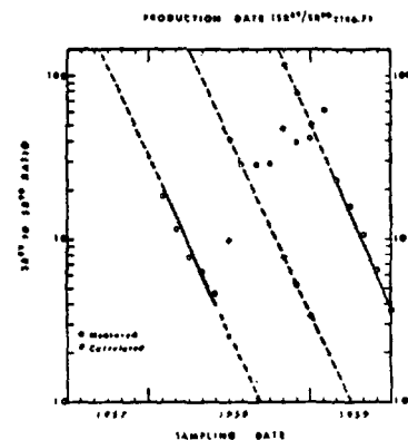
Fig. 1. Fallout from non-Hardtack sources in New York City during 1958 and 1959; Sr 90 /Sr 89 ratios, corrected for calculated Hardtack concentrations, are used. Most of the 1958 data are taken from the report of Welford and Collins (9). Strontium-89 values for the first three months of 1958 are taken from the data summaries of Hurdy et al. (12).
