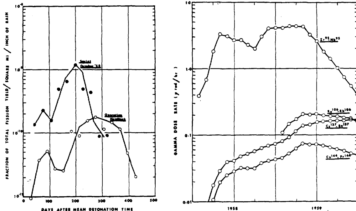
Fig. 2 (left). Comparison of the arrival patterns in New York City of debris from polar (Soviet) and from equatorial (Hardtack) test series conducted during 1958. Fig. 3 (right). Calculated infinite-plane dose rates from cumulative levels of gamma activities measured in fallout in New York City during 1958 and 1959.
