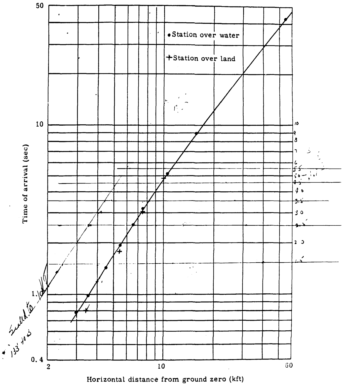
Fig. 21 — Time of arrival vs horizontal distance from ground zero (King shot).
