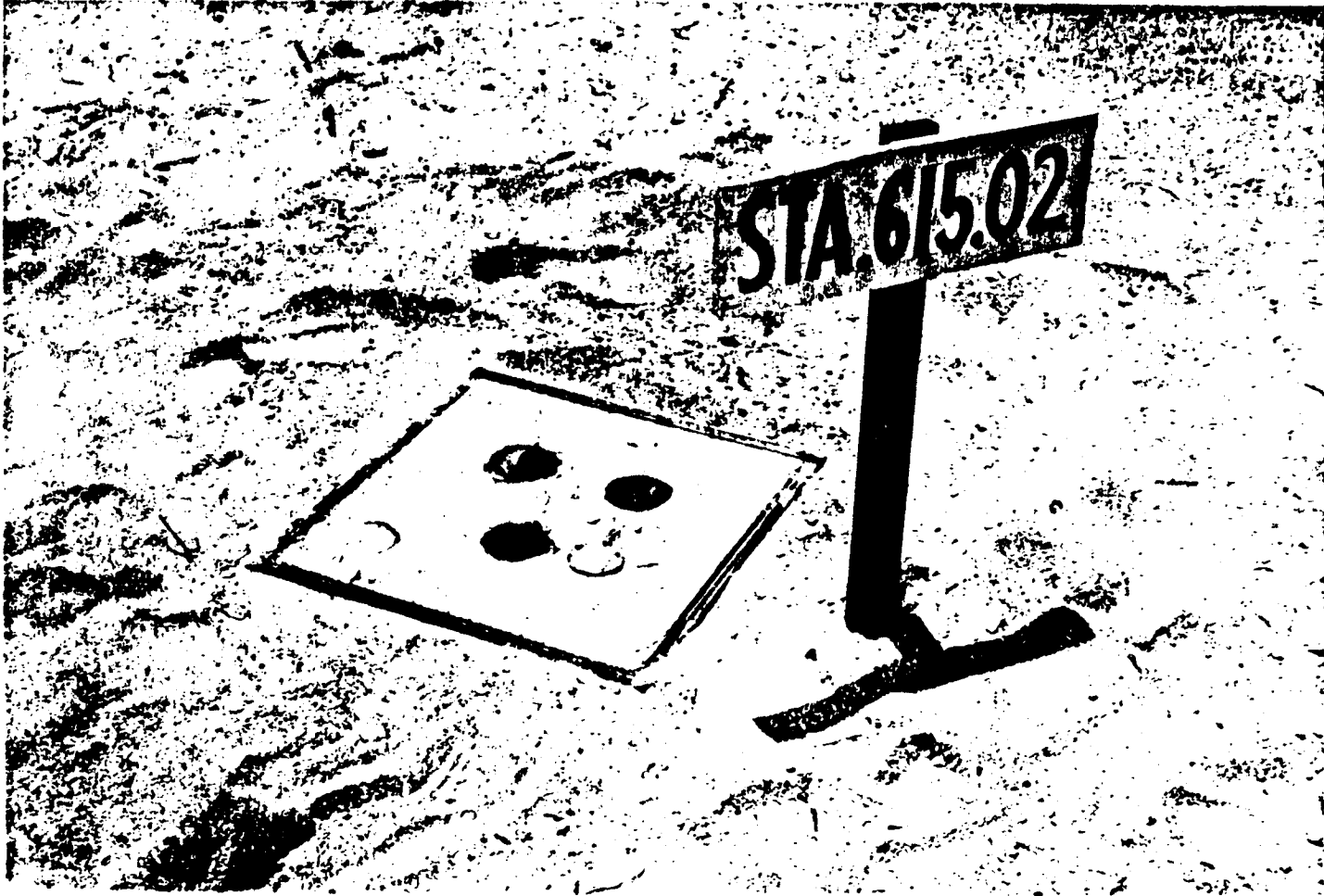
Fig. 2 — Wianeko gauges in ground baffle.
