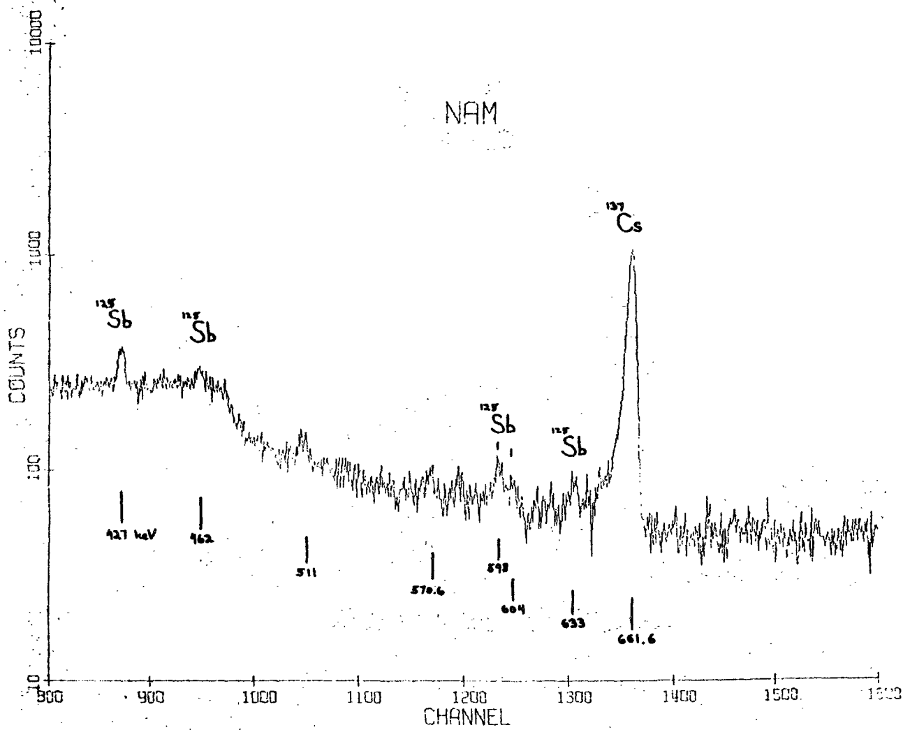
Figure 12b. Ge(Li) spectrum of soil sample taken from Nam Island.
