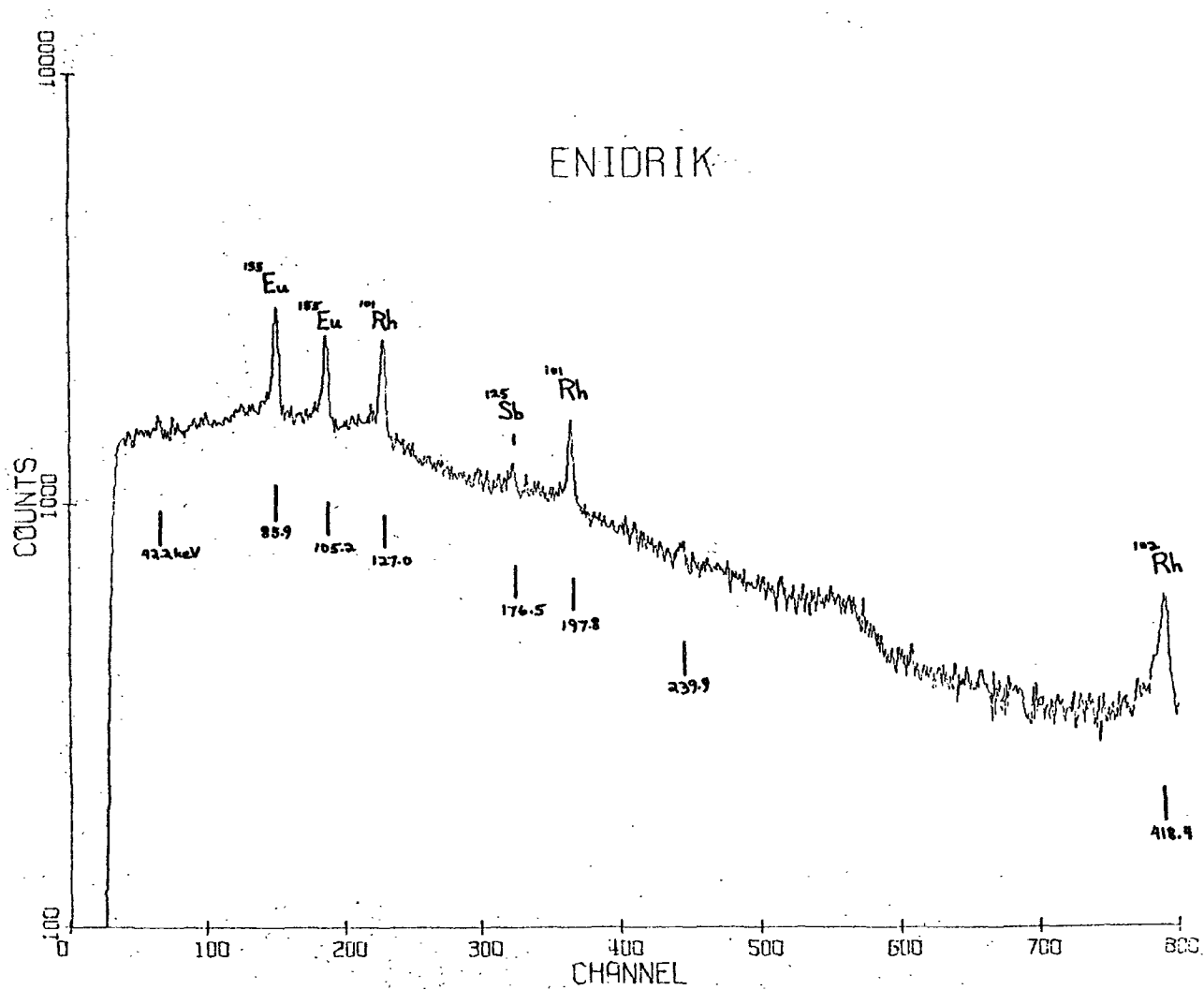
Figure 9a. Ge(Li) spectrum of soil sample taken from Enidrik Island.
