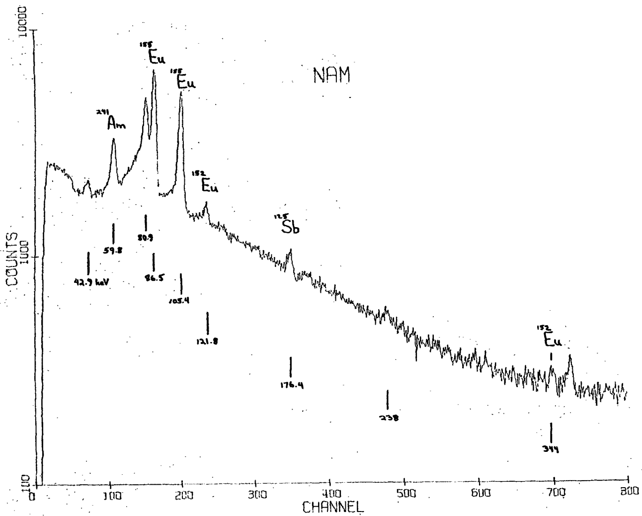
Figure 12a. Ge(Li) spectrum of soil sample taken from Nam Island.
