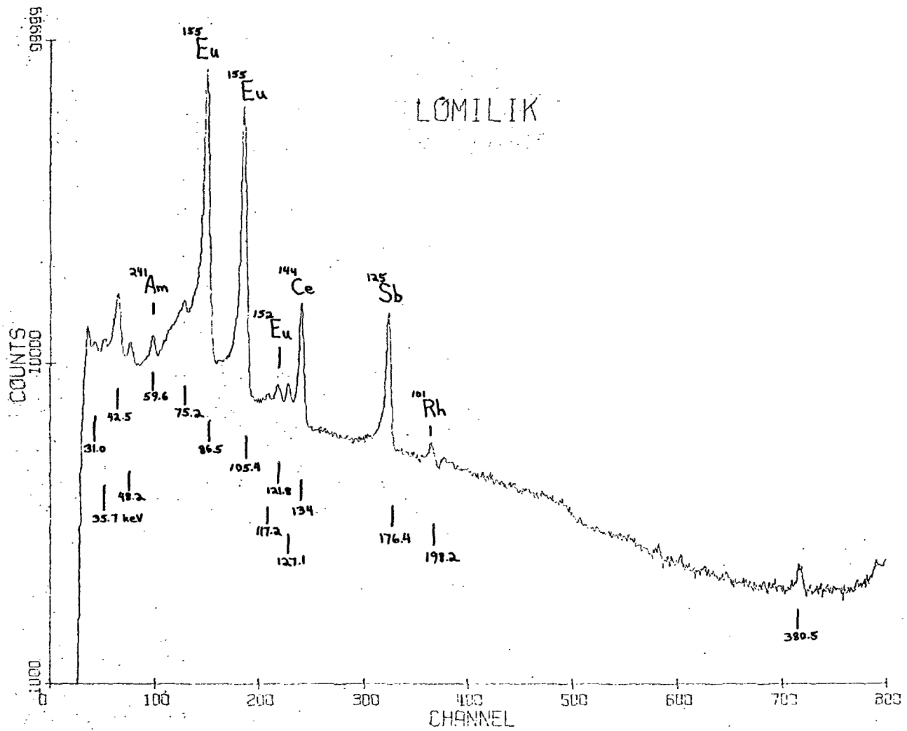
Figure 11a. Ge(Li) spectrum of soil sample taken from Lomilik Island, Aomen-Iroi Complex.
