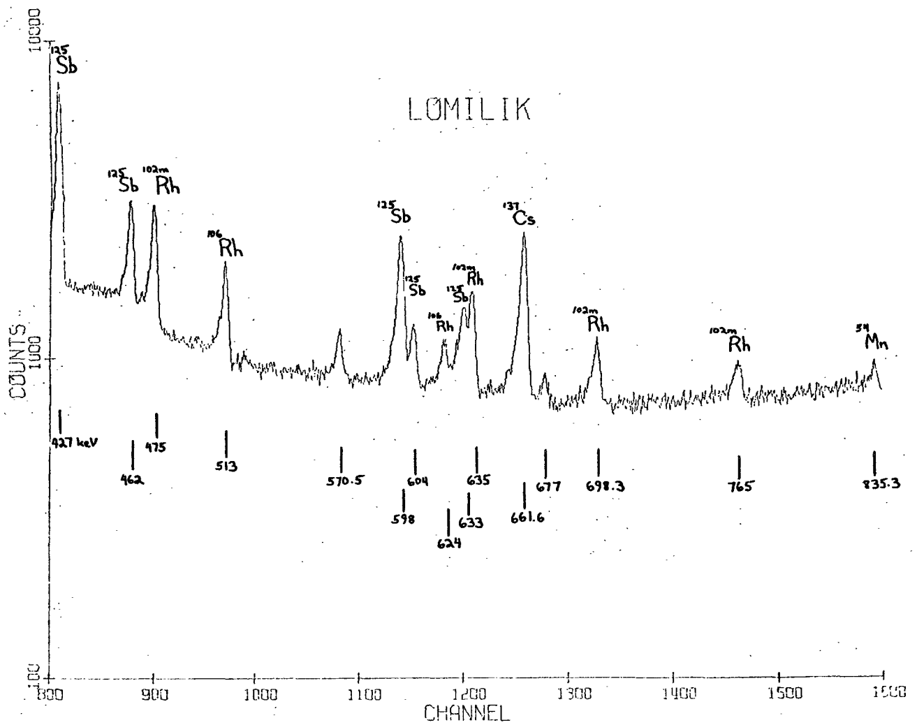
Figure 11b. Ge(Li) spectrum of soil sample taken from Lomilik Island, Aomen-Iroi Complex.
