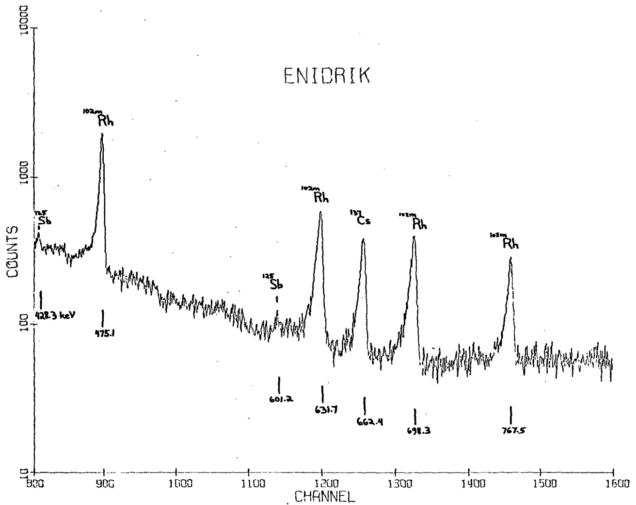
Figure 5b. Ge(Li) spectrum of soil sample taken from Enidrik Island.
