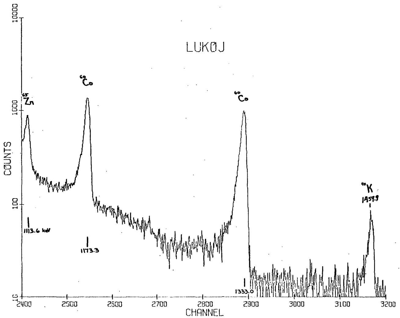
Figure 10d. Ge(Li) spectrum of soil sample taken from LukøJ Island.
