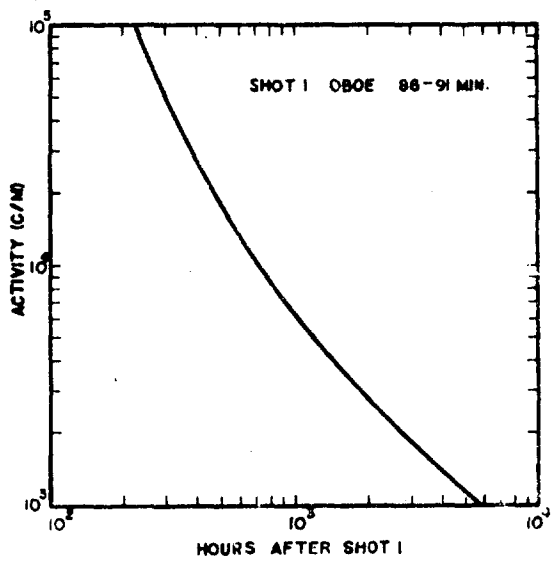
Fig. 3.2 Shots 1 and 3 Representative Decay Curves
