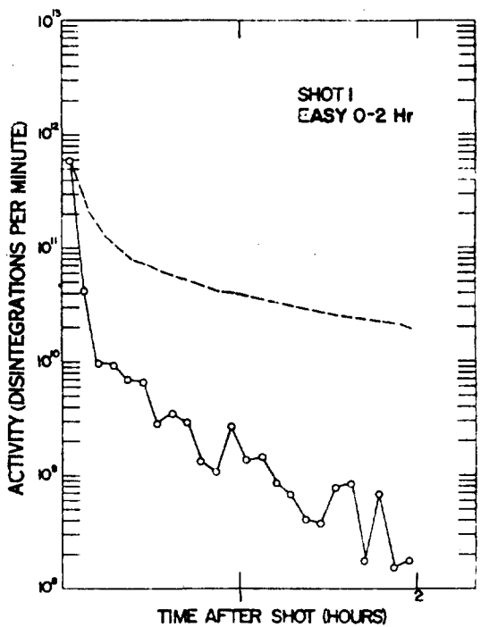
Fig. 3.5 Variation of Beta Activity with Time, Shot 1, Dog 1-24 min, Dog 0-12 hr, Easy 0-2 hr, Easy 0-12 hr.
