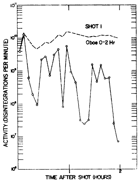
Fig. 3.7 Variation of Beta Activity with Time, Shot 1, Nan 0-2 hr, Nan 0-12 hr, Oboe 0-2 hr, Oboe 0-12 hr.
