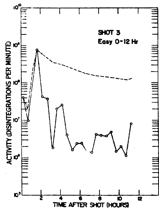
Fig. 3.12 Variation of Beta Activity with Time, Shot 3, Dog 0-12 hr, Easy 0-2 hr; Easy 0-12 hr, Fox 0-2 hr.
