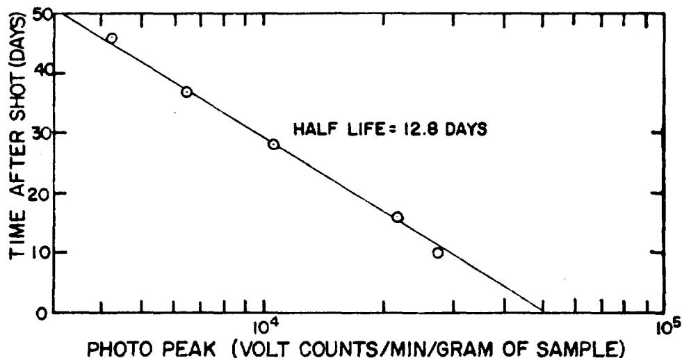
Fig. 3.28 The \text{La}^{140} 1.6 Mev Photopeak as a Function of Time
