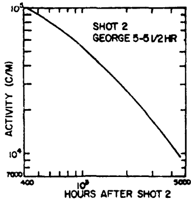
Fig. 3.3 Example of Shot 2 Decay Curve Plotted to Shots 2 and 1 Zero Times
