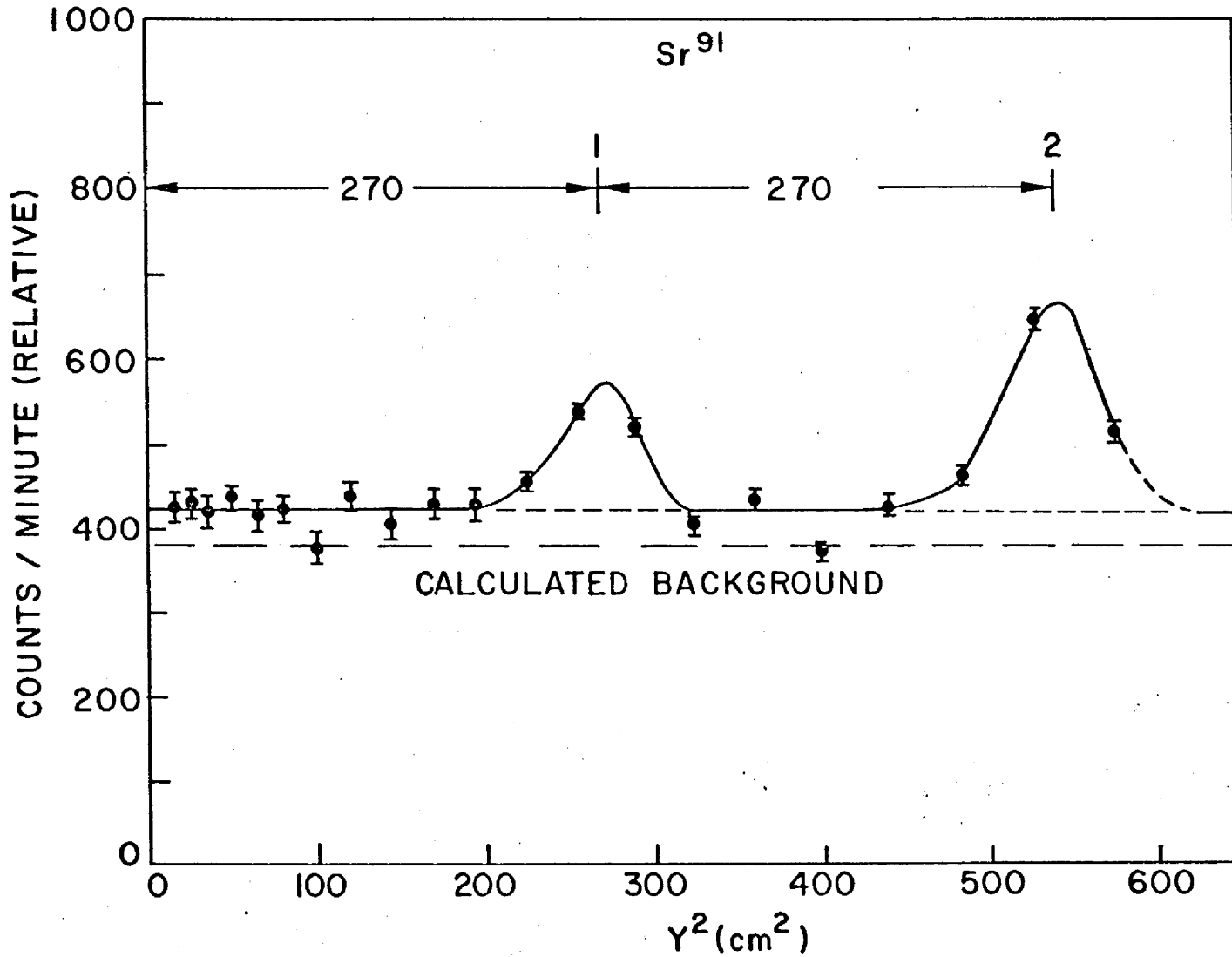
Fig. 9 - UCRL-6491 Rev. II Author s: P. C. Stevenson and H. C. Hicks PK
