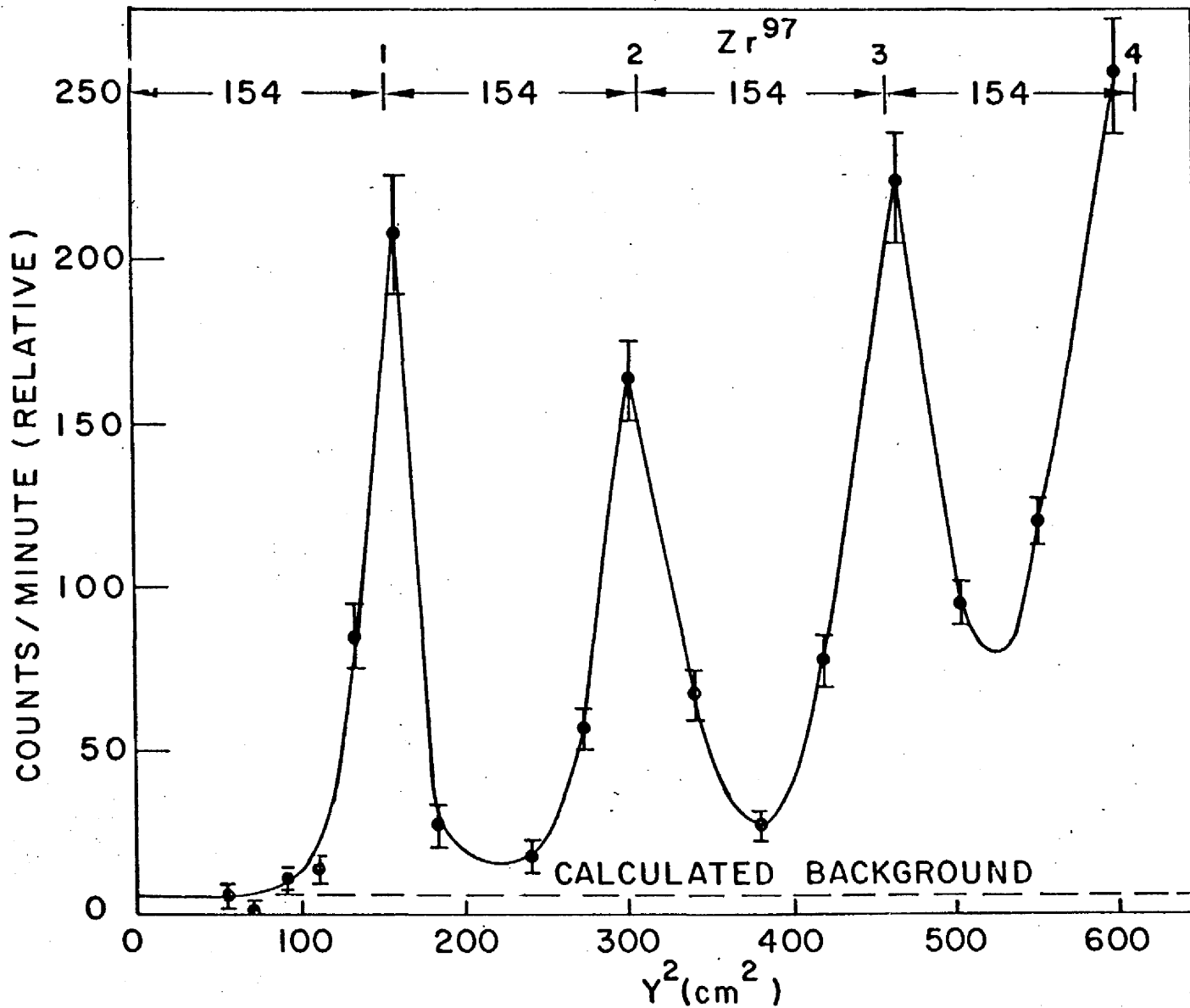
Fig. 10 - UCRL-6491 Rev. II Authors: P.C. Stevenson and H.C. Hicks
