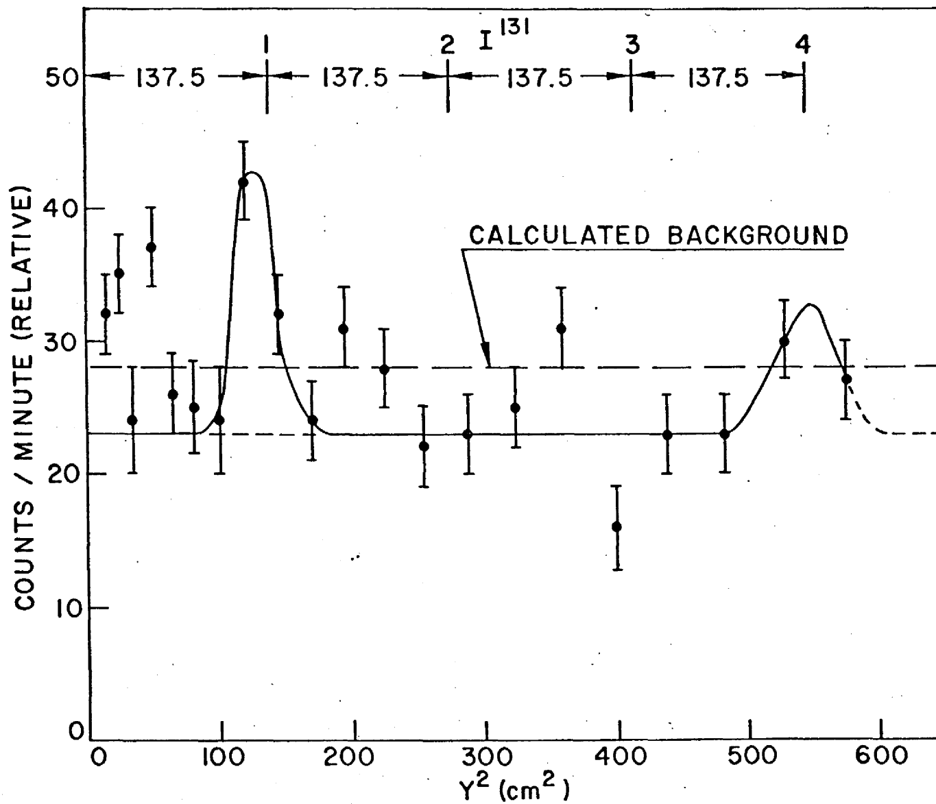
Fig. 12 - UCRL-6491 Rev. II Authors: P.C. Stevenson and H.C. Hicks
