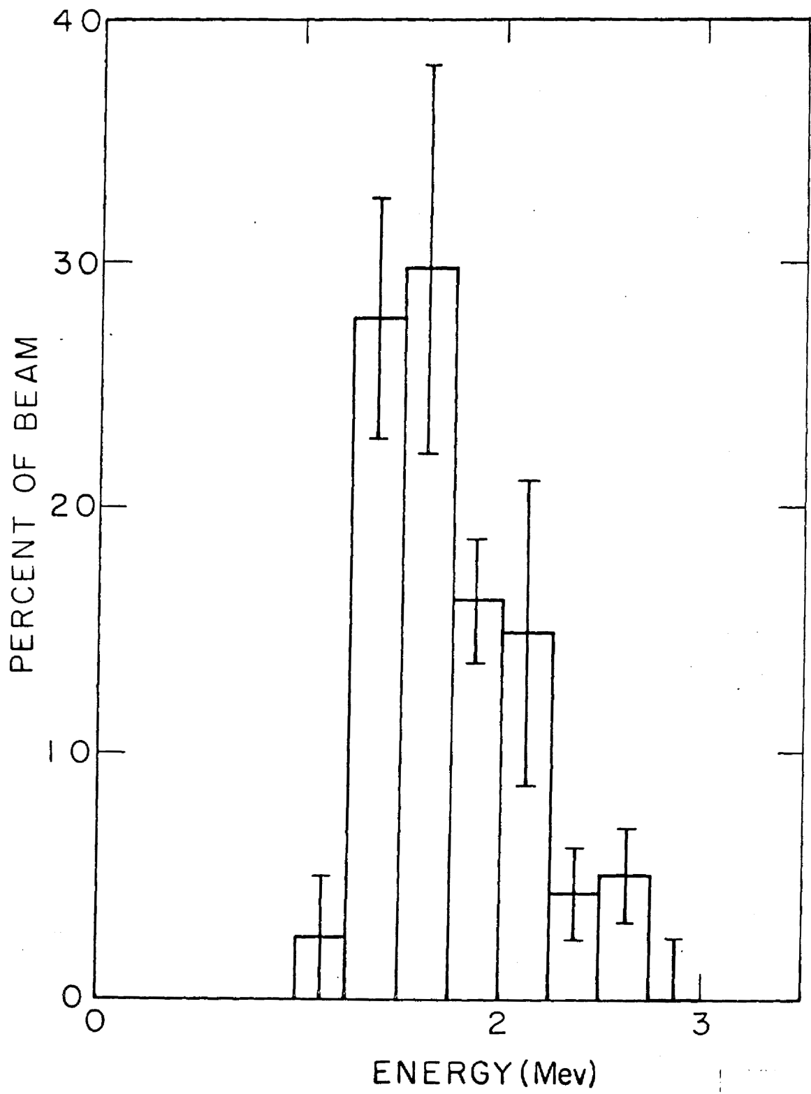
Fig. 16 - UCRL-6491-Rev. II Authors: P.C. Stevenson and H.C. Hicks
