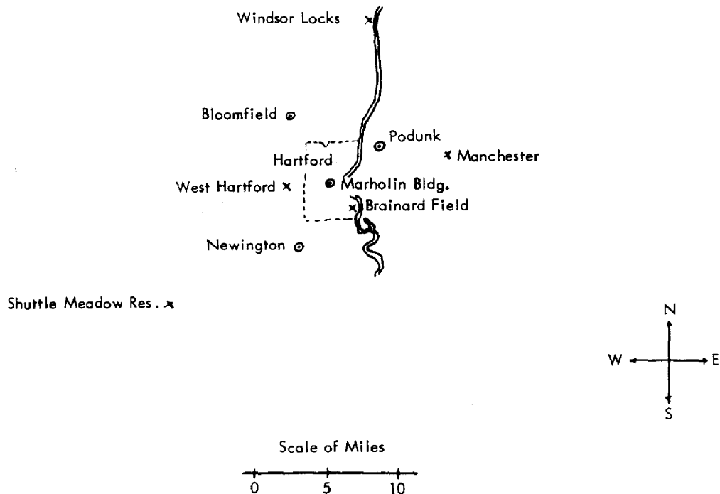
Fig. 14—Pot fallout collections in the Hartford area. \odot , pot fallout collecting stations; \times , rain measurement stations.
