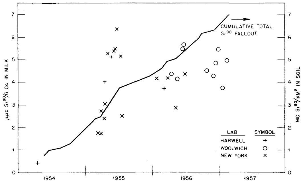
Fig. 6—Sr 90 in Somerset milk.
