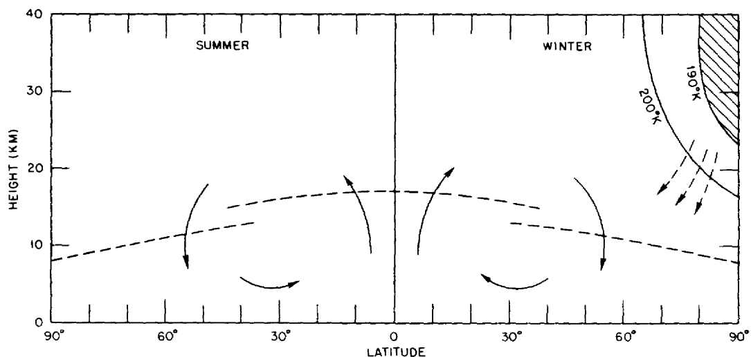
Fig. 7— Atmospheric circulation model (after Dobson and Brewer).
