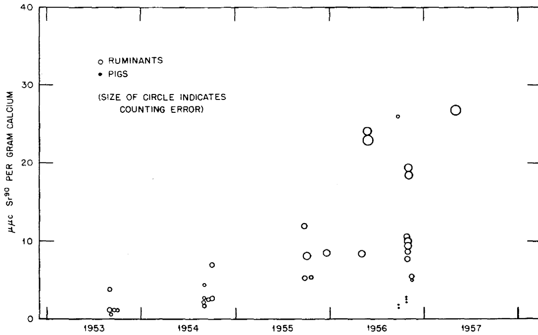
Fig. 1—Strontium-90 in animal bone.
