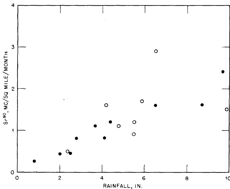
Fig. 2a— Regression of Sr^{90} in rain water on the amount of rainfall in March 1956.
