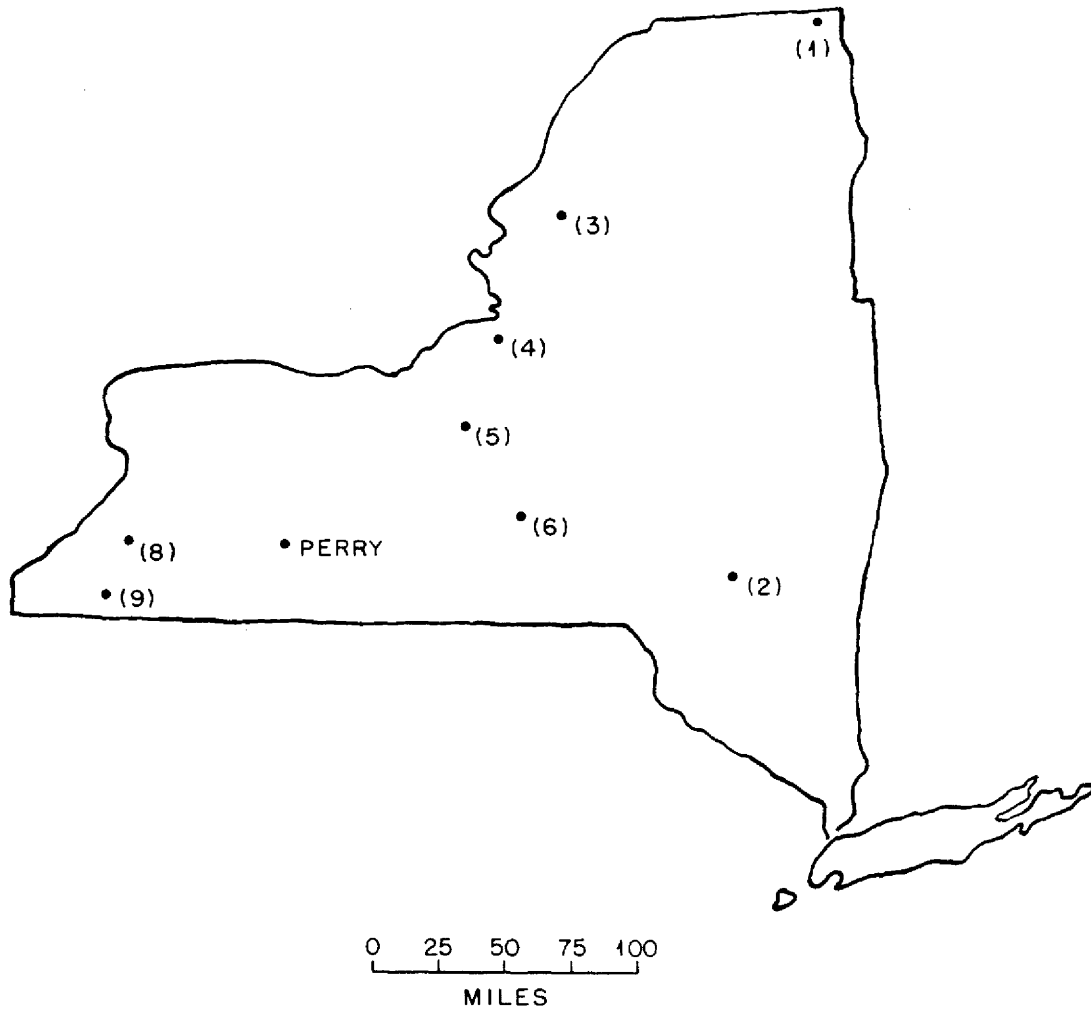
Fig. 15—New York State Department of Health milk powdering plant survey. (1), Champlain Milk Products, Champlain; (2) Andes Co-op Creamery, Andes; (3), Borens, Evans Mills; (4), Ontario Milk Producers Co-op, Mexico; (5) Cooperdale Dairy, Inc., Skaneateles; (6) Borens Farm Products, Cincinnatus; (7). Arkport Dairies, Arkport; (8), Collins Center Cooperative, Collins Center; (9). Queensboro Milk Products Co., Steamburg.
