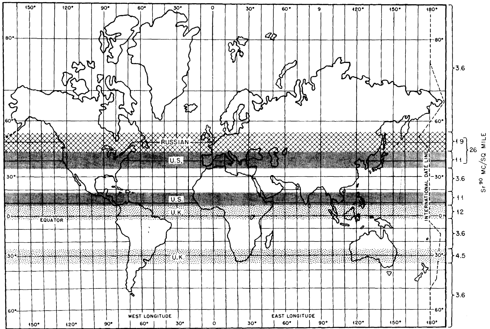
Fig. 4—World fallout map (at end of 1957).
