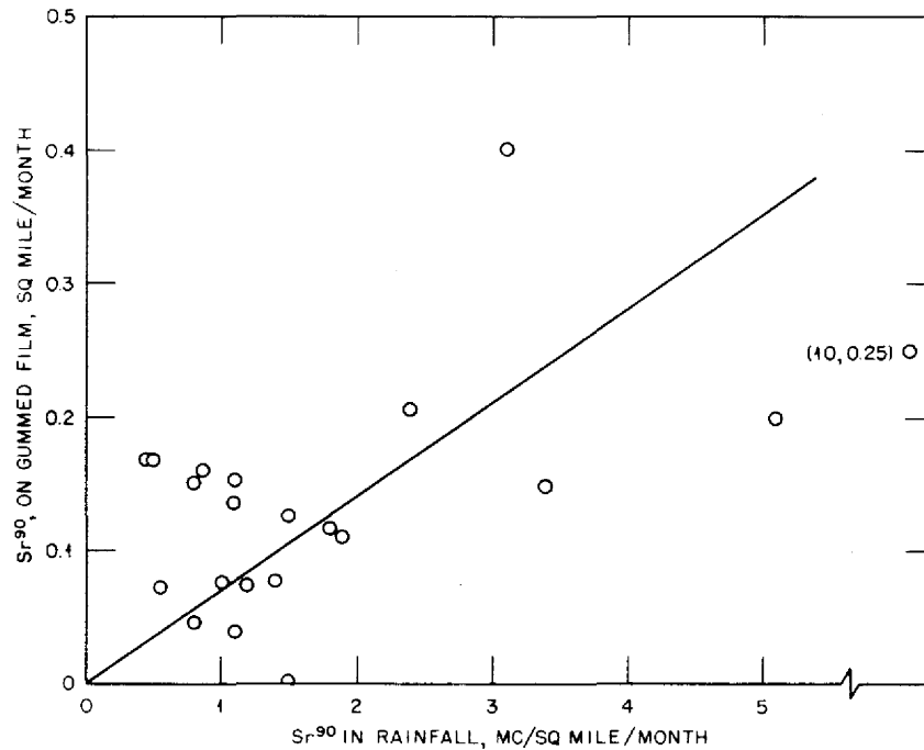
Fig. 5—Regression of \text{Sr}^{90} in gummmed film on \text{Sr}^{90} in rain water from 20 stations in May 1956.
