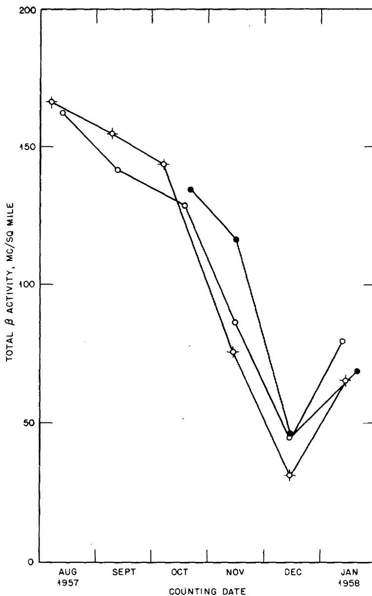
Fig. 2—Comparison of total \beta activity from three collection units. ◇, roof pot; ●, roof funnel; ○, roof funnel and resin.
