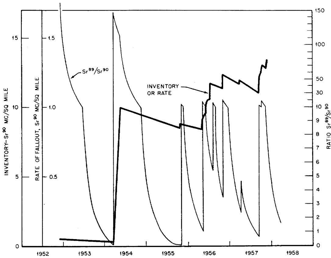
Fig. 9—Stratospheric inventory and rate of fallout; also Sr^{89}/Sr^{90} ratio.
