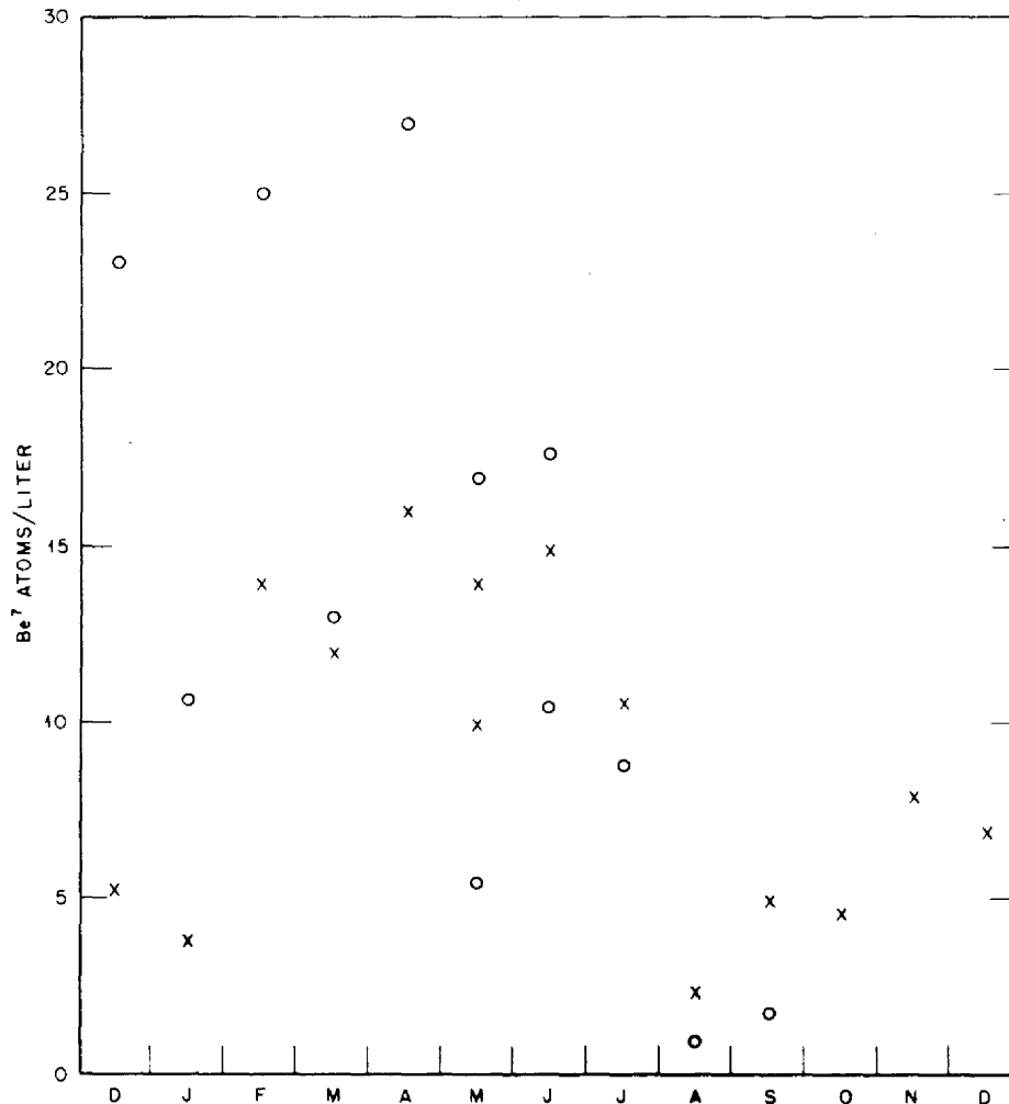
Fig. 6 — Beryllium measurements: O, Station 1; x, Station 2.
