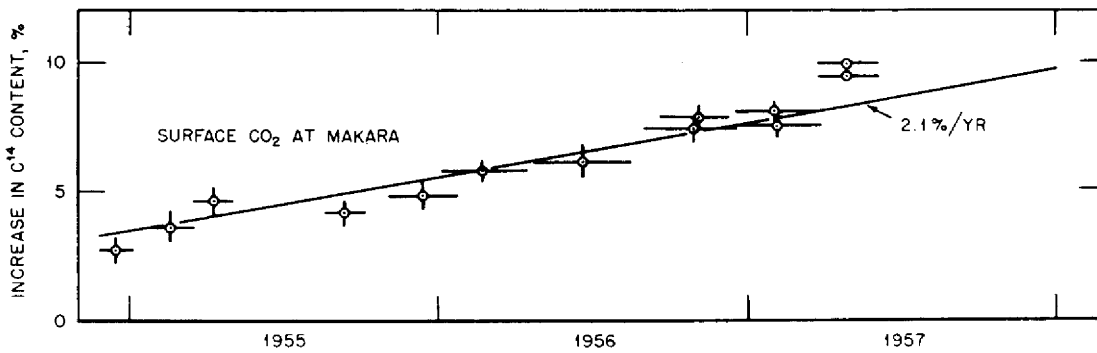
Fig. 10—Bomb C^{14} effect.
