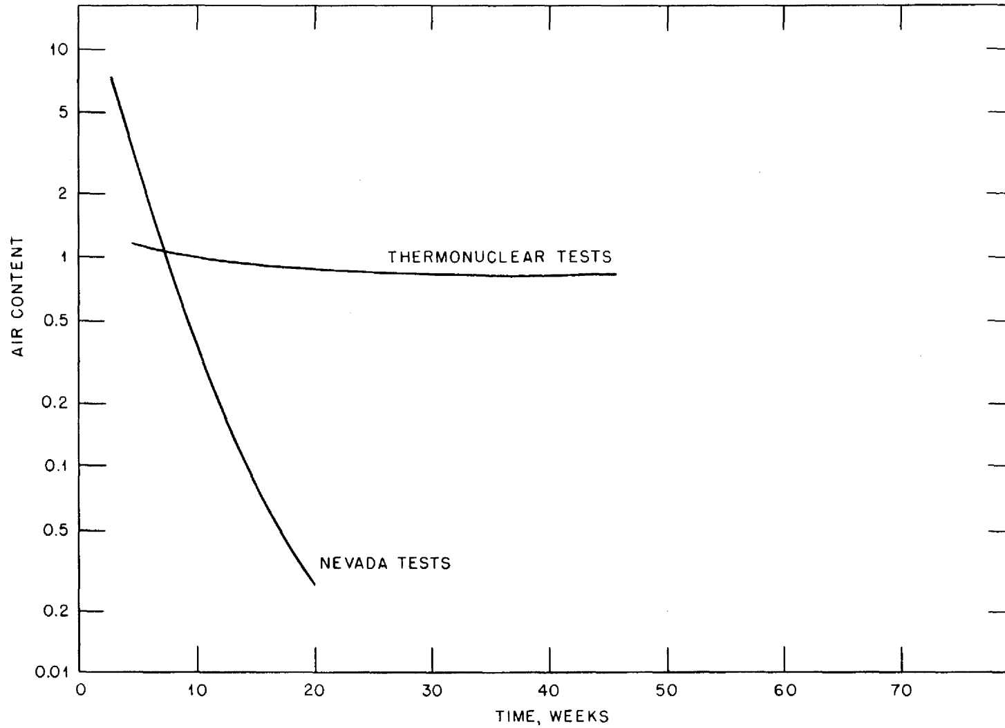
Fig. 2—Intermediate fallout from Nevada and thermonuclear tests.
