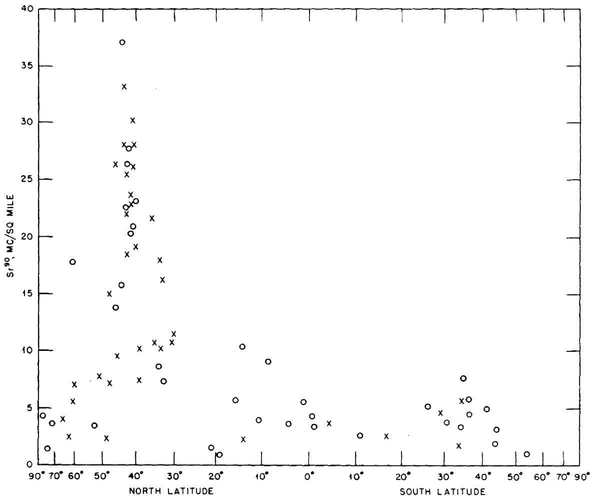
Fig. 9— Soil data, 1956: ○, electroanalysis × 1.15; x, HCl extraction.
