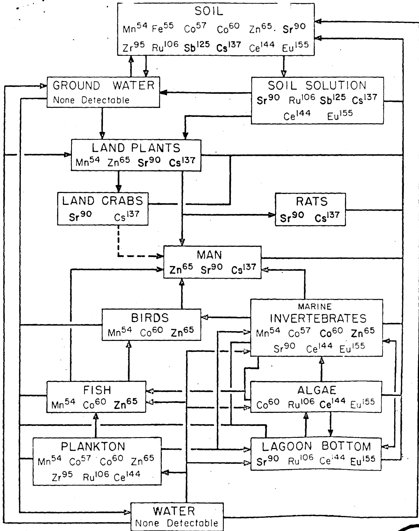
DISTRIBUTION OF FALLOUT RADIOISOTOPES 5005111 RONGELAP ATOLL. 1961
