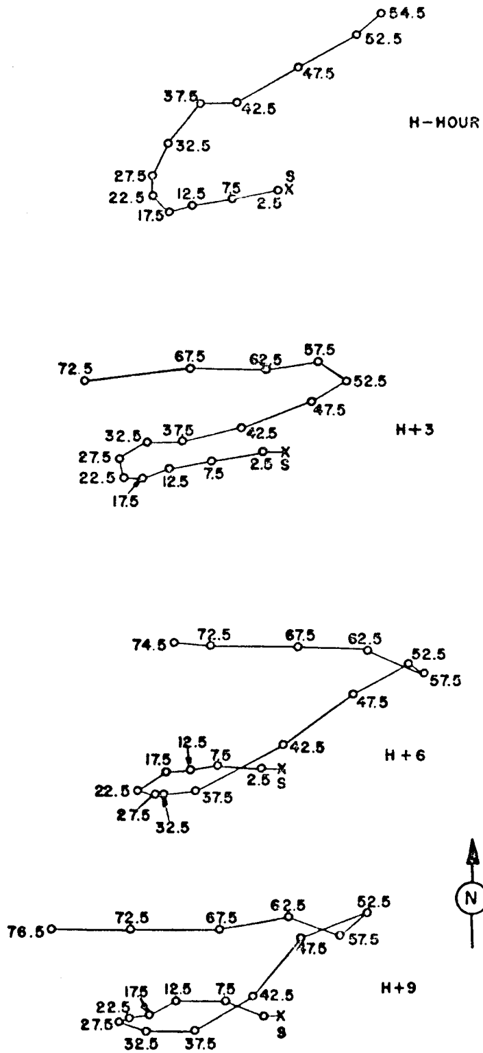
Figure 106. Hodographs for Operation REDWING -
