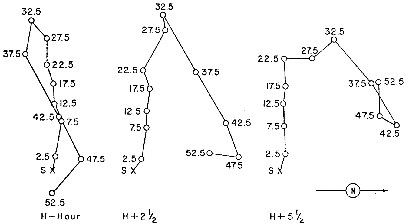
Figure 87. Hodographs for Operation REDWING - Blackfoot.
