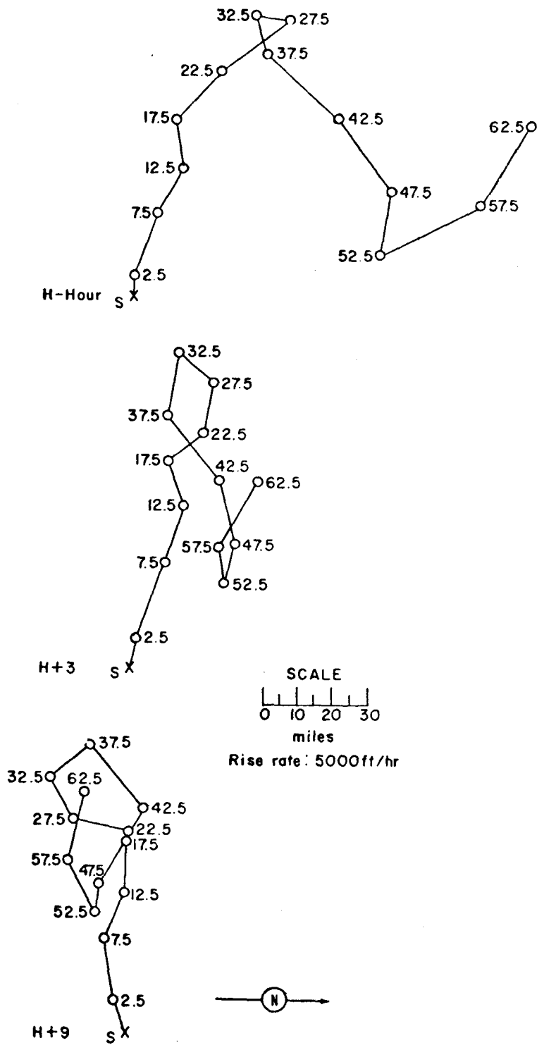
Figure 138. Hodographs for Operation HARDTACK I -
