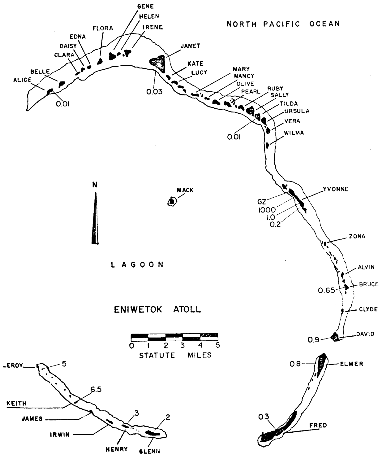
Figure 16. Operation GREENHOUSE - rates in r/hr at H+1 hour.
