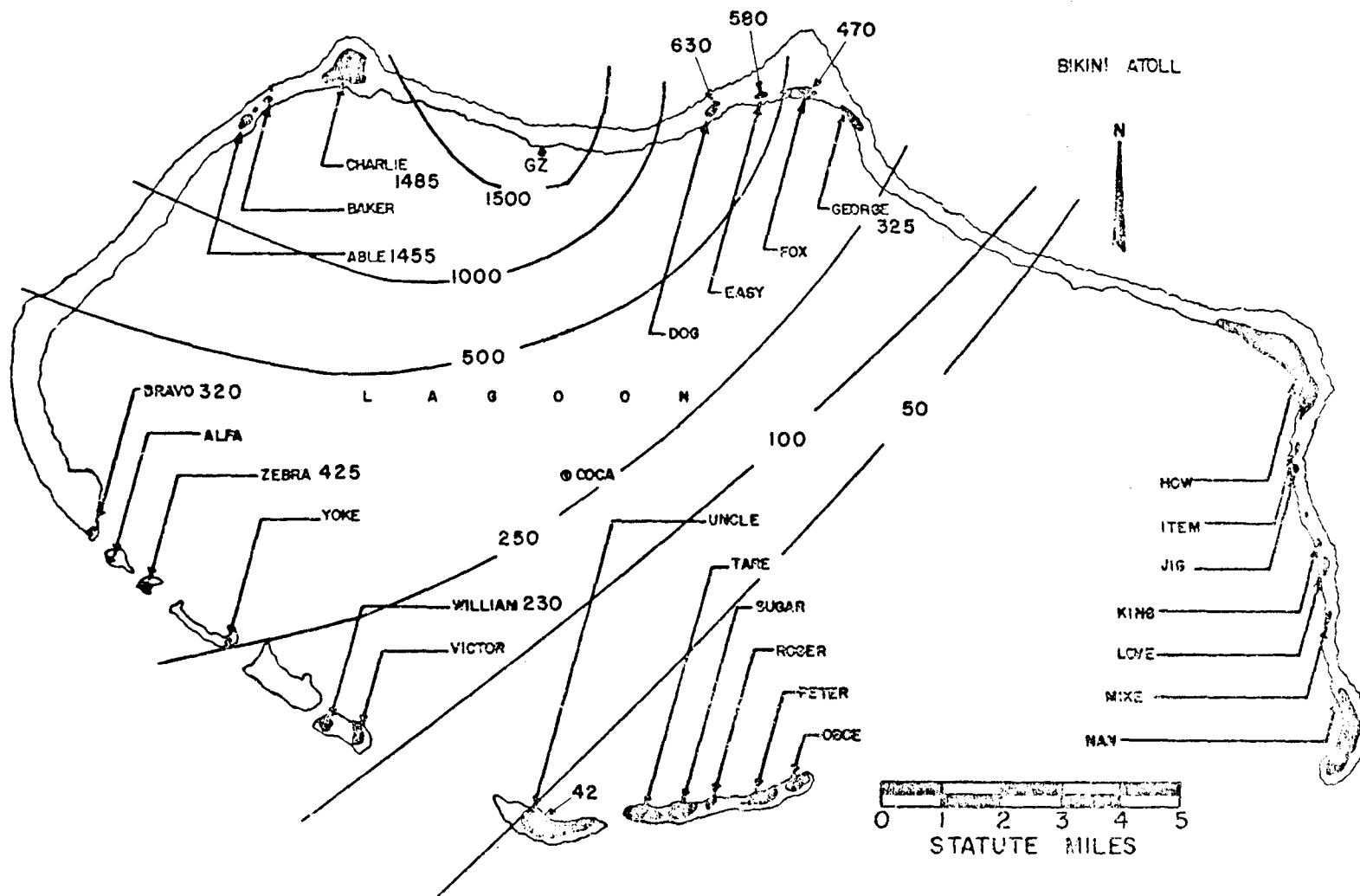
Figure 107. Operation REDWING - Tewa. Atoll dose rate contours in r/hr at H+1 hour.
