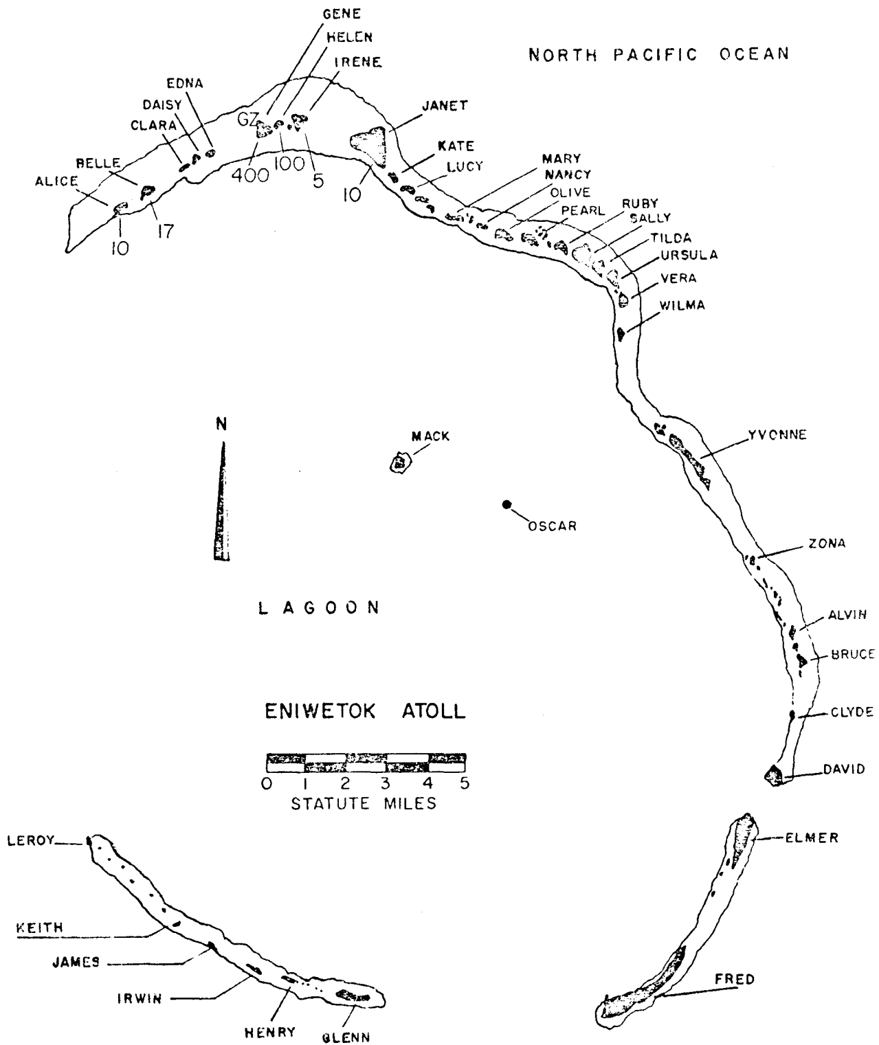
Figure 111. Operation REDWING - Huron. Island dose rates in r/hr at H+1 hour.
