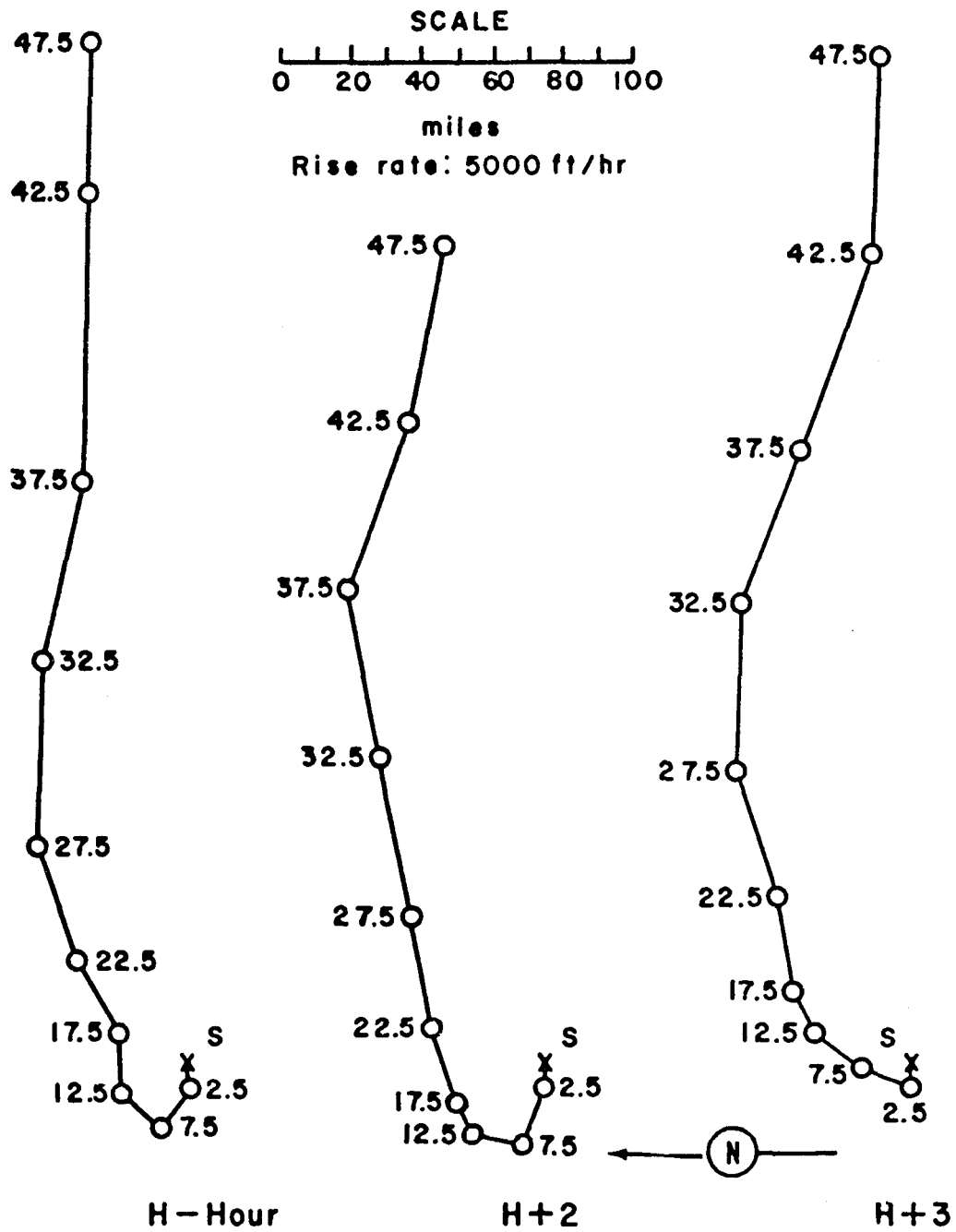
Figure 13. Hodographs for Operation SANDSTONE - Zebra
