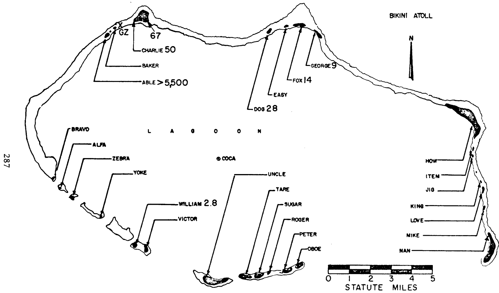
Figure 165. Operation HARDTACK I - Poplar. Island dose rates in r/hr at H+1 hour.
