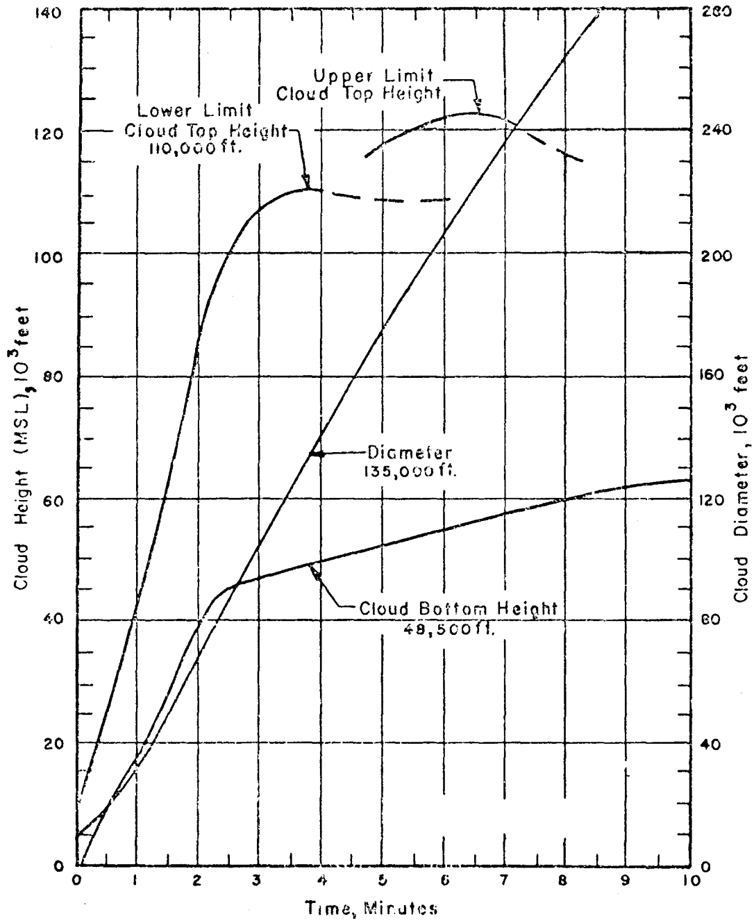
Figure 46. Cloud Dimensions: Operation CASTLE - Romeo.
