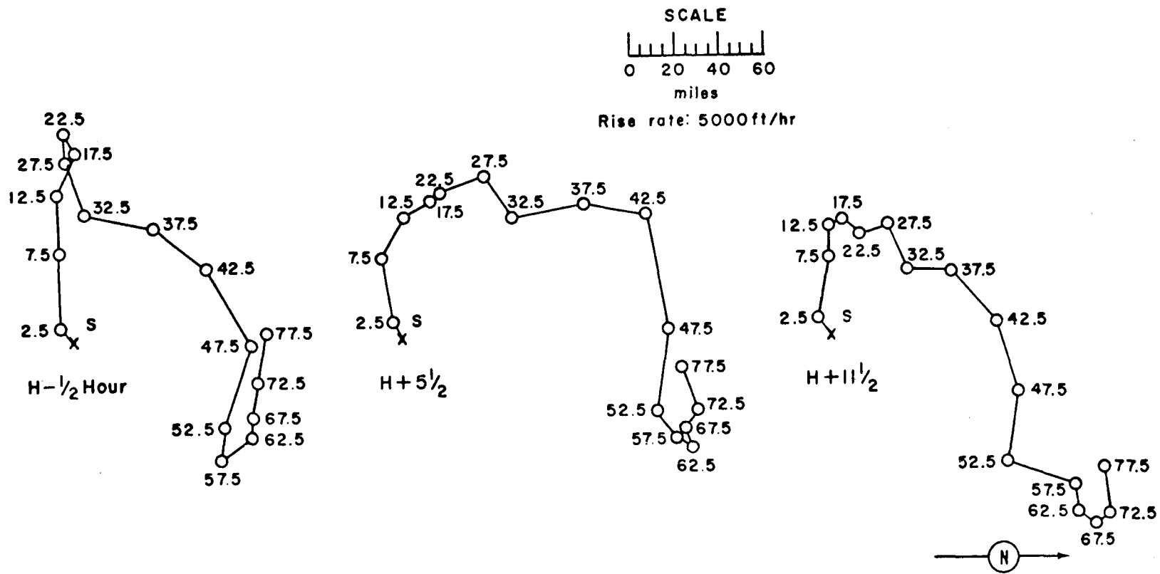
Figure 124. Hodographs for Operation HARDTACK I - Koa.
