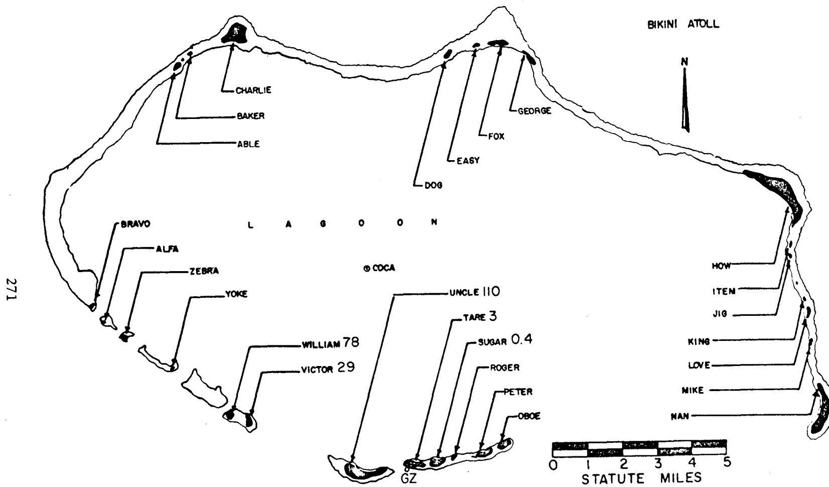
Figure 157. Operation HARDTACK I - Hickory. Island dose rates in r/hr at H+1 hour.
