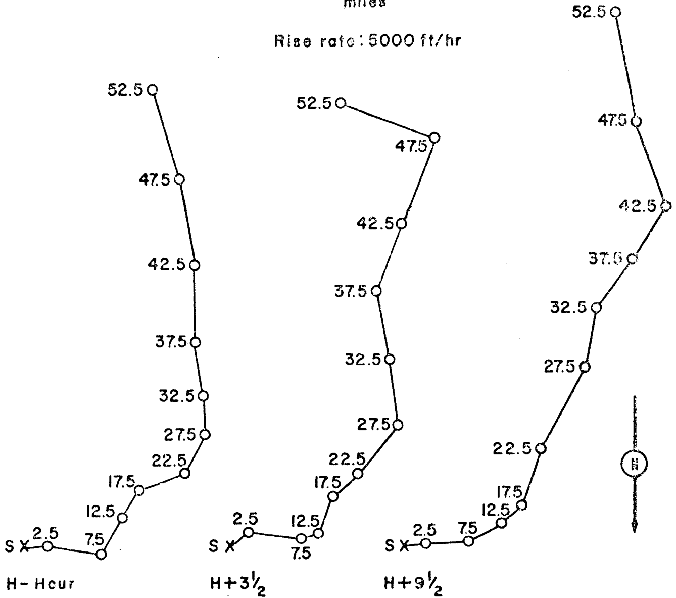
Figure 89. Hodographs for Operation REDWING - Kickapoo
