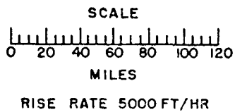
Figure 110. Hodographs for Operation REDWING - Tewa.
