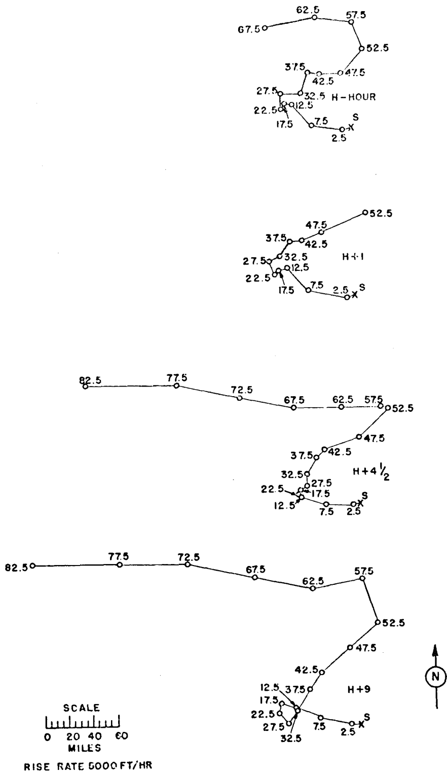
Figure 102. Hodographs for Operation REDWING -
