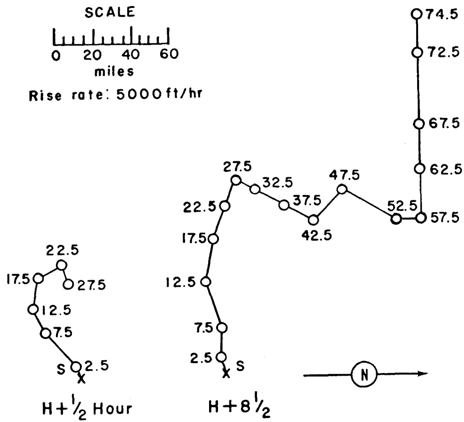
Figure 166. Hodographs for Operation HARDTACK I -
