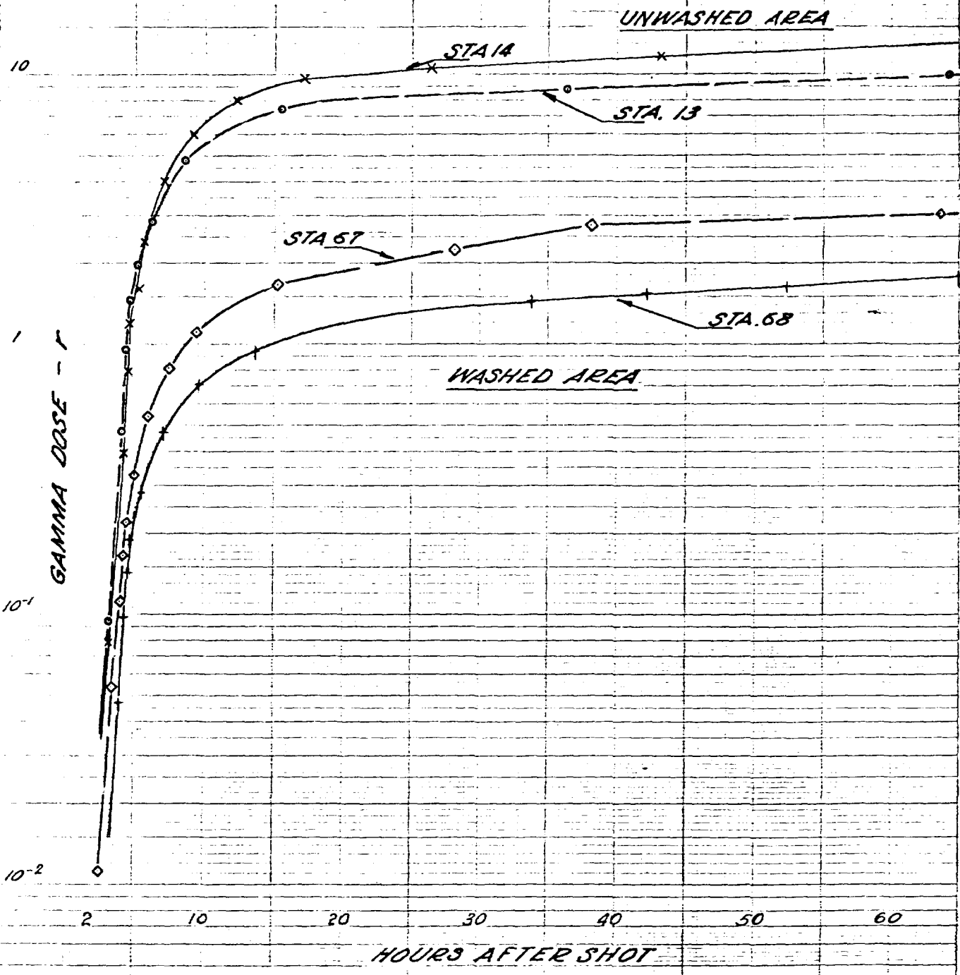
GAMMA DOSE ON DECK OF YAG 39
