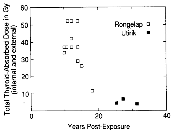
Fig. 6: Relation of thyroid-absorbed dose to time of development of surgically confirmed nodules in persons who were between 1 and 6 years of age at the time of exposure on Rongelap and Utirik.
