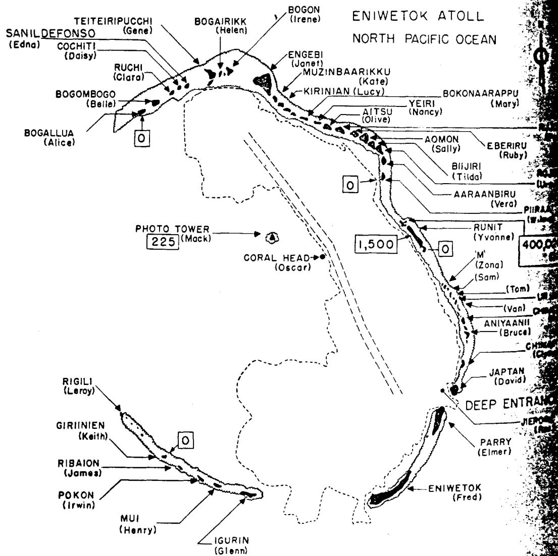
Fig. 2.1—Cactus radiation intensities on Eniwetok Atoll at H+4 hr, in milliroentgens per hour. Shot island was Runit.
