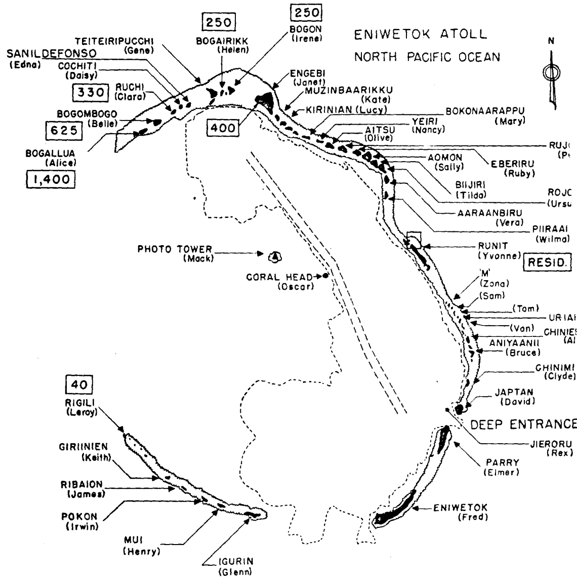
Fig. 2.11—Elder radiation intensities on Eniwetok Atoll at H+4 hr, in m. roentgens per hour. Shot was fired on a barge off Engebi.
