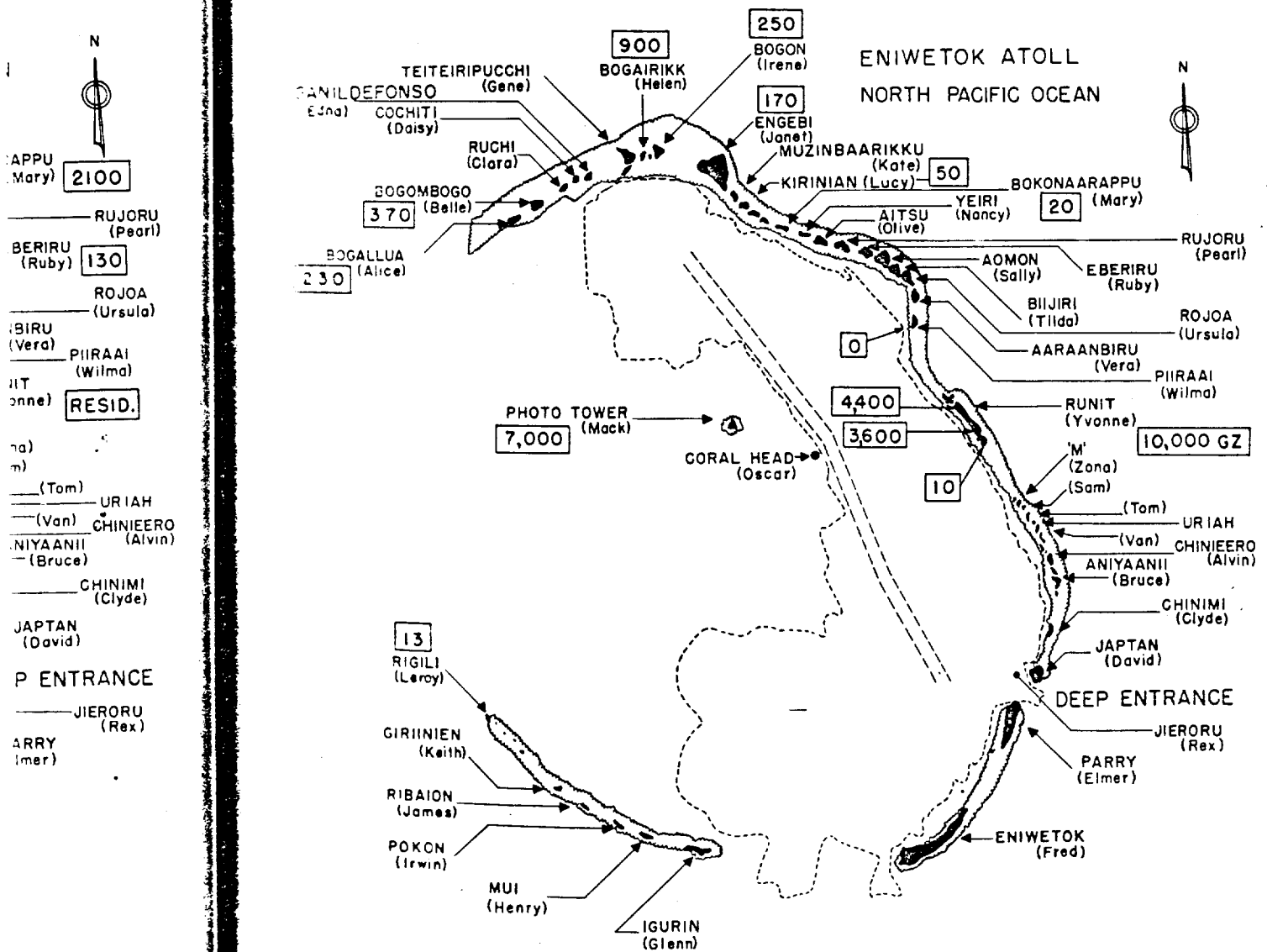
Fig. 2.4—Holly radiation intensities on Eniwetok Atoll at H+4 hr, in milli-roentgens per hour. Shot was fired on a barge off Runit.
