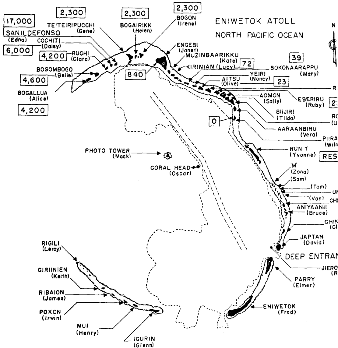
Fig. 2.9—Walnut radiation intensities on Eniwetok Atoll at H+4 hr, in m roentgens per hour. Shot was fired on a barge off Engebi.
