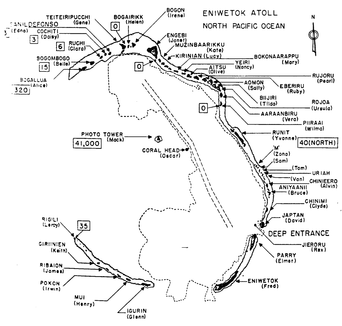
Fig. 2.2-Butternut radiation intensities on Eniwetok Atoll at H+4 hr, in milliroentgens per hour. Shot was fired on a barge off Runit.
