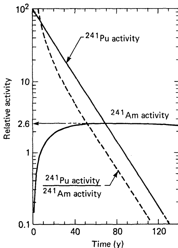
Figure 2. Relationship between parent ^{241}\text{Pu} activity and daughter ^{241}\text{Am} activity.
