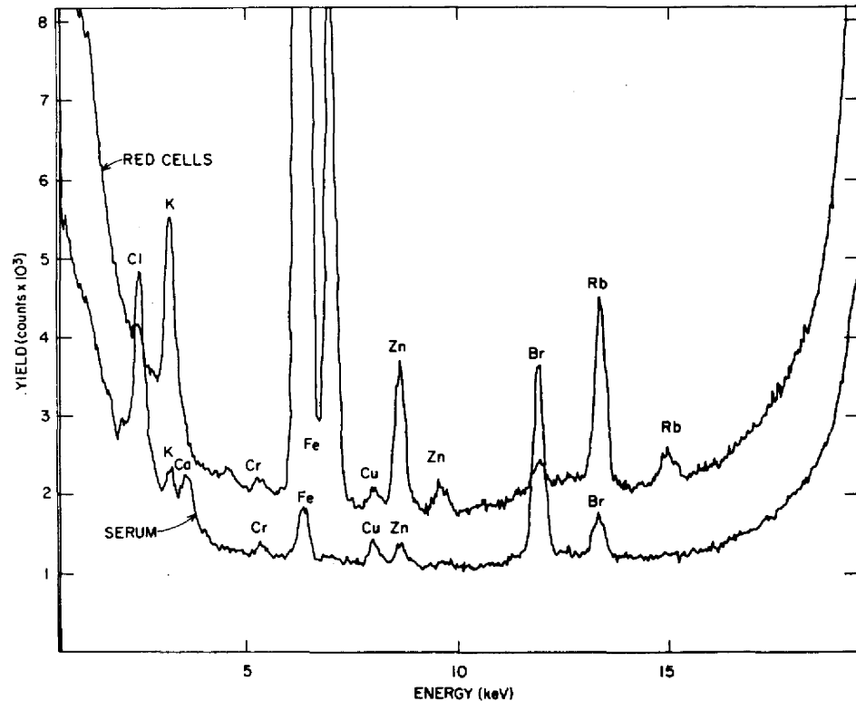
FIG. 1. Typical EDXRF spectrum of red cells and serum from a New York subject.
