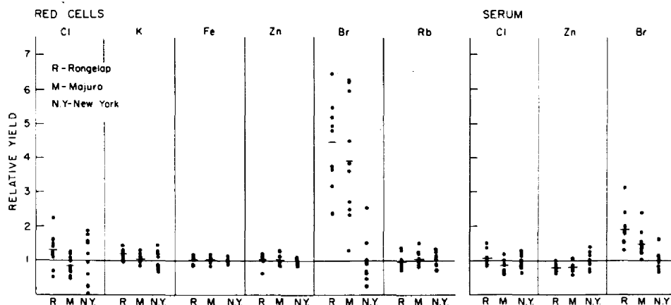
FIG. 2. Relative abundance of the elements present in the red cells and the serum normalized by the mean value of the New York group.
