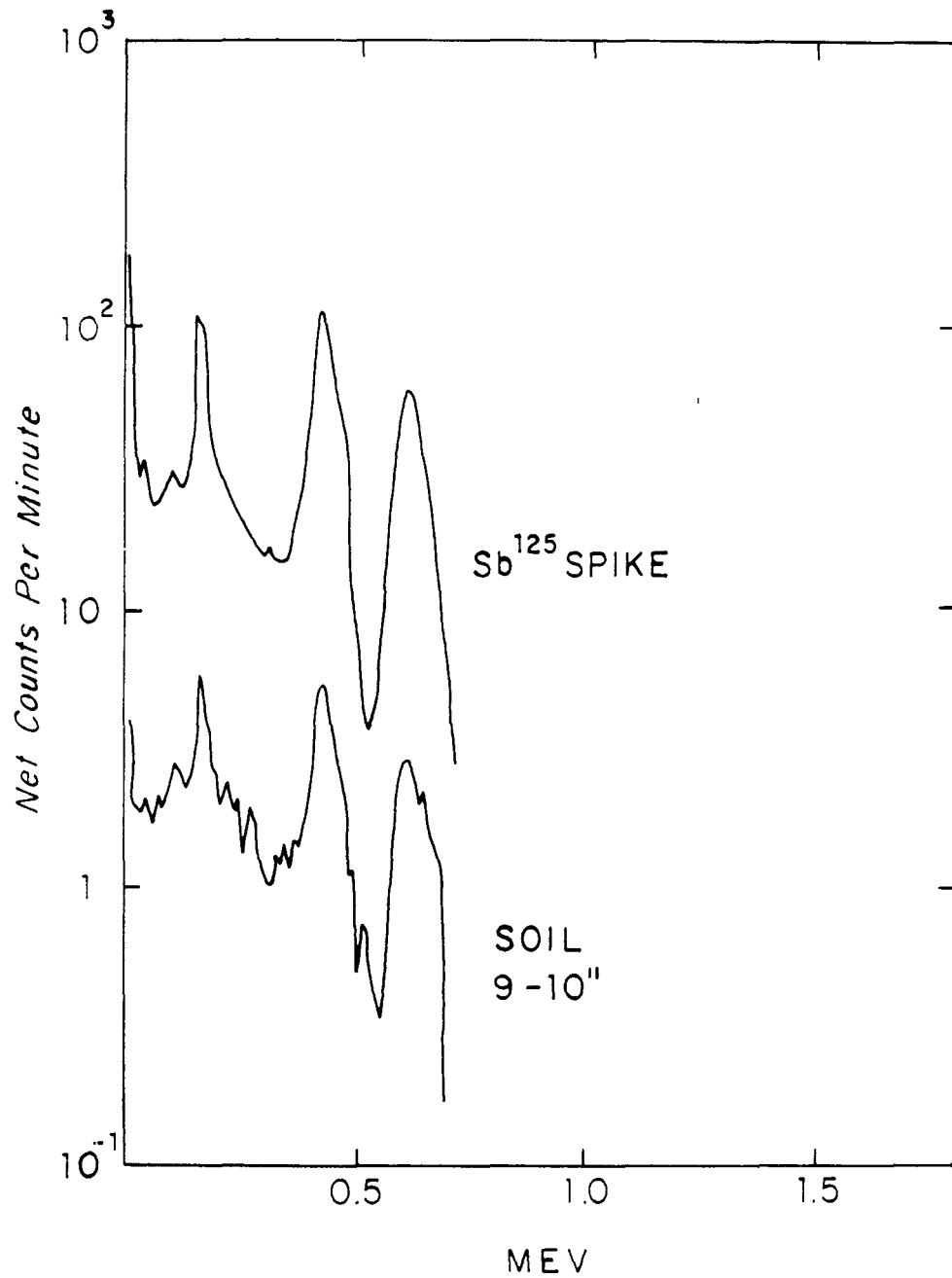
Fig. 10. Gamma-ray spectrum of young soil from a depth increment of 9 to 10 inches compared with the gamma spectrum of Sb^{125} .
