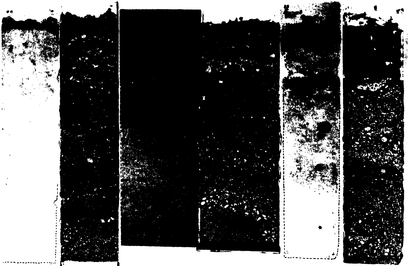
Fig. 12. Radioautographs and photographs of soil core sections. From left to right: undisturbed young soil, eroded young soil, old soil.
