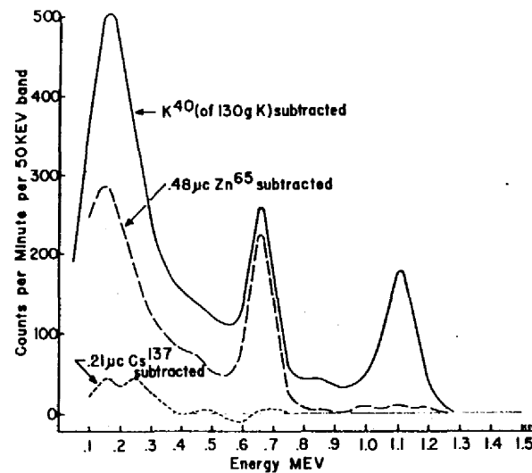
Fig. 21. Analysis of gamma-ray spectrum of Marshallese Subject No. 5
