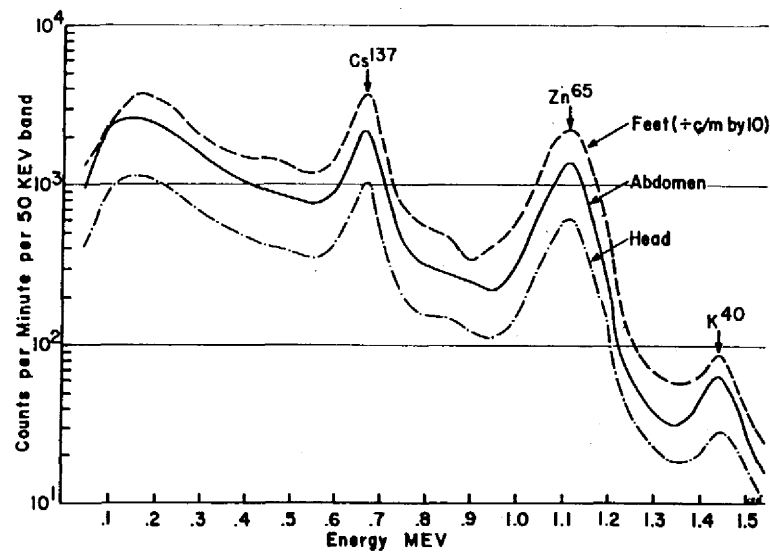
Fig. 23. Net gamma-ray spectra of Marshallese Subject No. 5
