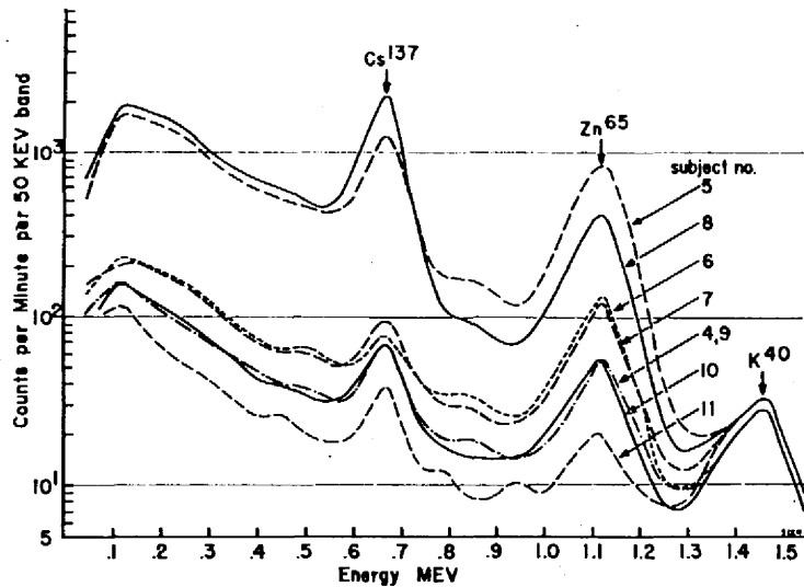
Fig. 20. Net in vivo gamma-ray spectra of Marshallese
