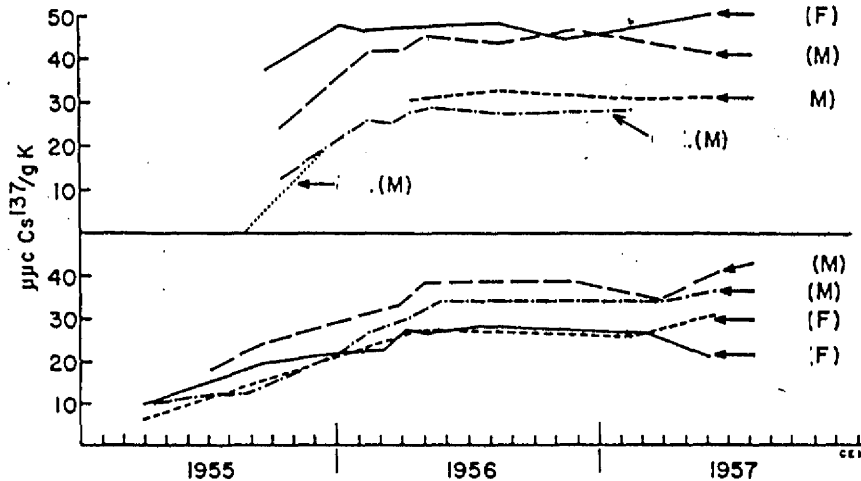
Fig. 18. Cs^{137} trends in humans
