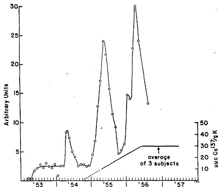
Fig. 19. Cs^{137} activity in filter papers
