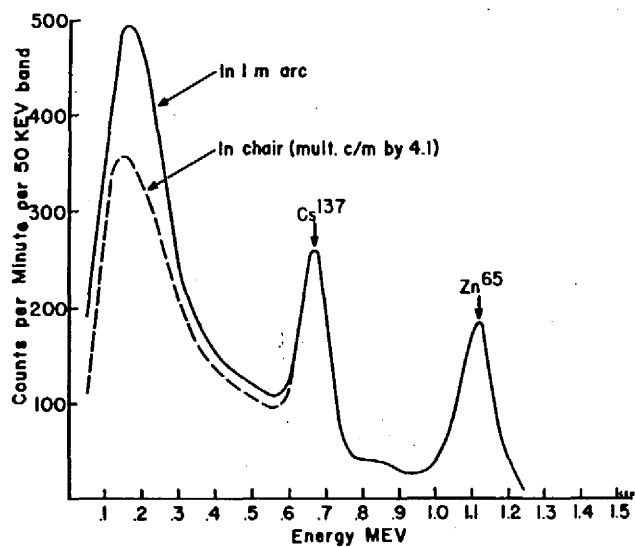
Fig. 22. Net in vivo gamma-ray spectra of Marshallese Subject No. 5
