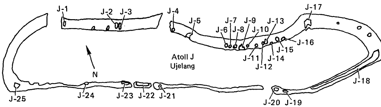
FIG. 14. Ujelang Atoll with code letter and numbers for the islands.
