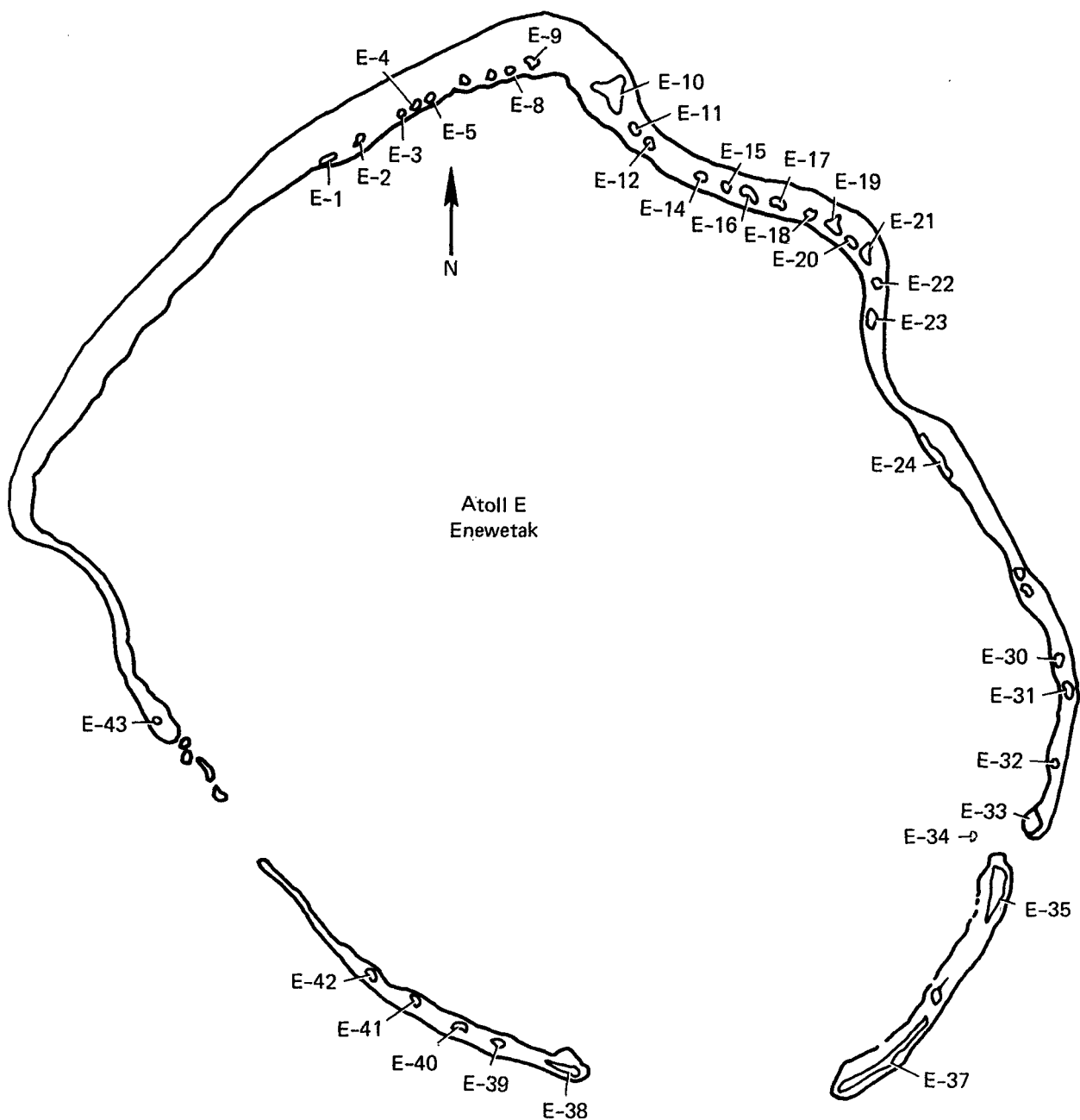
FIG. 16. Enewetak Atoll with code letter and numbers for the islands.
