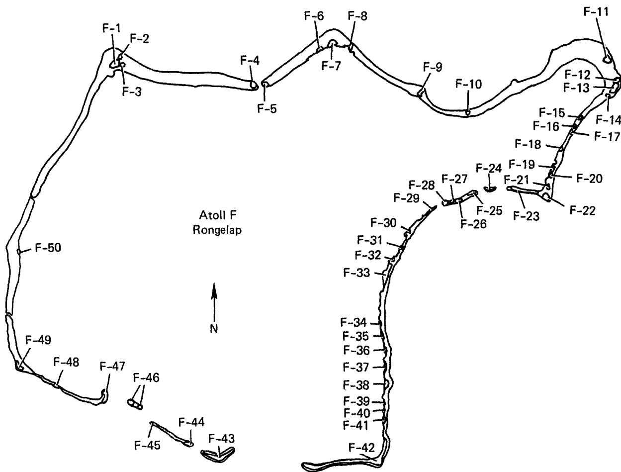
FIG. 2. Rongelap Atoll with code letter and numbers for the islands.
