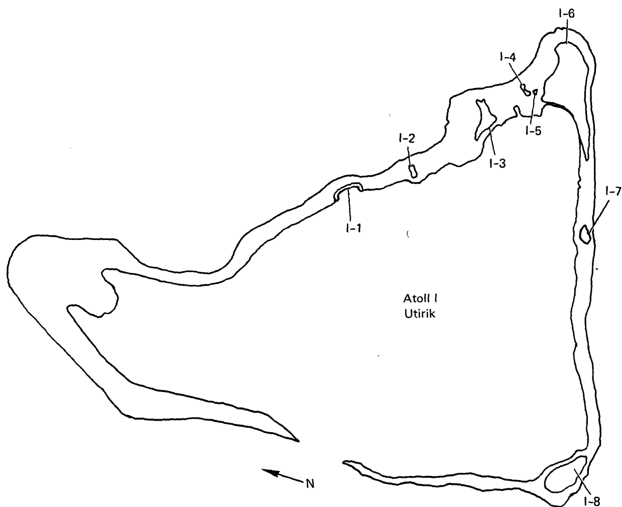
FIG. 4. Utirik Atoll with code letter and numbers for the islands.
