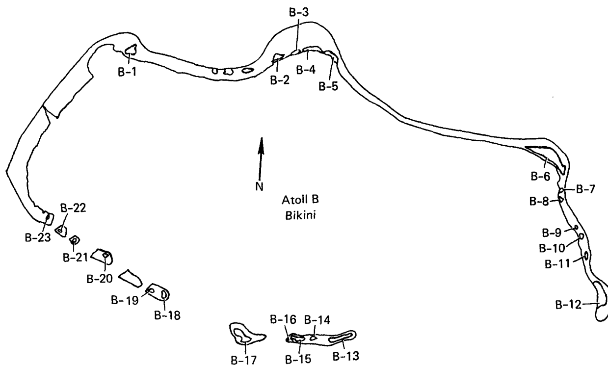
FIG. 15. Bikini Atoll with code letter and numbers for the islands.
