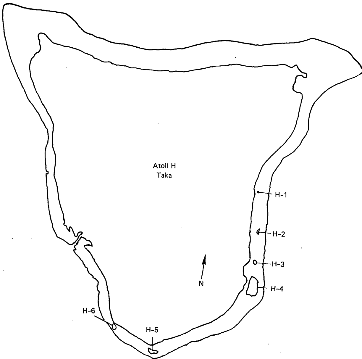
FIG. 3. Taka Atoll with code letter and numbers for the islands.
