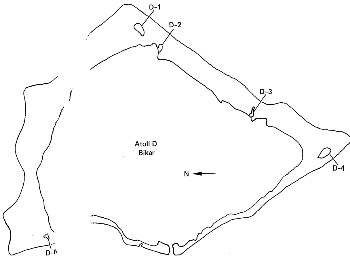
FIG. 5. Atoll D Bikar with code letter and numbers for the islands.
