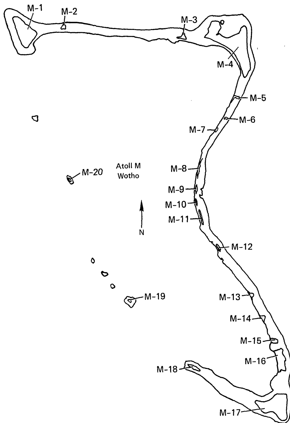
FIG. 13. Wothe Atoll with code letter and numbers for the islands.
