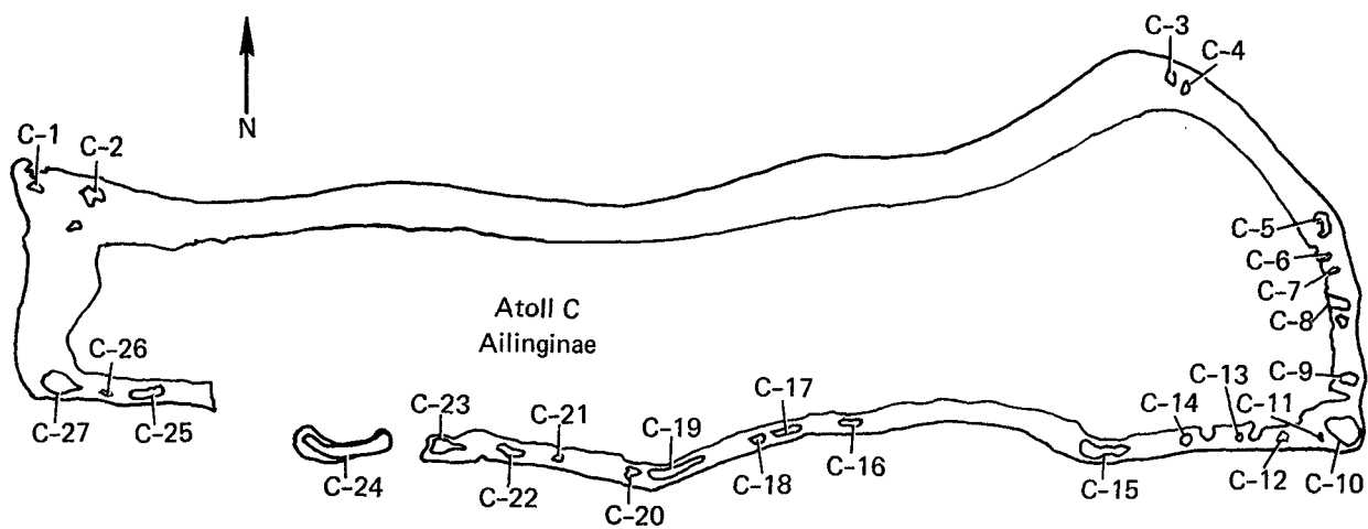
FIG. 7. Ailinginae Atoll with code letter and numbers for the islands.
