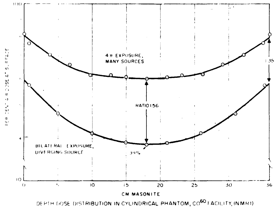
Fig. 1.4 Comparative Depth Doses for Bilateral Exposure from a Small Source and Multiple Source 4\pi Exposure with Cobalt-60
