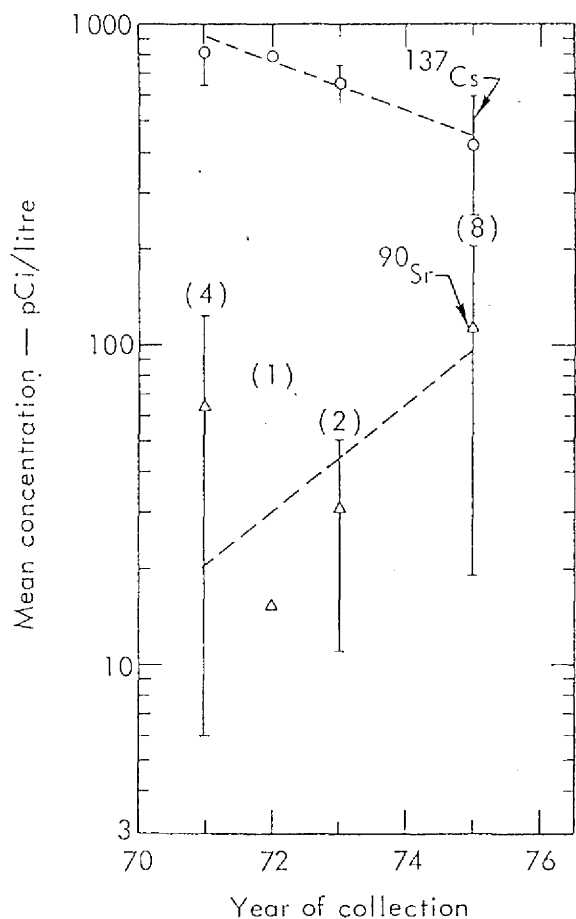
Fig. 5. Changes in groundwater concentrations of ^{137}\text{Cs} and ^{90}\text{Sr} with time at Bikini Island. Numbers in parentheses are the number of samples analyzed.
