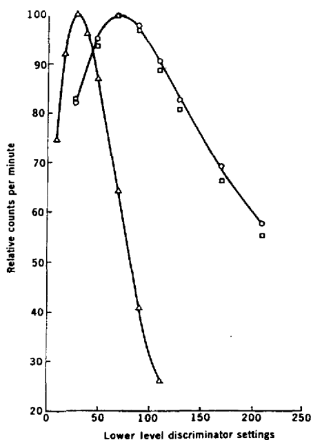
Fig. 1. Relative activity and discriminator settings for 59 Ni (Δ) and 63 Ni (O) spike solutions, plus the activity isolated from Tridacna gigas clam kidney collected from Bikini Atoll (□). Instrument settings were 20 percent gain and 4 percent window.
