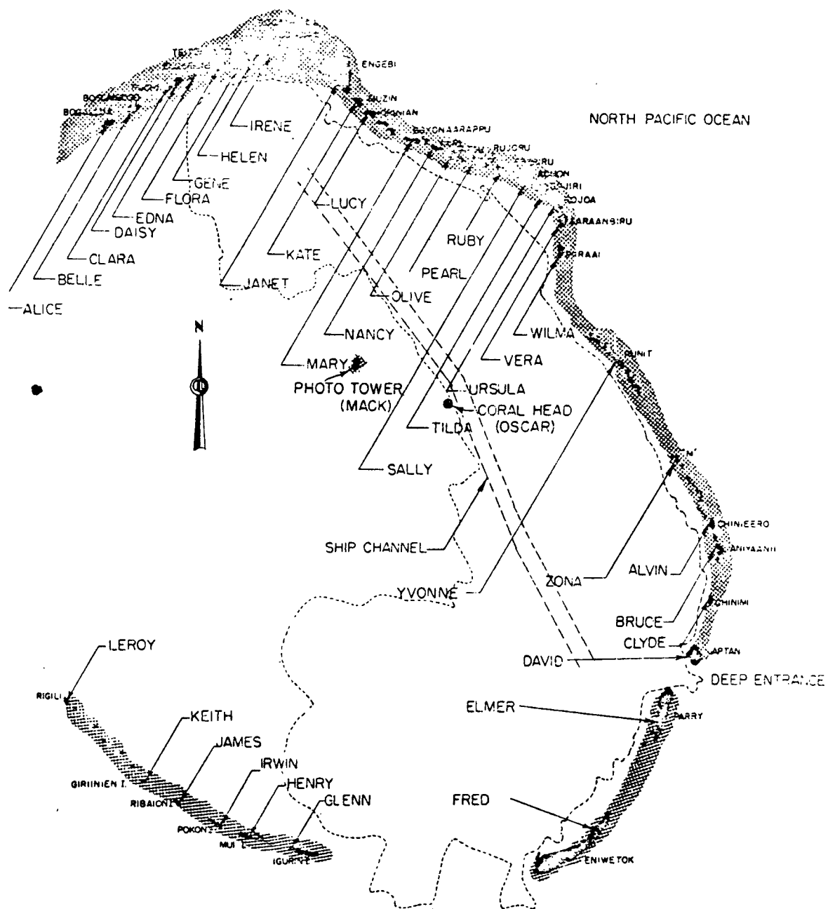
Fig. A.1 — Map of Eniwetok Atoll.
