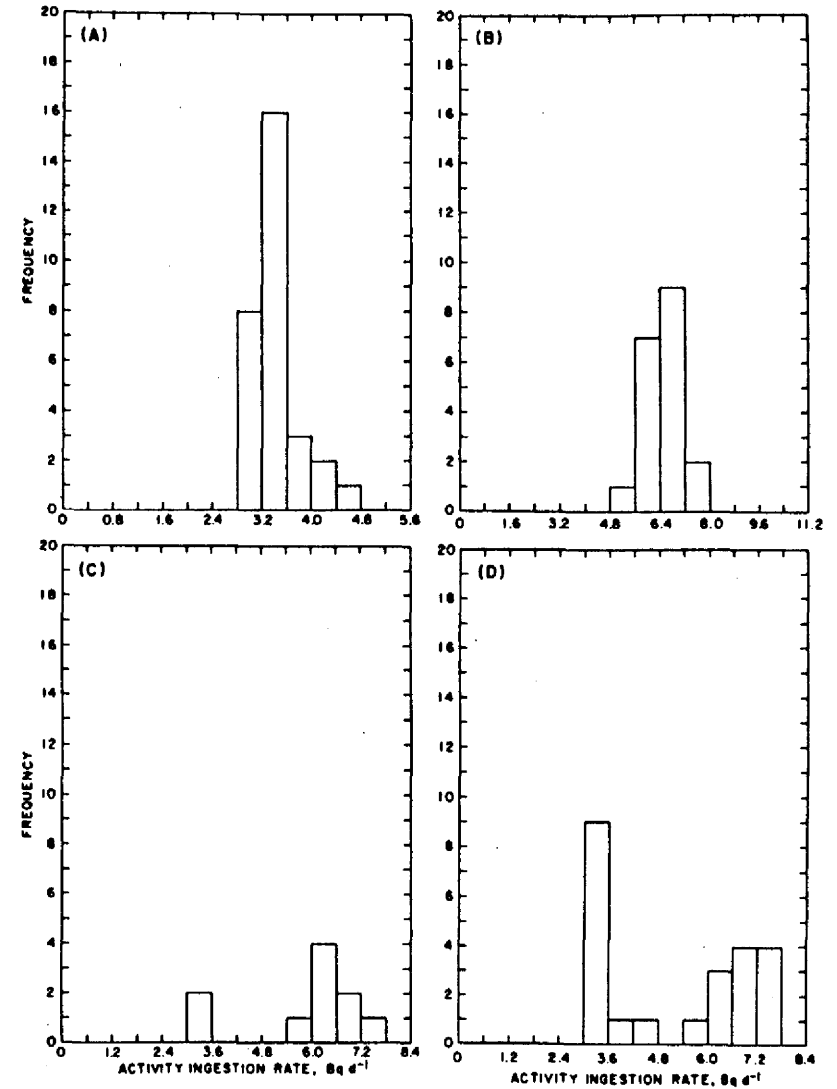
Fig. 13b 90 Sr Daily Activity Ingestion Rate for (A) Adult Males (B) Adult Females (C) Young Adults and (D) Children on Rongelap
