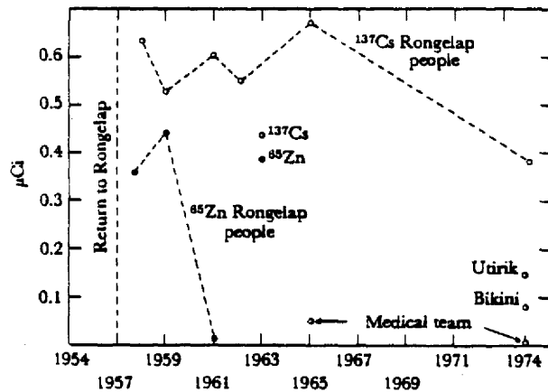
Figure 56. Body burdens of gamma emitters, obtained by whole-body gamma spectroscopy (○, 137 Cs; ●, 65 Zn).
