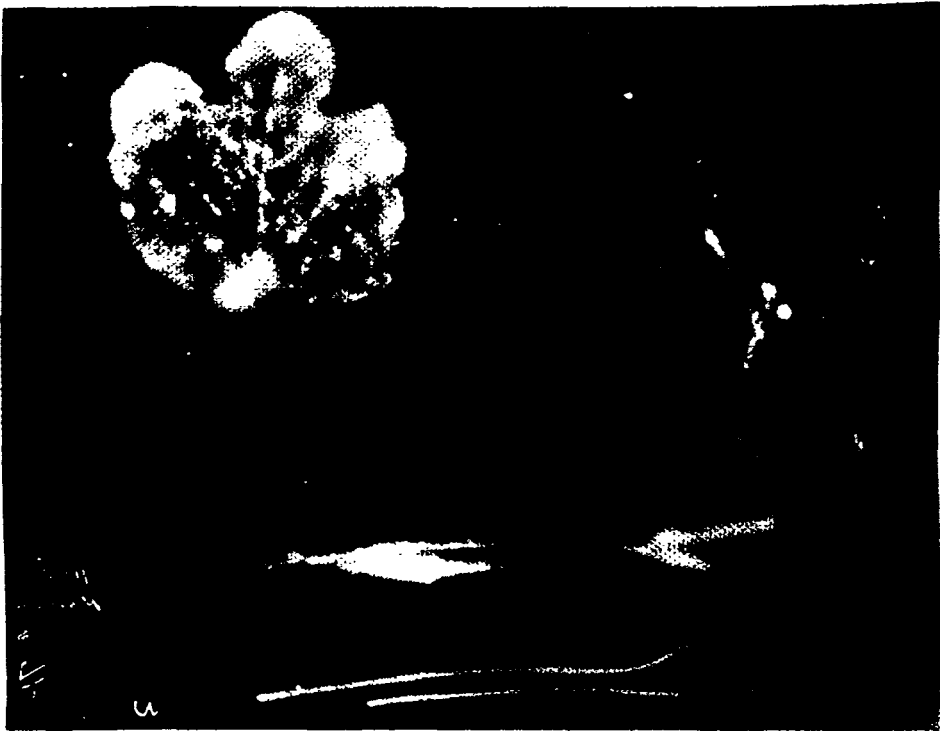
Figure 22 - Land plants from Engel, post shot. (a) Photo- graphs No. 297 and 299, portions of Timuletia groumiana ; No. 298, Timuletia ovata , upper portion not washed, lower portion washed with running tap water. (b) Autodiagraphs of the plants in (a), 7 days exposure to Super xx Pan film.
