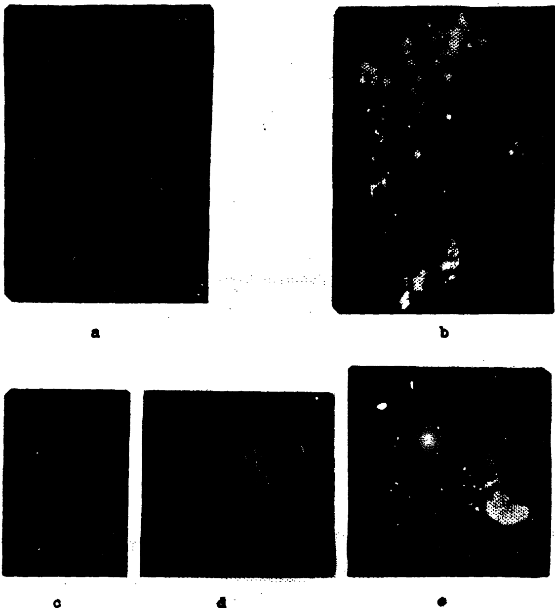
Figure 21. Autoradiographs of algae exposed to Super xx Pan Film. (a) Udo tea before washing, 2 1/2 hours exposure; (b) Udo tea , same plant after washing with detergent, 60 hours; (c) Lyngbia and (d) Bryopsis , 52 days; (e) Enteromorpha and Rhizoclonium , 60 days. (a) to (d) post shot, (e) pre-shot.
