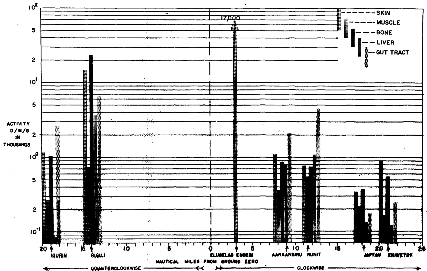
Figure 12. Histogram showing radioactivity of post shot terns with relation to distance of collecting site from ground zero, thousands of d/m/g wet sample.
