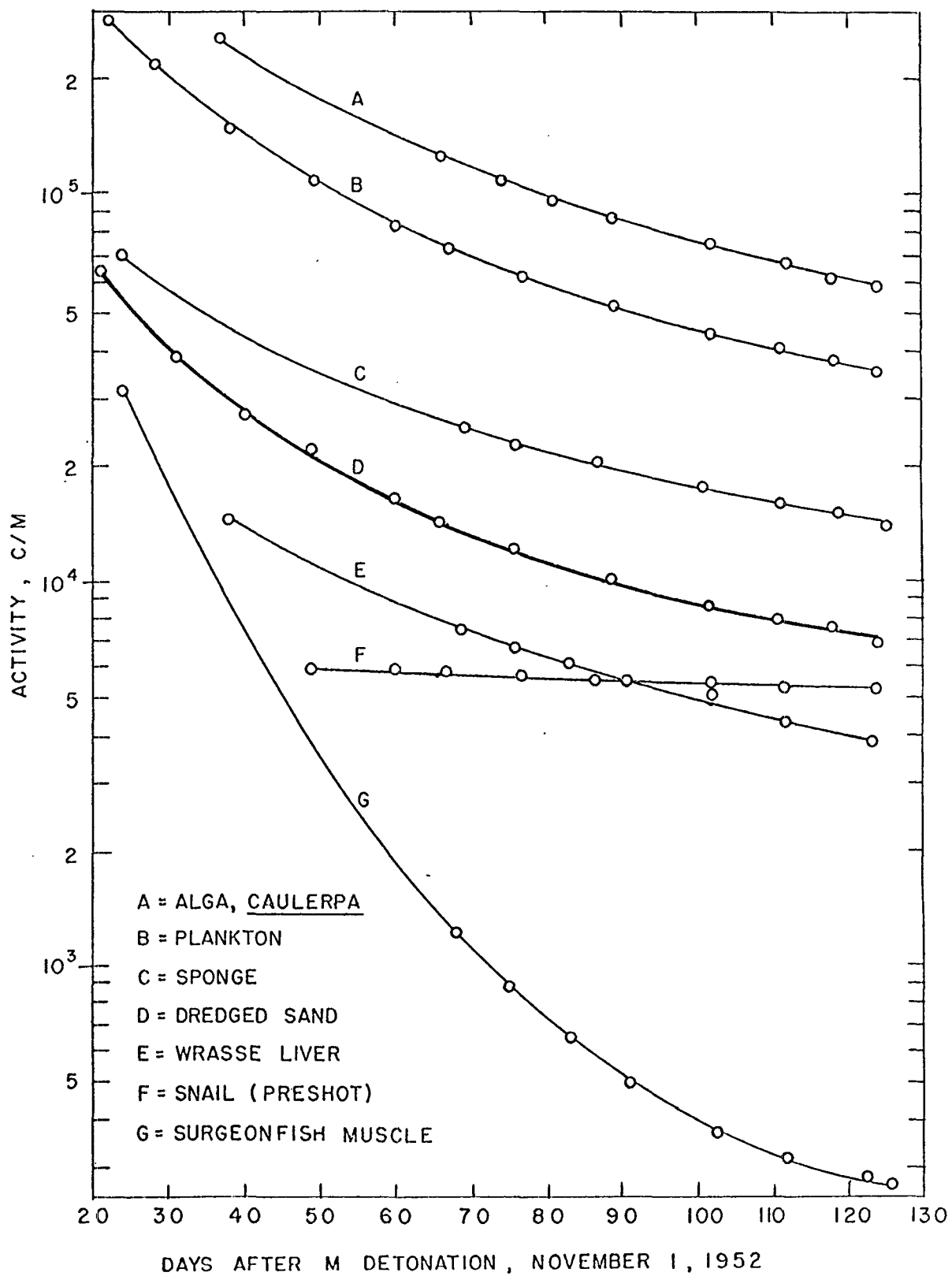
Figure 3. Decay curves.
