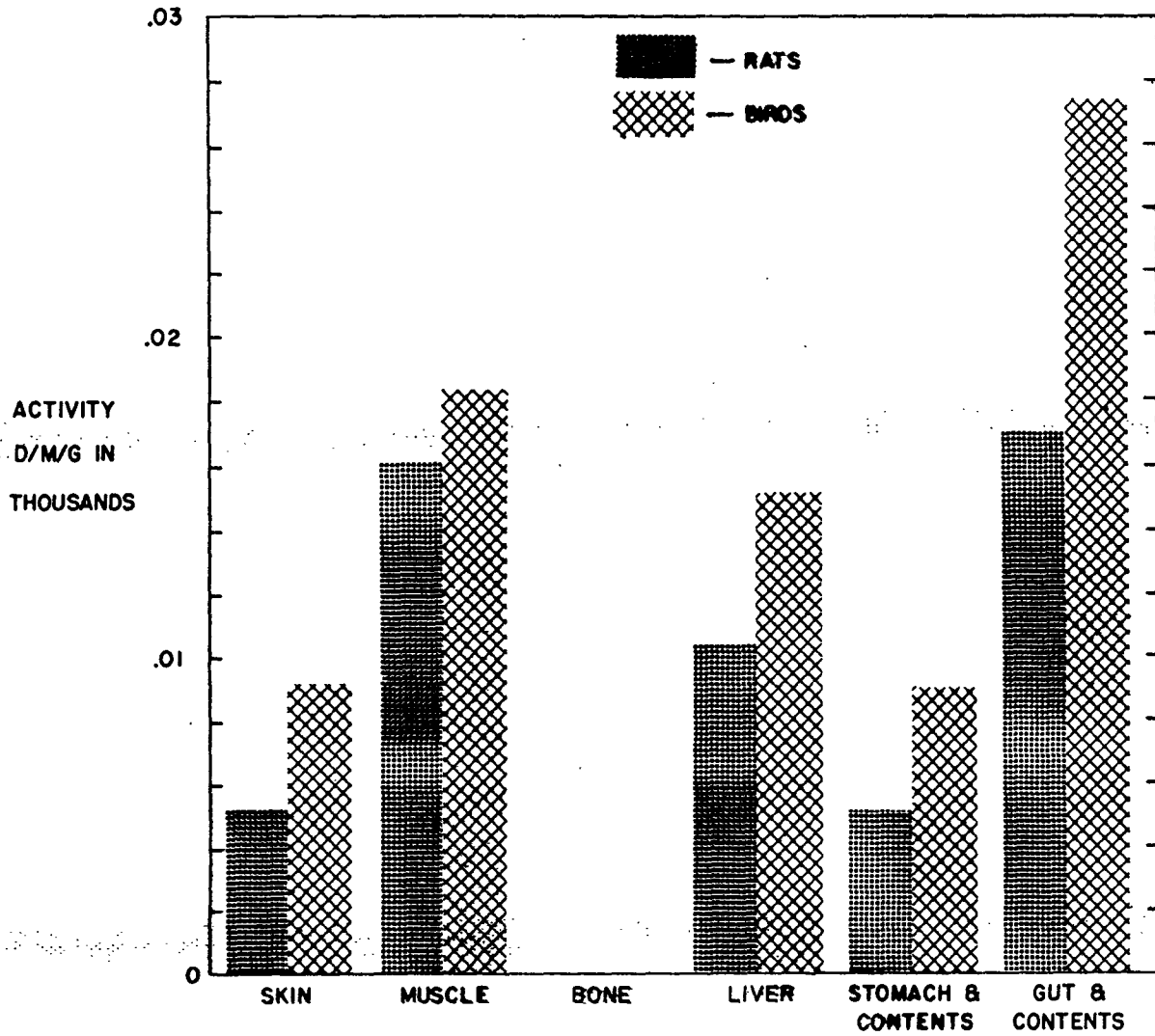
Figure 11. Radioactivity of pre-shot rats and birds, d/m/g wet sample.
