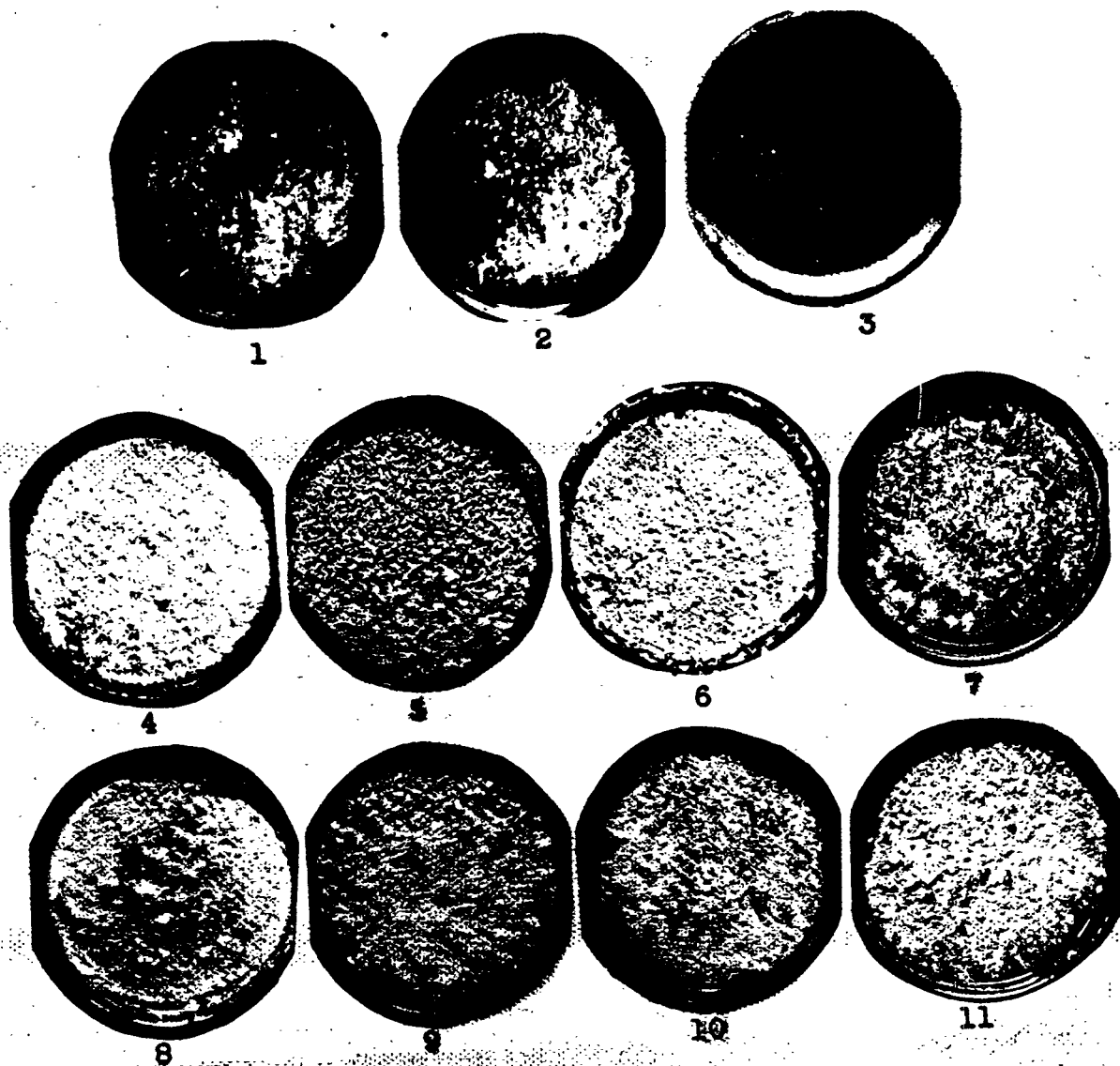
Figure 20 - Photographs approximately actual size of 11 of the more radioactive post test samples whose autoradiographs are shown in Figure 19. Orientations do not necessarily correspond in the two figures.
