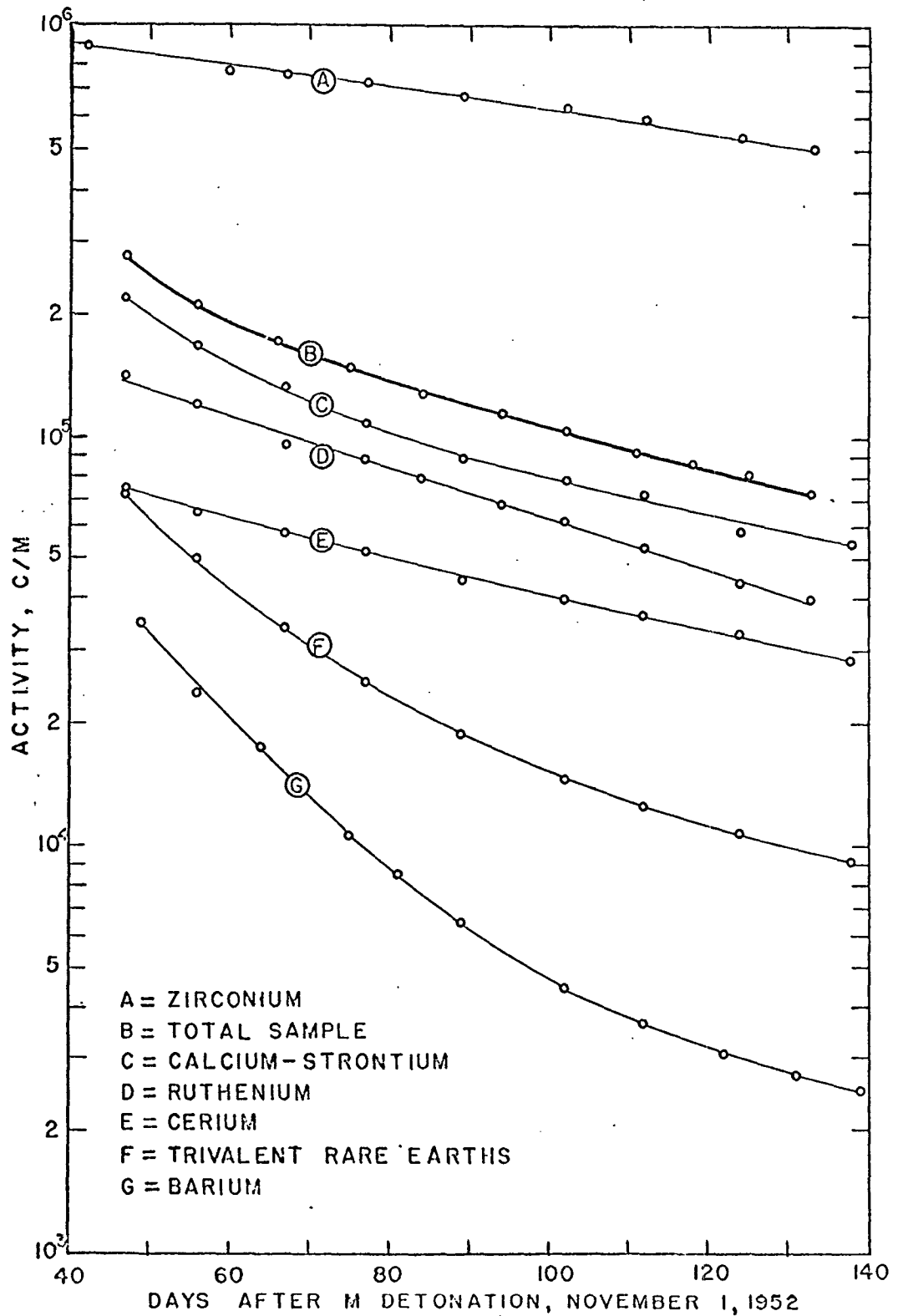
Figure 16. Decay curves of radiochemically-separated fractions of Rojoa dredged sand.
