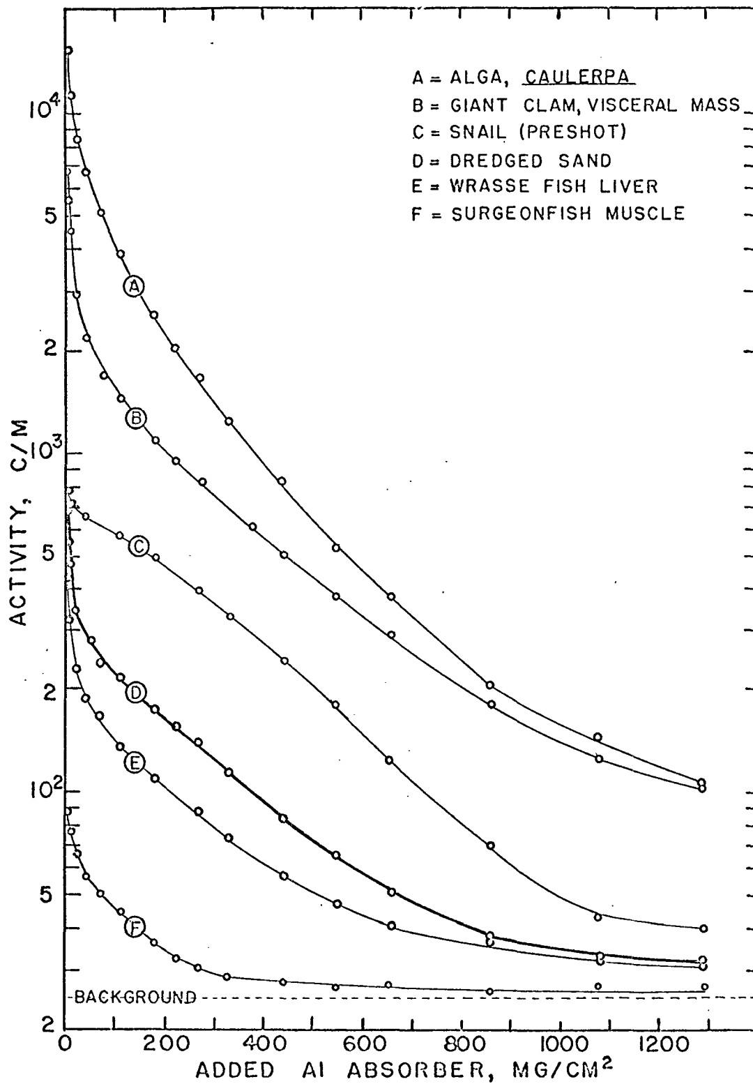
Figure 4. Mass Absorption curves.
