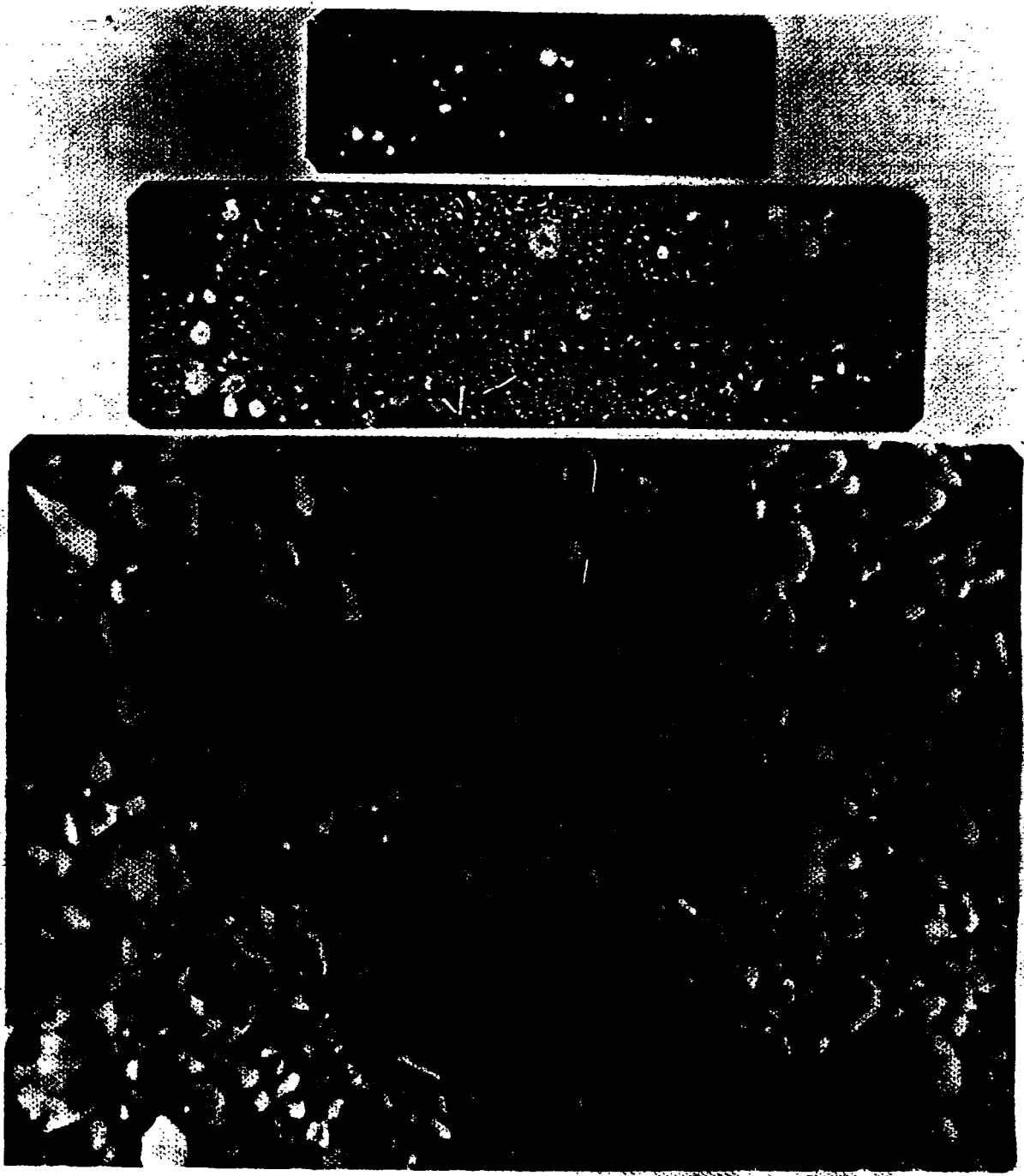
Figure 18 (upper). Autoradiograph actual size of Billiri- from measured using an 3/4-inch scotch tape. Figure 18 (middle). Photograph, 1.8x, of the same sand preparation partially illuminated from below through a positive transparency of its own autoradiograph. Figure 18 (lower). Photomicrograph, 20x, of the large radio- active particle near top center of preceding figure. This irregular, chainy particle weighing 0.6 mg, when removed to a plate on May 18, 1953, counted 5,300 in the Nucleometer.
