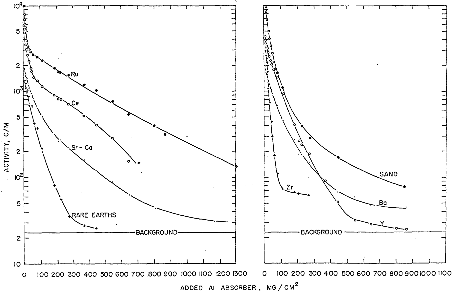
Figure 15. Mass absorption curves of radiochemically-separated fractions of Rojoa dredged sand
