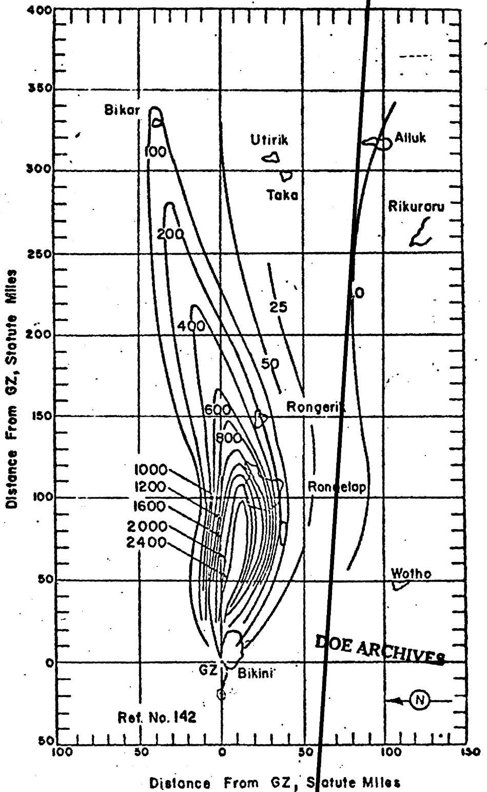
Operation CASTLE - Shot 1 - Bravo. Off-site dose rate contours in r/hr at H+1 hour (P)
