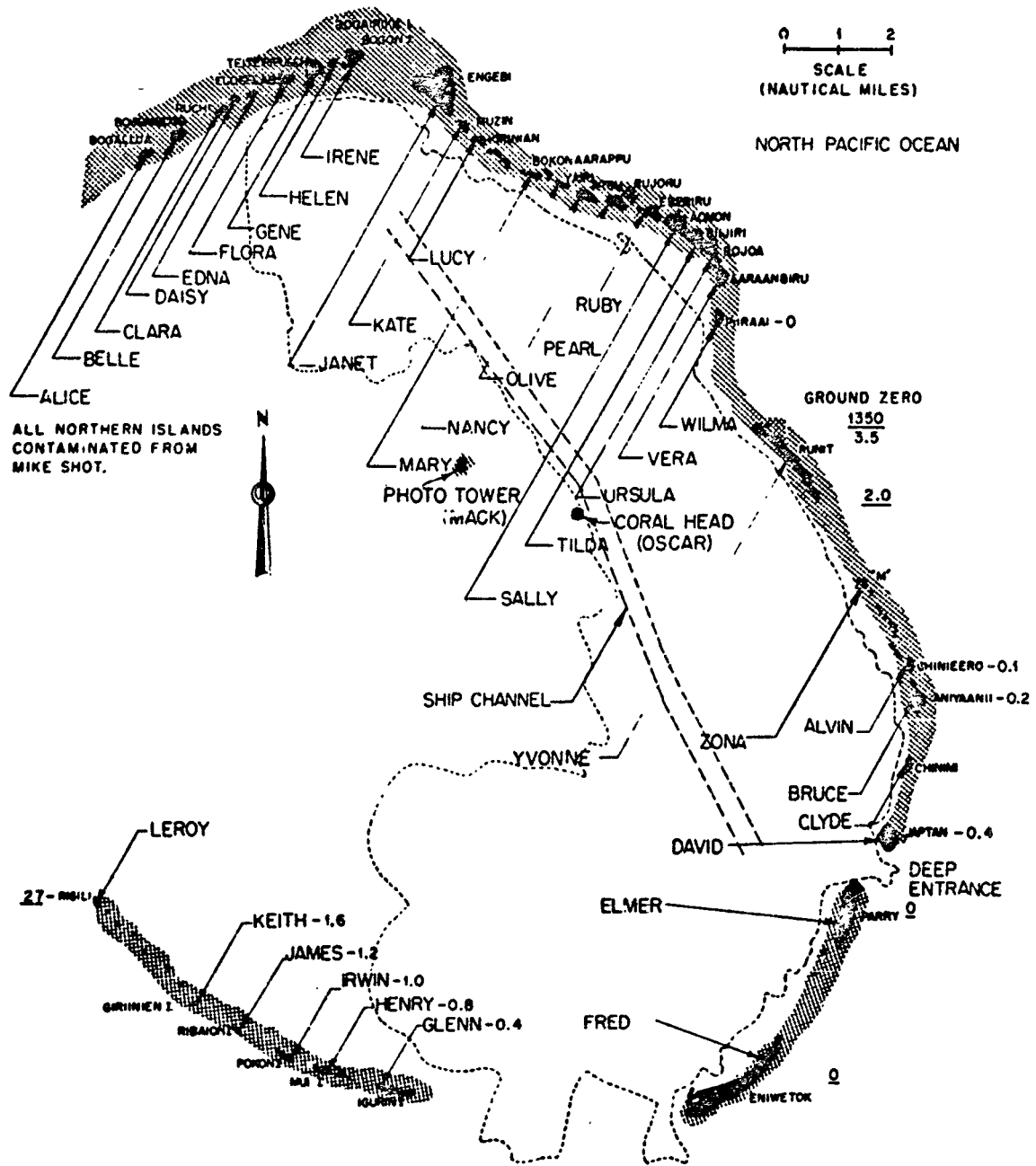
Fig. 10.2 — King shot, H + 5 hr. Underlined readings are ground values in milliroentgens per hour; other readings are helicopter readings 25 ft above ground in milliroentgens per hour.
