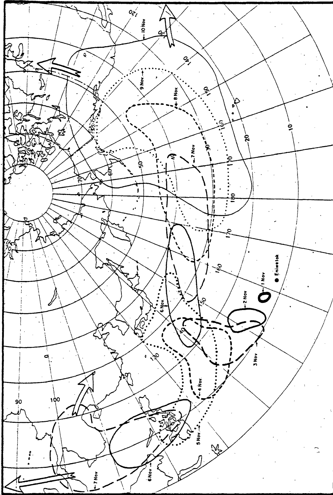
Figure 3.2 Schematic outlines, daily at 1500 GCT, trade wind portion of the MIKE cloud
