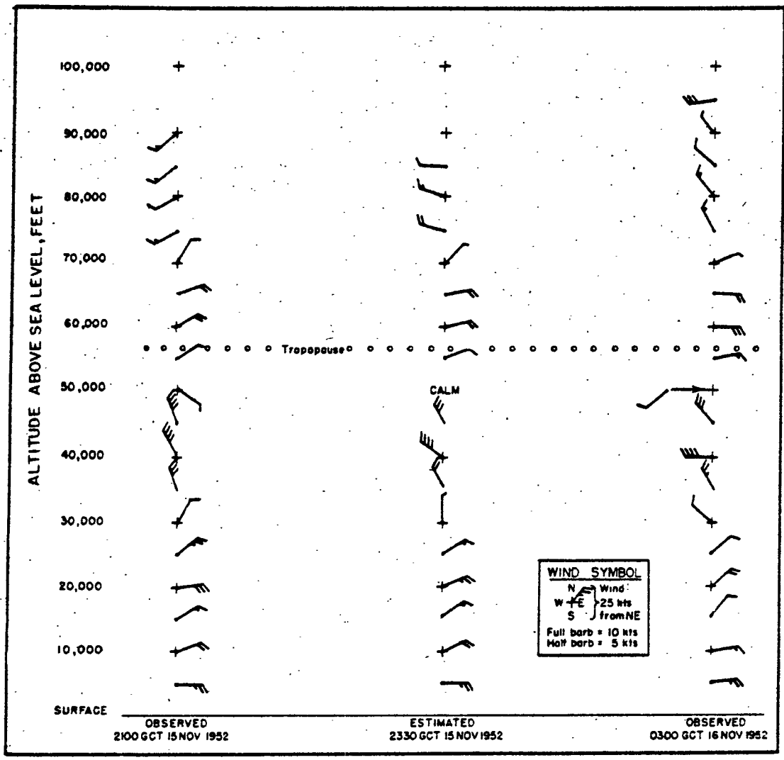
Figure 4.1 Winds aloft — KING burst
