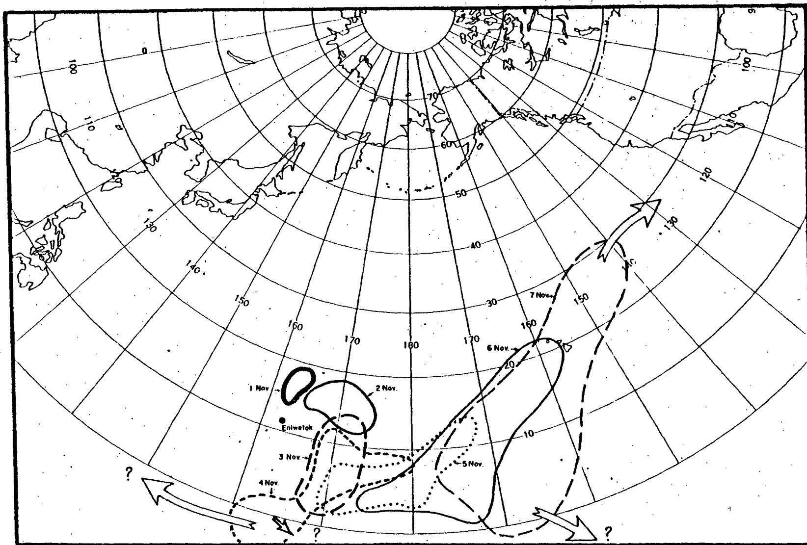
Figure 3.3 Schematic outlines, daily at 1500 GCT upper troposphere portion of the MIKE cloud
