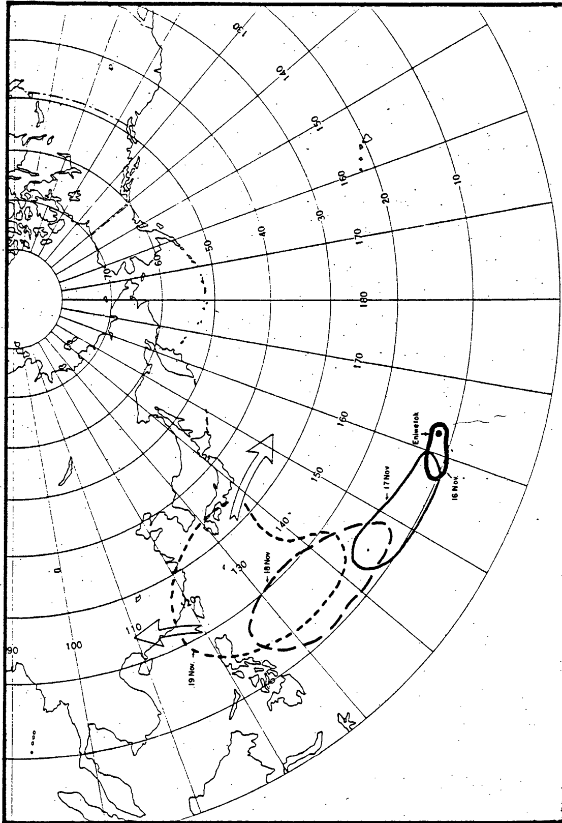
Figure 4.4 Schematic outlines, daily at 1500 GCT, stratosphere portion of the KING cloud
