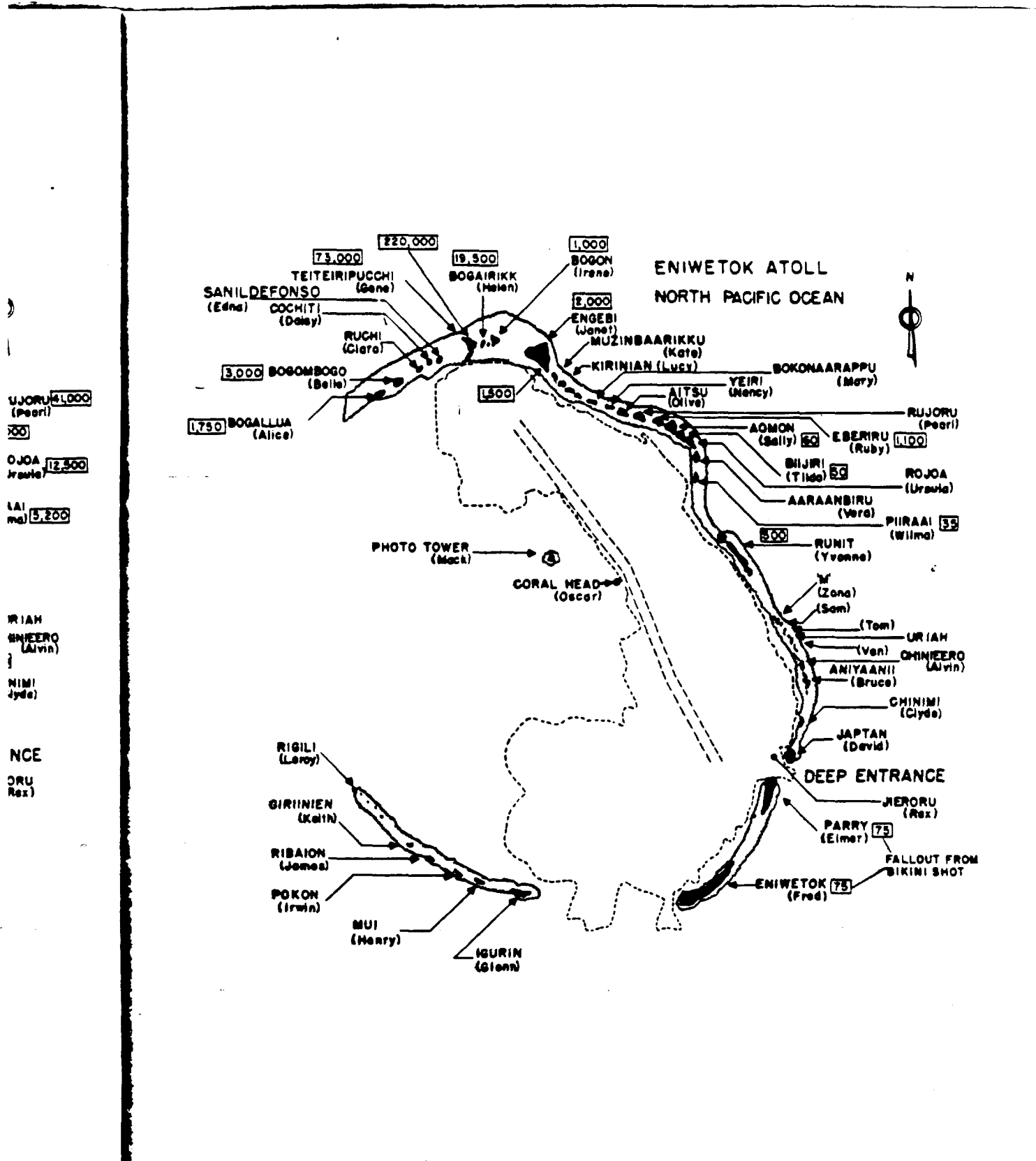
Fig. 2.10 [redacted] intensities on Eniwetok Atoll at H+4 hr, in milliroentgens per hour. Shot site was Mike crater.
