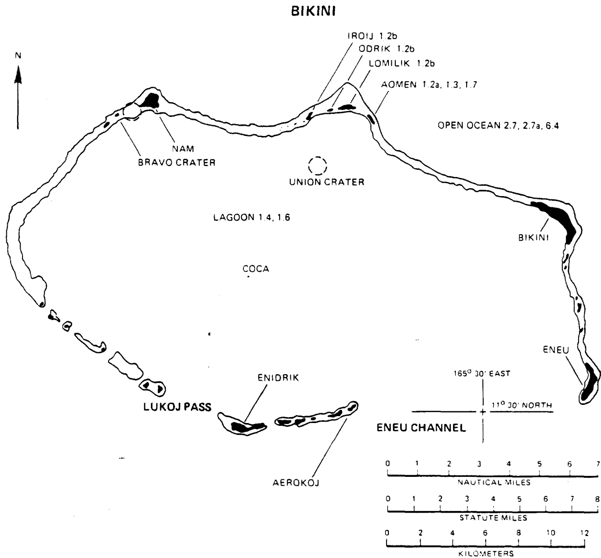
Figure 86. CASTLE, YANKEE instrumentation stations for the DOD scientific projects at Bikini Atoll.
