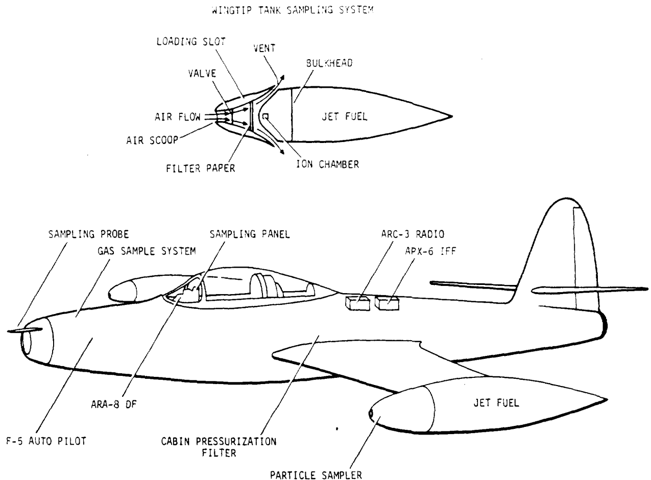
Figure 23. F-84G sampler aircraft, CASTLE.
