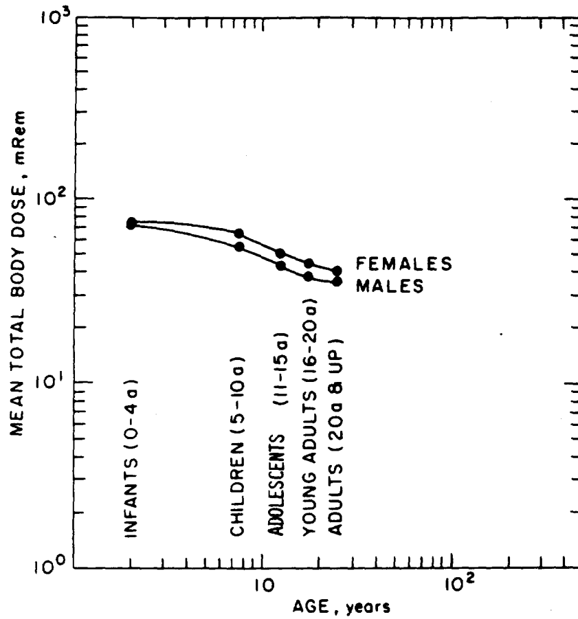
Fig. 22 Age and Sex Groups Mean Values for 90 Sr Dose Equivalent For The Interval 1957 to 1980 at Rongelap Atoll
