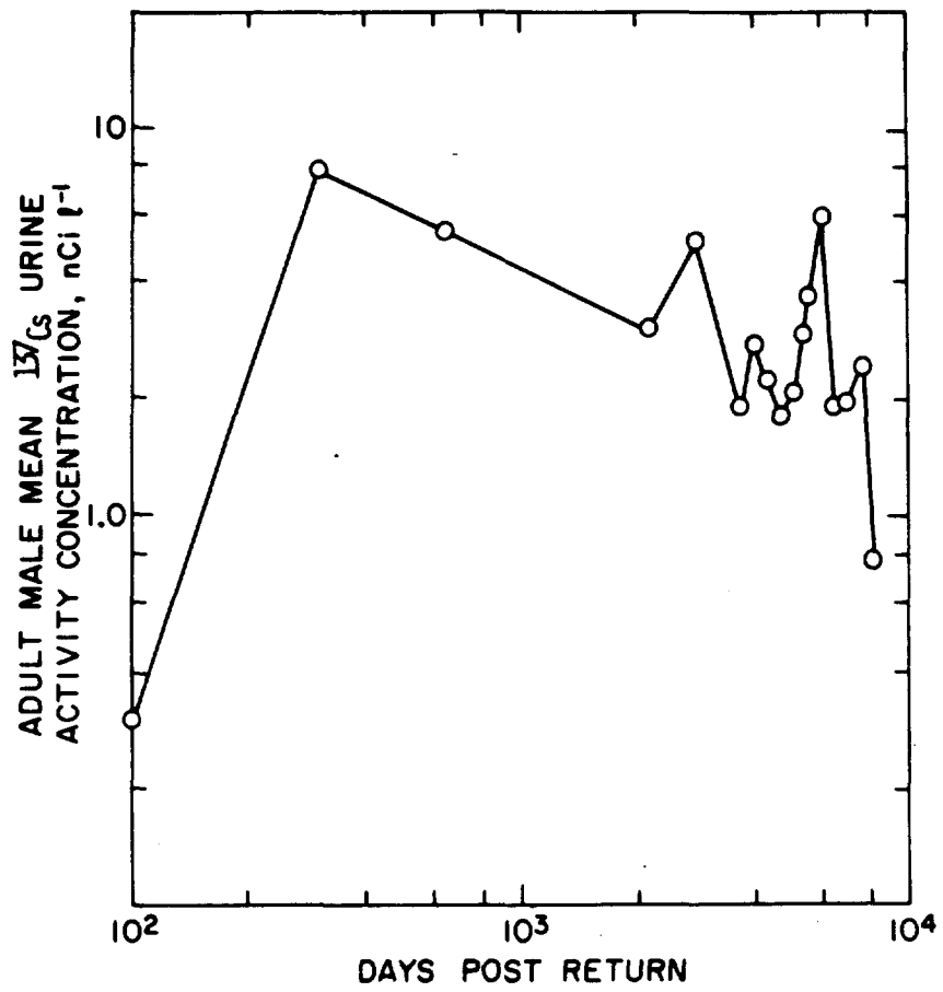
Fig. 6 Mean Adult Male 137 Cs Urine Activity Concentration History at Rongelap Atoll
