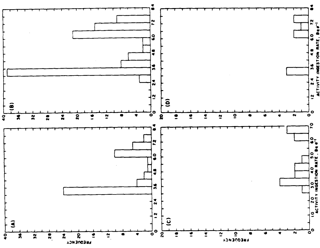
Fig. 13a ^{90}\text{Sr} Daily Activity Ingestion Rate For (A) All Residents (B) Infants and (D) Adolescents on Rongelap
