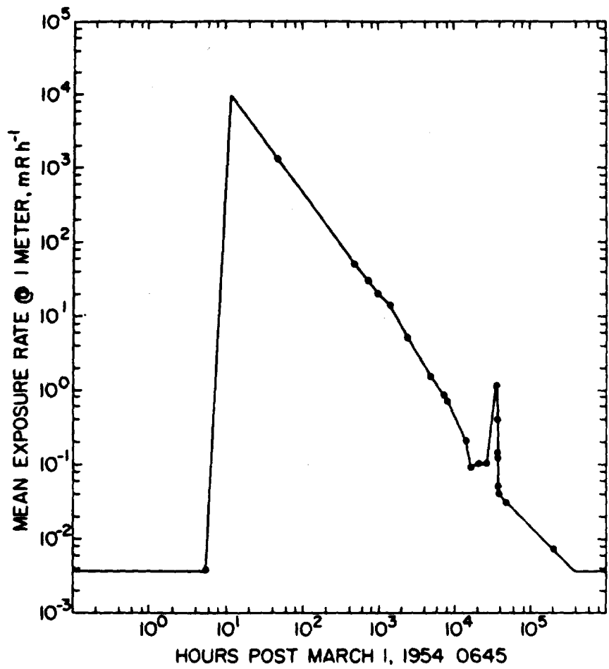
Fig. 24 Rongelap External Exposure Rate History Post Bravo
