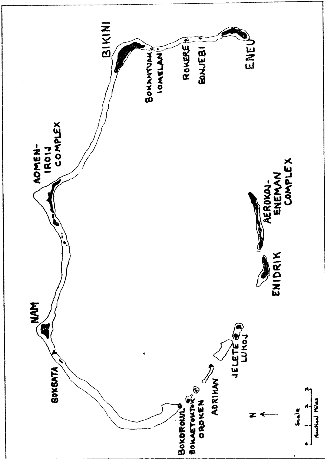
Figure 1 - Palmyra Atoll
