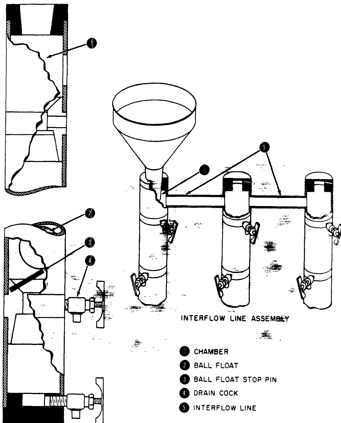
Fig. 3.4—Incremental liquid fall-out collector.
