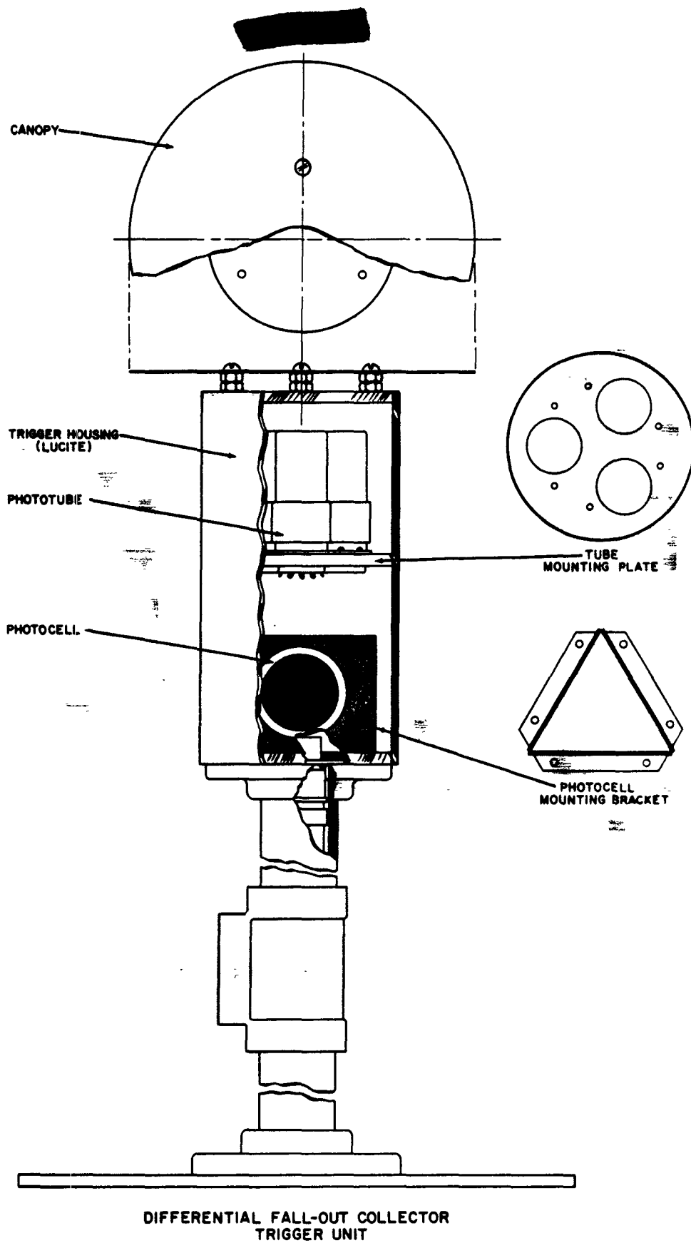
Fig. 3.3—Light-actuated trigger mechanism.
