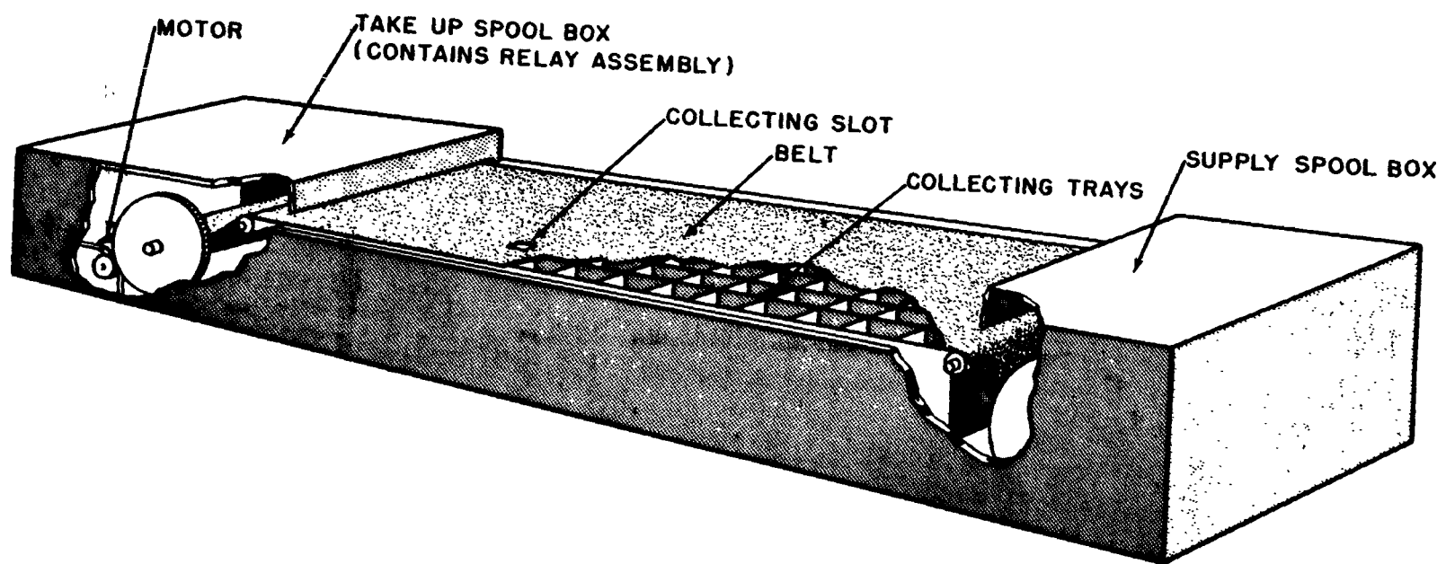
Fig. 3.2—Differential fall-out collector.
