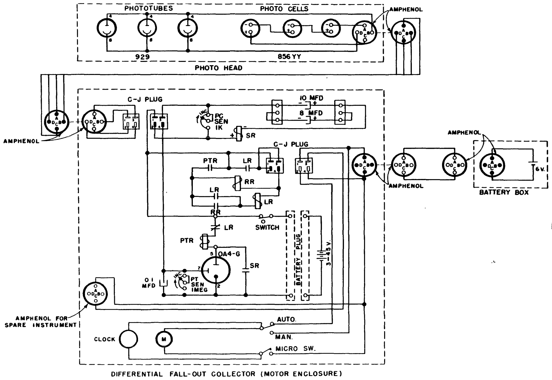
Fig. C.1—Schematic diagram of the electronic trigger mechanism.
