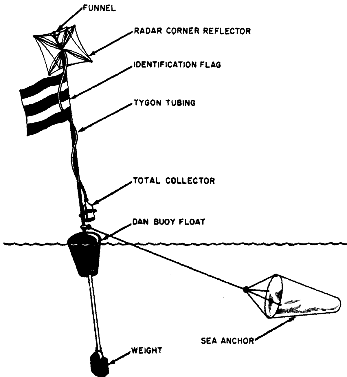
Fig. 3.10—Free-floating sea station.
