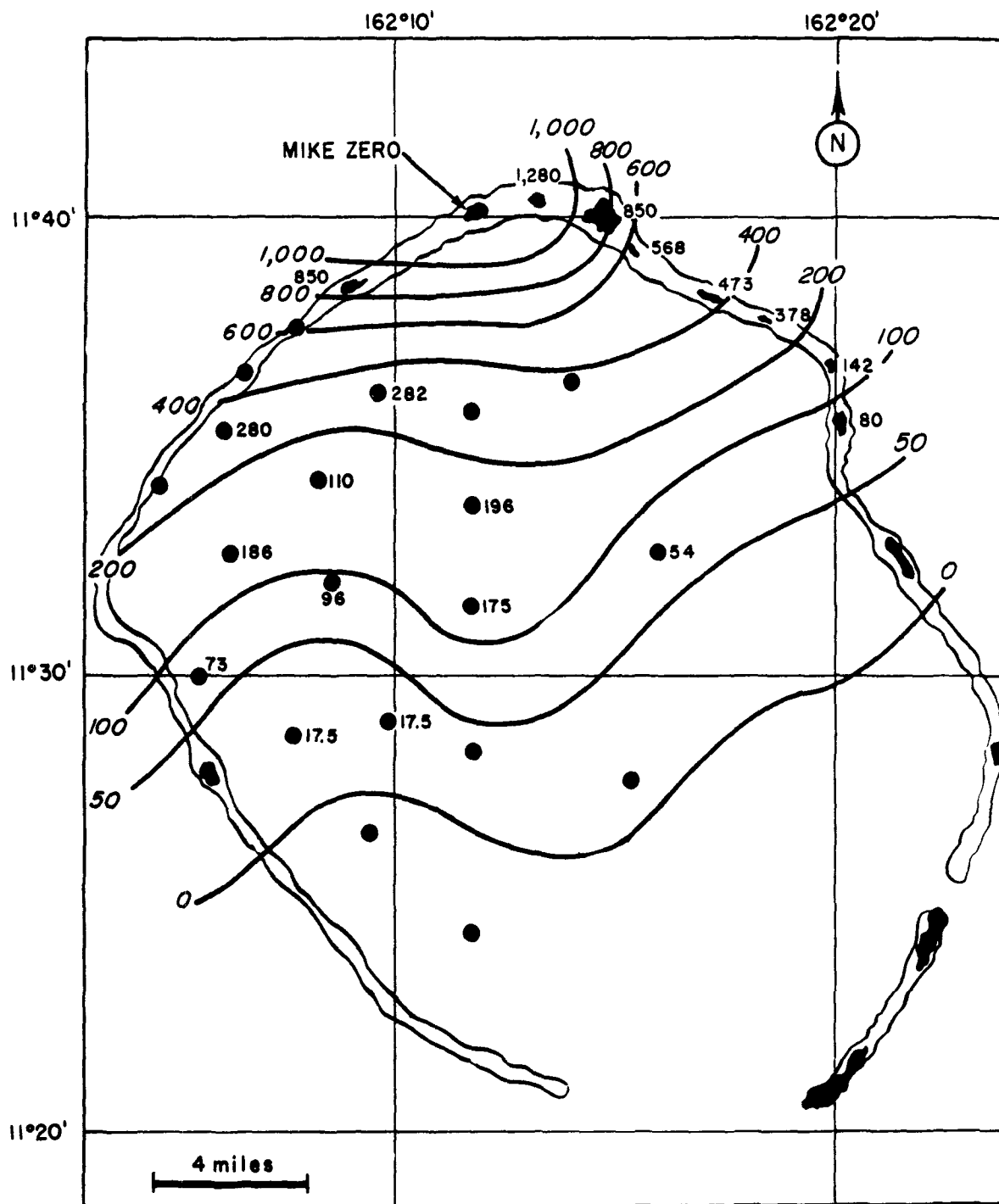
Fig. 4.1—Fall-out gamma pattern at 2 hr as would be experienced on a land mass (r/hr).
