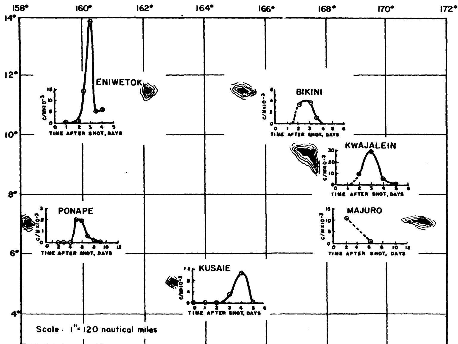
Fig. 5.2—Periods of secondary fall-out at the outer island stations.
