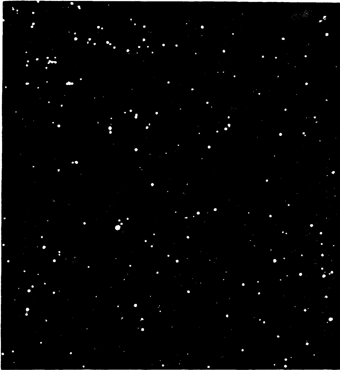
Fig. 5.1—Radioautograph of secondary fall-out particles.
