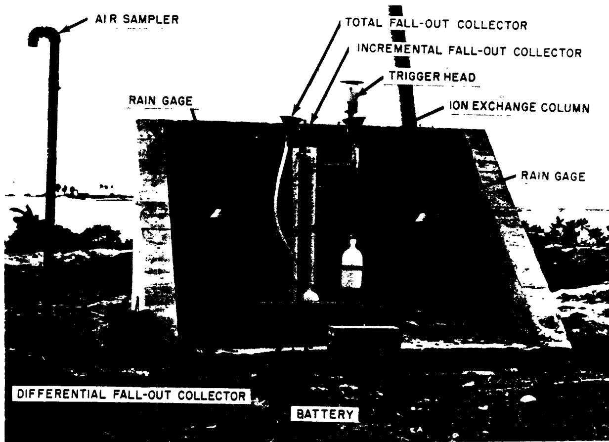
Fig. 3.8—A typical land station.
