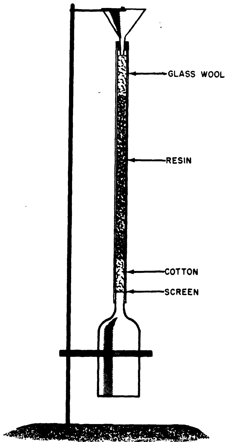
Fig. 3.6—Ion-exchange-column collector.
