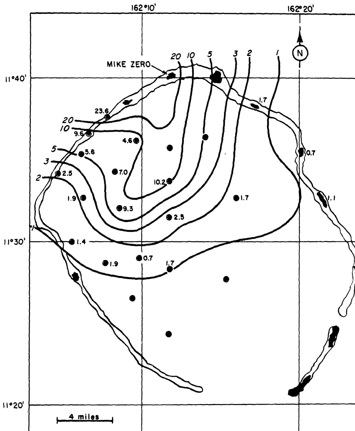
Fig. 4.8—Mass distribution of fall-out (g/sq ft).
