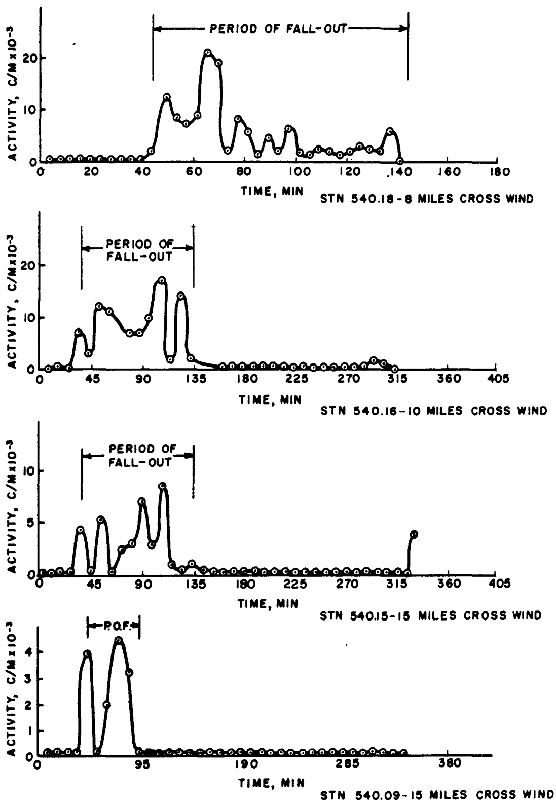
Fig. 4.11—Periods of primary fall-out at different stations.
