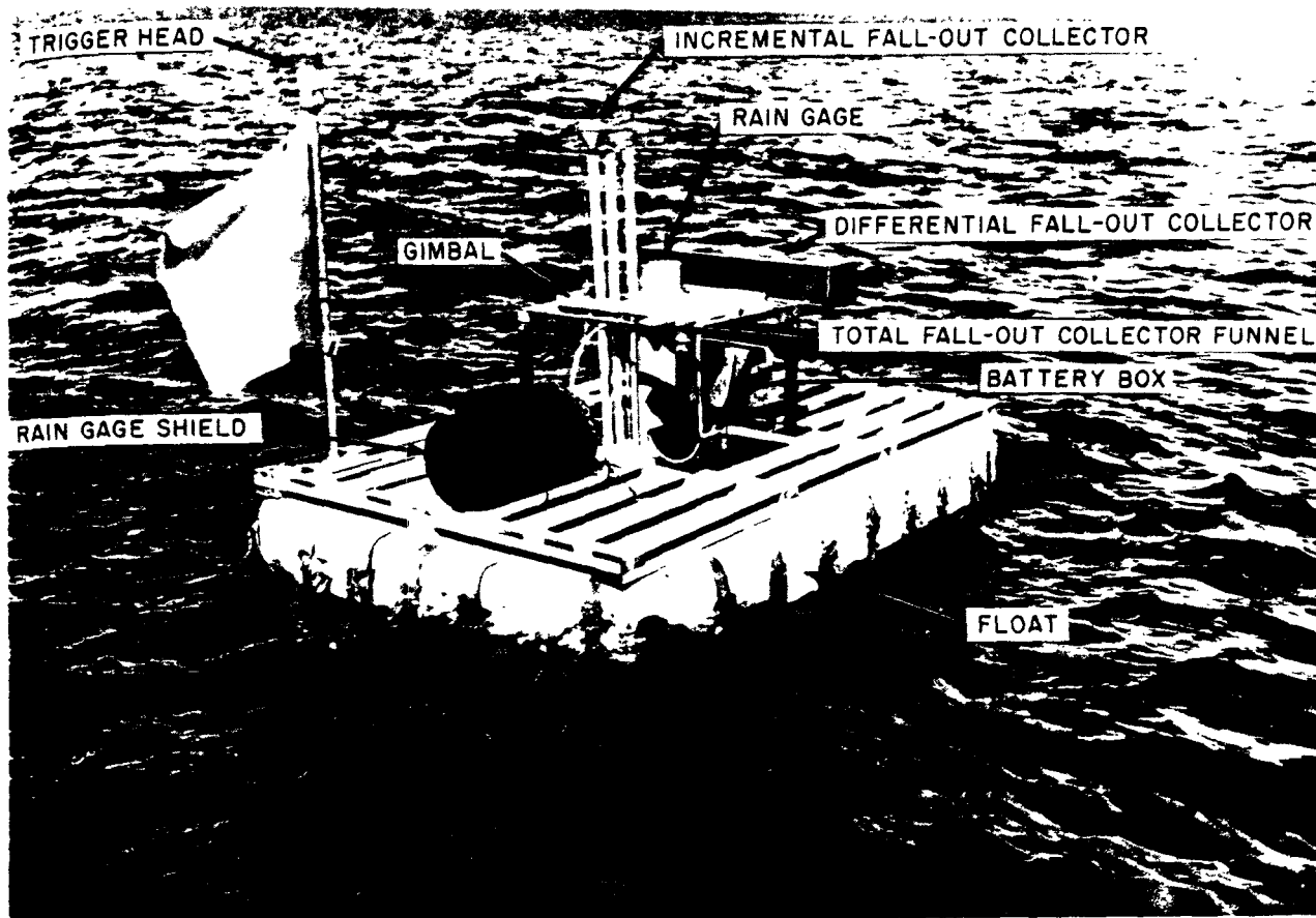
Fig. 3.9—A typical lagoon station.
