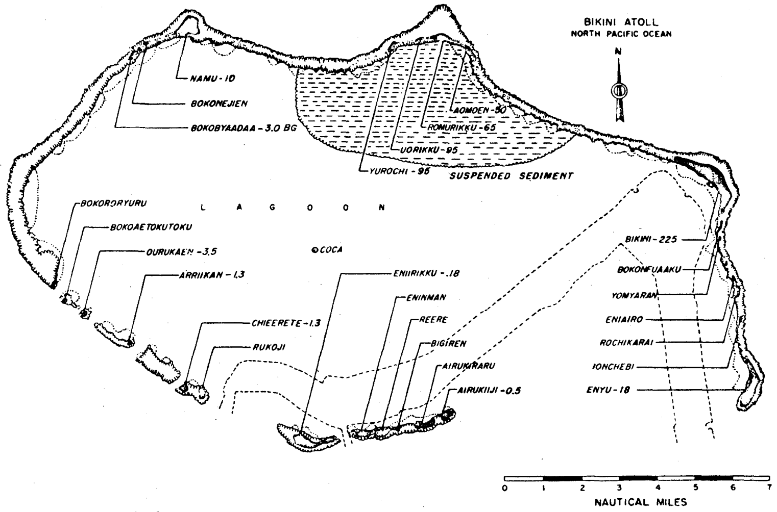
YANKEE Fig. 4.12- Radiation intensities in roentgens per hour extrapolated to H + 4 hr, plus background (bg) for Bokobyadaa. Location, UNION anchorage (barge). Yield, 14 Mt Time fired, 05/0610M May 1954.
