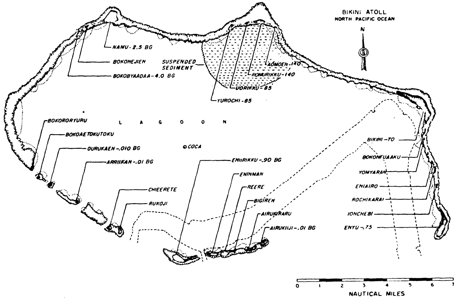
UNION Fig. 4.11 — radiation intensities in roentgens per hour extrapolated to H + 4 hr, plus background levels (bg) for some islands. Location, intersection of arcs with radii of 6900 ft from Yurochi and 3 nautical miles from Aomoen (barge). Yield, 7 Mt) _____, Time fired, 26/0610M April 1954.
