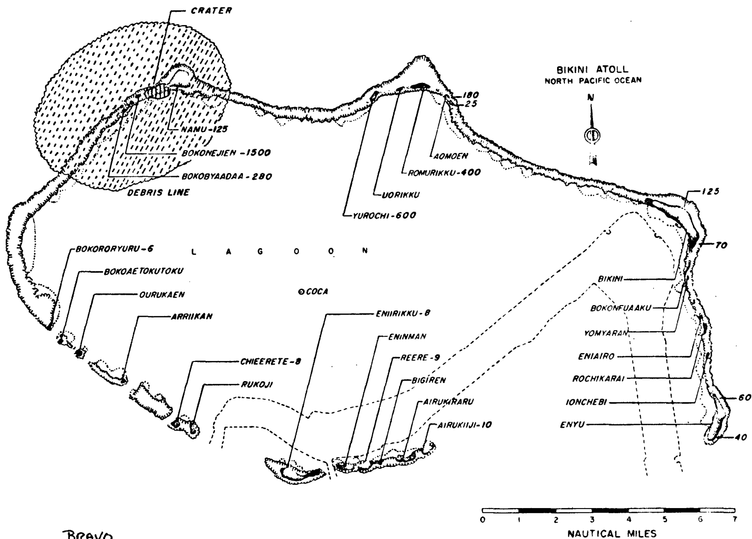
Fig. 4.1-1 radiation intensities in roentgens per hour extrapolated to H + 4 hr. Location, on reef 2950 ft; bearing, 250 deg true from southwest tip of Namu. Yield, 15 Mt. Time fired, 01/0645M March 1954.
