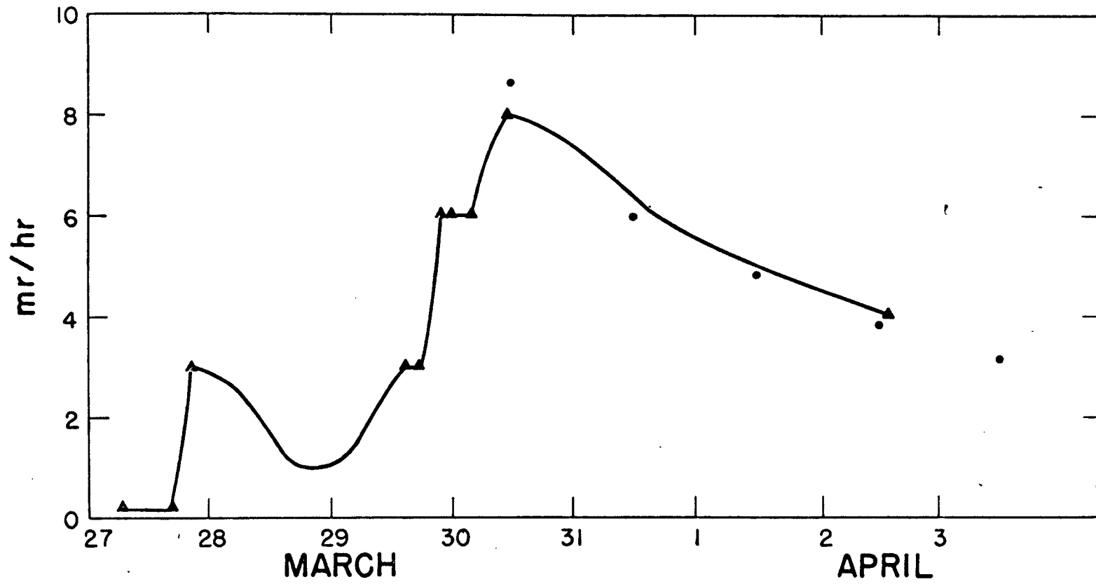
Fig. 4.9 R0MEO radiation fall-out, Parry Island.
