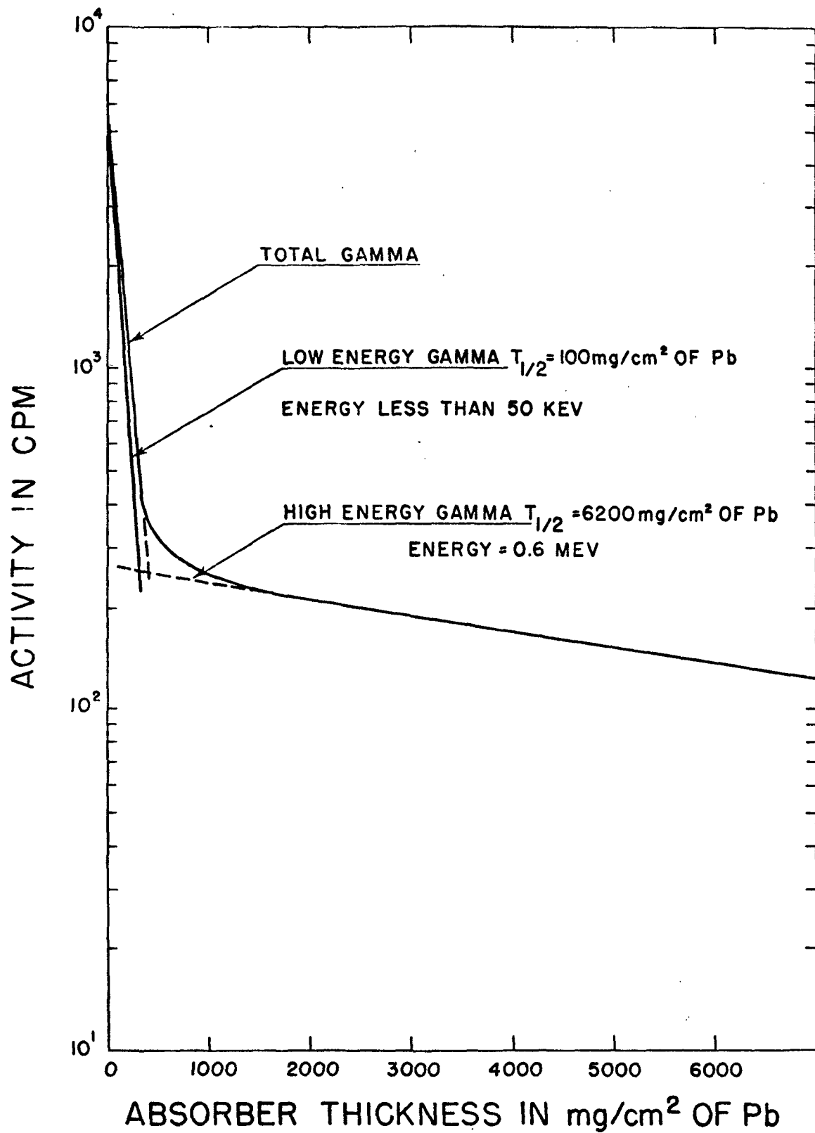
Fig. 5.4—Gamma-absorption curve.
