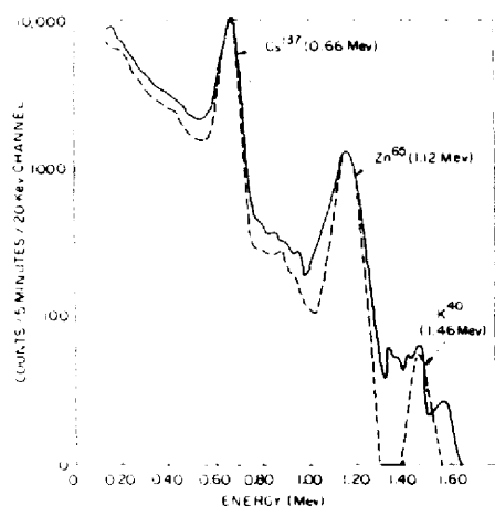
Figure 52. Gamma spectra of Marshallese male (subject \bar{x} 4, age 40, wt 70 kg—solid line) and normalized plastic phantom (containing 0.61 \mu\text{C} \text{Zn}^{65} , 1.22 \mu\text{C} \text{Cs}^{137} , and 110 g \text{K}^{40} )—(dashed line), 1959.
