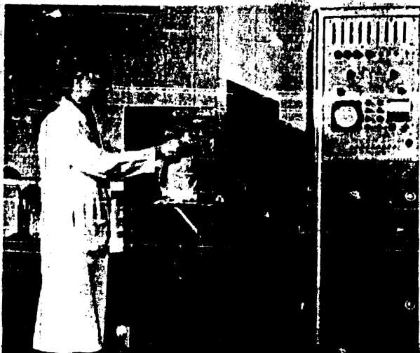
U.S. PUBLIC HEALTH SERVICE, DIVISION OF RADIOLOGICAL HEALTH PHOTO FIGURE 6. Counting a sample of milk for iodine 131. The procedure is quick and simple—the milk is merely poured into a plastic container and set into the counter. In contrast, analysis of milk for strontium 90 may require weeks including radiochemical preparation of the sample.
