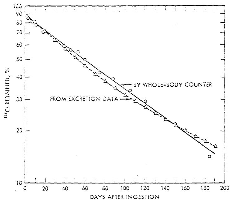
Fig. 5—Percent retention of ^{137}\text{Cs} from Rongelap food.
