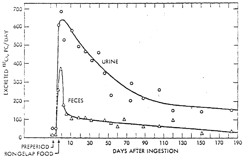
Fig. 1—Excretion of ^{137}\text{Cs} following ingestion of Rongelap food.
