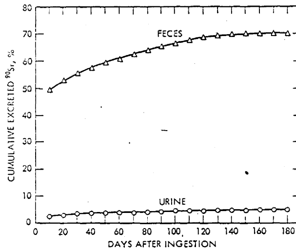
Fig. 1—Cumulative urinary and fecal excretions of ^{90}\text{Sr} following ingestion of Rongelap food.
