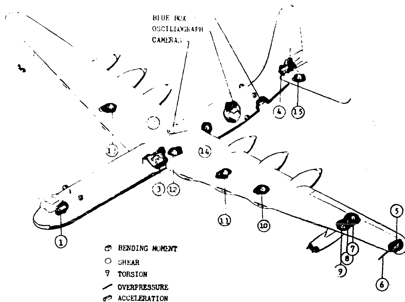
Fig. 2.7 Location of Instrumentation in E-36D Aircraft for IVY
