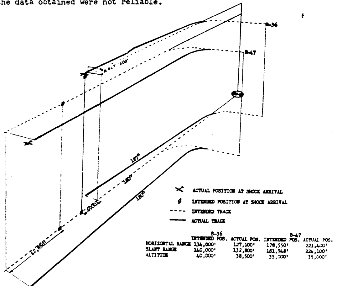
Fig. 3.1 Position of B-36D and B-47B Aircraft for Mike Shot
