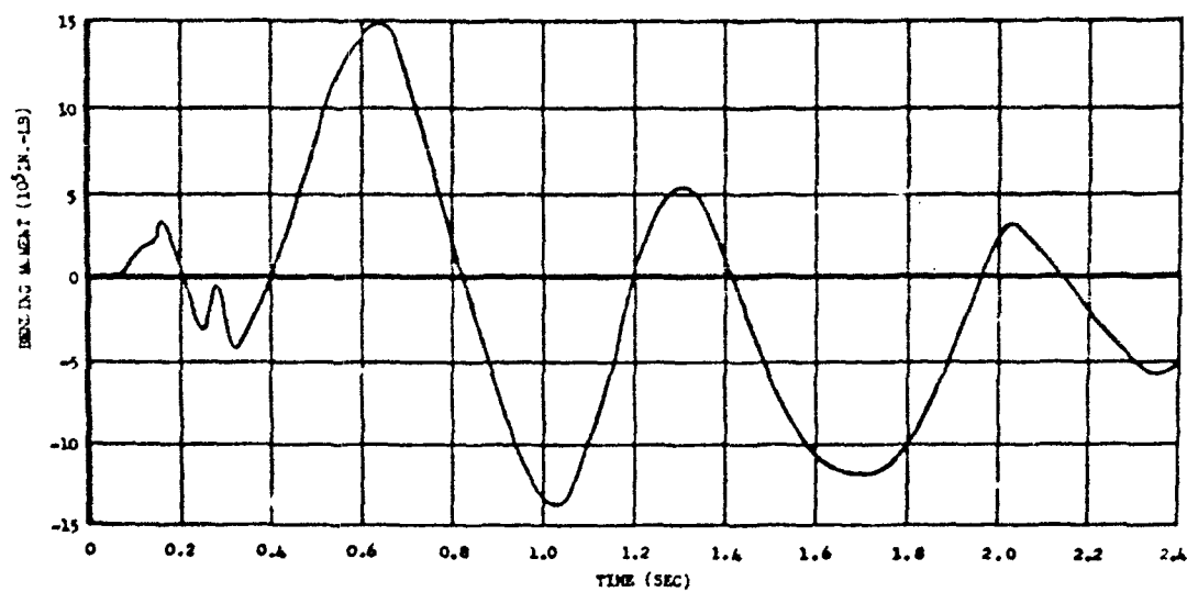
Fig. 4.3 Wing Bending versus Time after Shock Arrival, Right Wing Station 390, E-36D, King Shot
