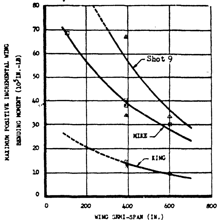
Fig. 6.1 Peak Positive Wing Bending Moments Measure in Mike, King, and Shot 9 Plotted versus Wing Station (Expressed as Distance in Inches from Aircraft Center Line)
