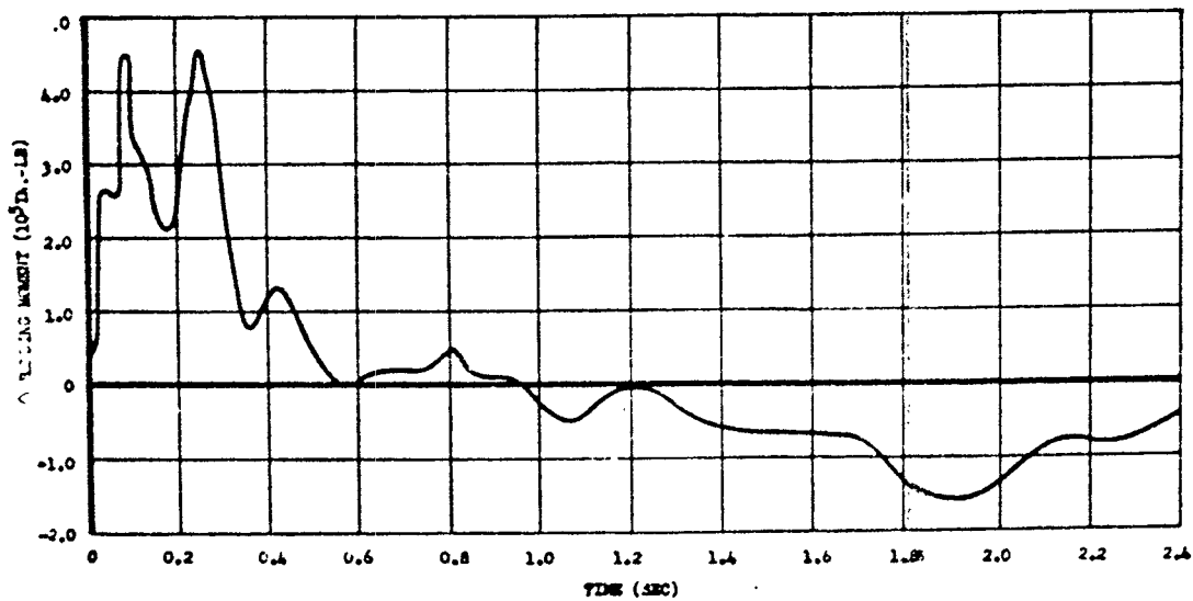
Fig. 4.7 Stabilizer Bending versus Time after Shock Arrival, Left Horizontal Stabilizer Station 62, B-36D, King Shot
