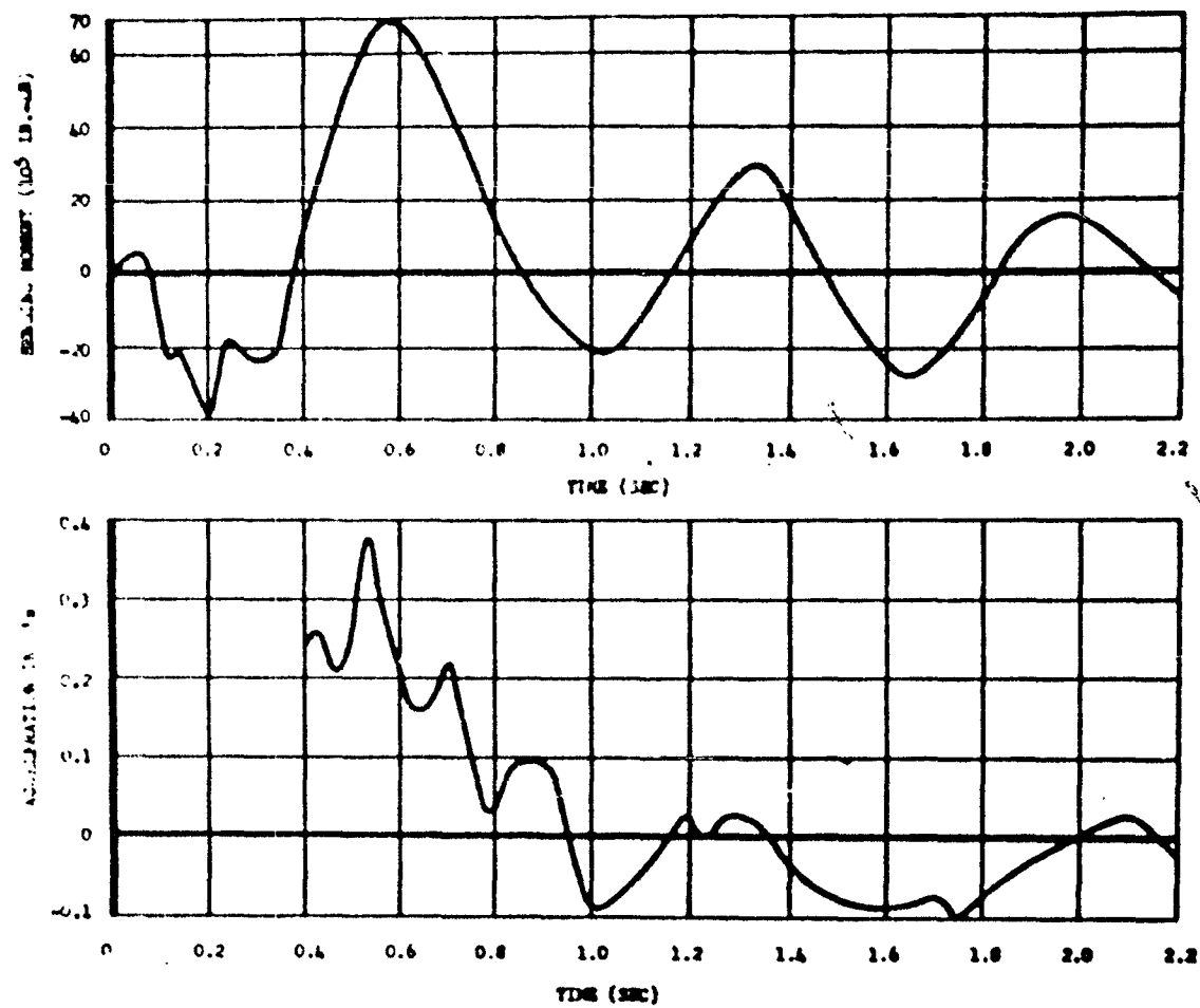
Fig. 6.4 Comparison of Center of Gravity Acceleration Versus Time with Wing Bending (Station 110) Versus Time, B-36D, Mike Shot
