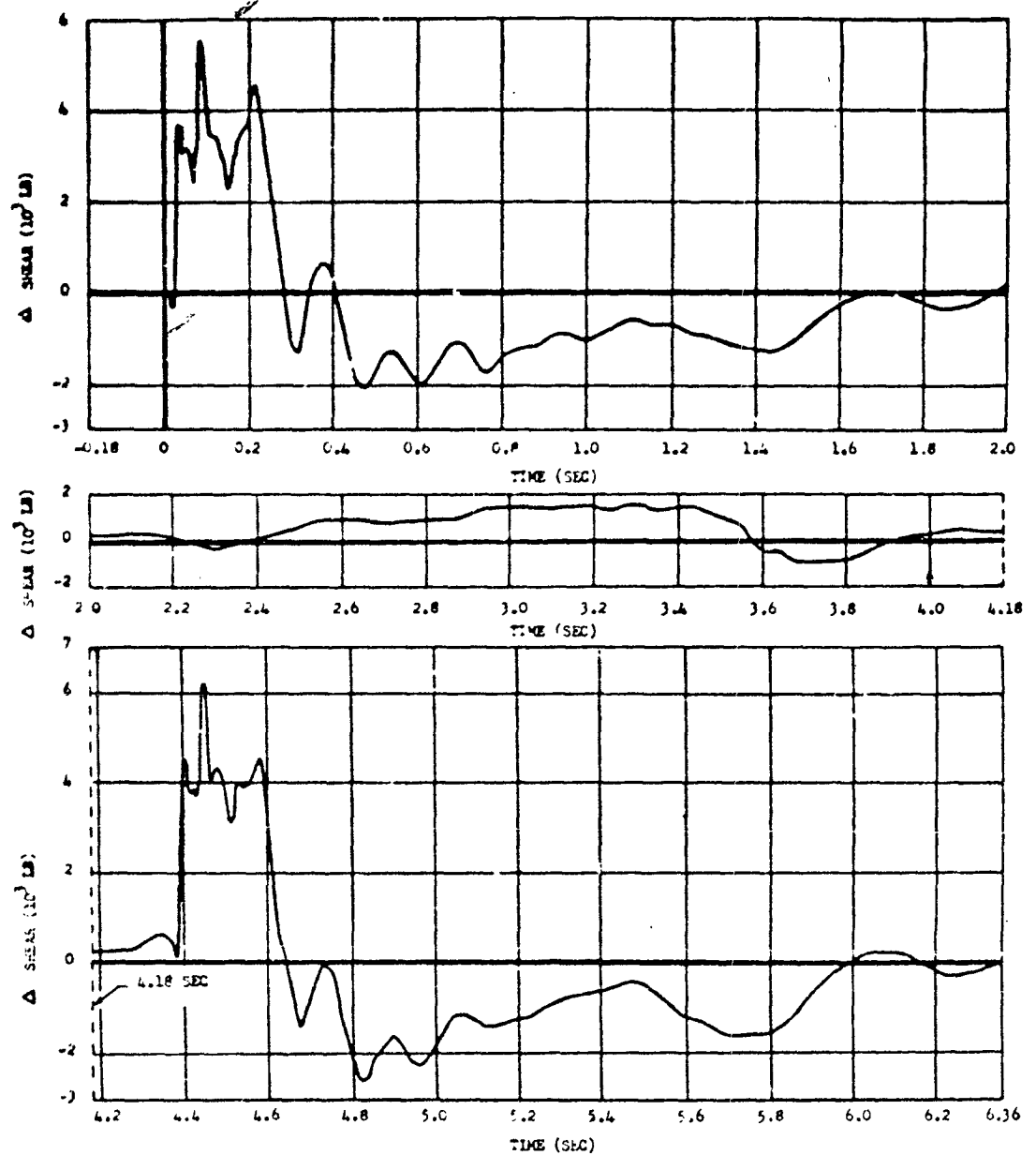
Fig. 5.16 Stabilizer Shear (Point Load Measurement) versus Time after Shock Arrival, Right Horizontal Stabilizer Station 144, B-36D Shot 9
