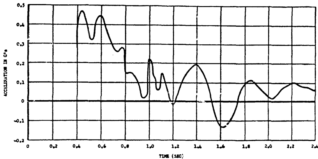
Fig. 3.10 Vertical Acceleration versus Time after Shock Arrival, B-36D Nose, Fuselage Station 212, Mike Shot
