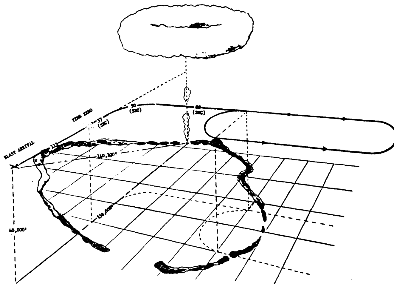
Fig. 2.18 Assigned Position and Flight Pattern of B-36D Aircraft for Mike Shot Showing Flight Times from Leaving Orbit to Blast Arrival
