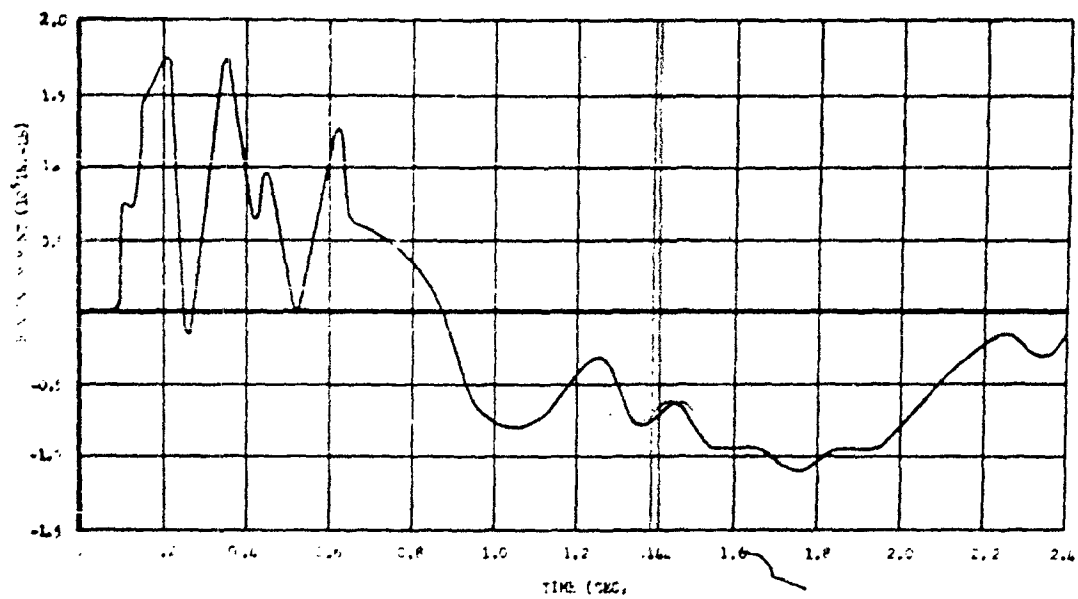
Fig. 4.5 Wing bending versus Time after Shock Arrival, Left Wing Station 1062, B-36D, King Shot
