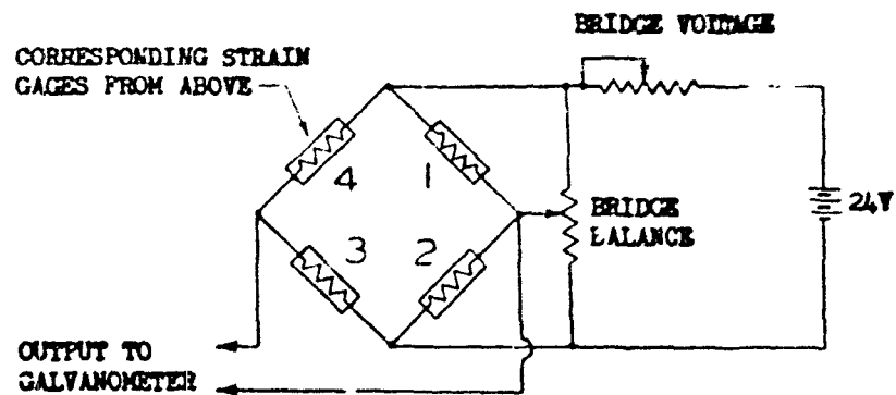
Fig. 2.1 Typical Bending Gage Installation with Schematic Circuit
