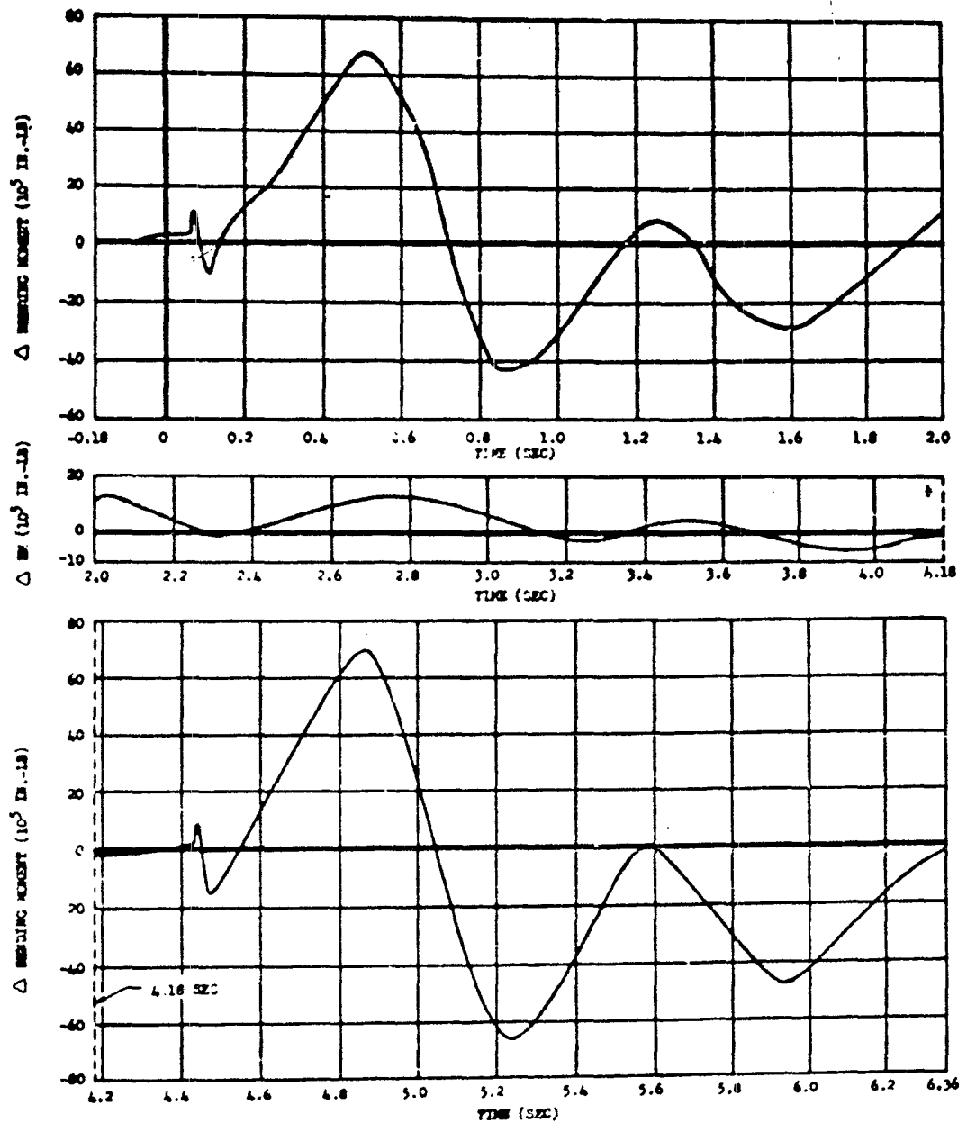
Fig. 5.2 Wing bending versus Time after Shock Arrival, Right Wing Station 390, b-36D, Shot 9
