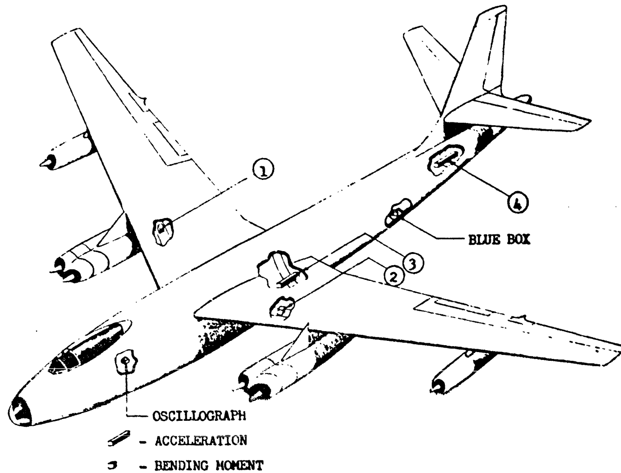
Fig. 2.14 Location of Instrumentation in B-47B Aircraft for IVY
