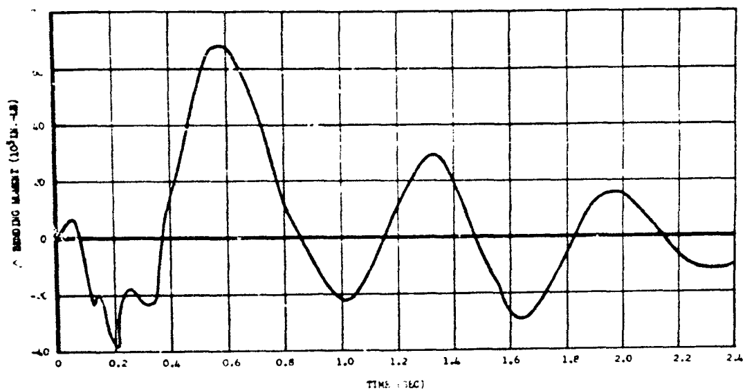
Fig. 3.7 Fuselage Bending versus Time after Shock Arrival, Fuselage Station 1040, B-36D, Mike Shot
