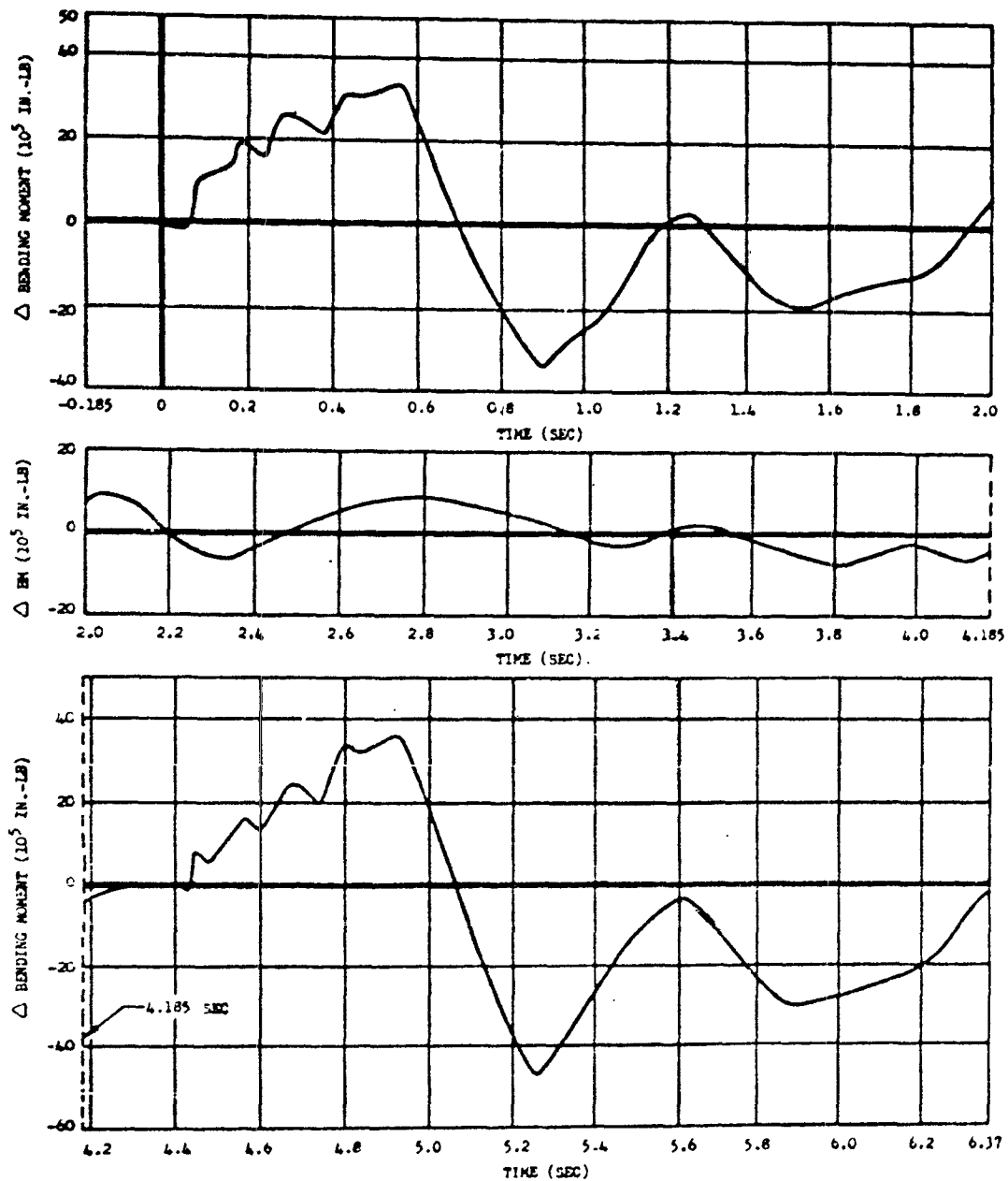
Fig. 5.3 Wing Bending versus Time after Shock Arrival, Left Wing Station 604, B-36D, Shot 9
