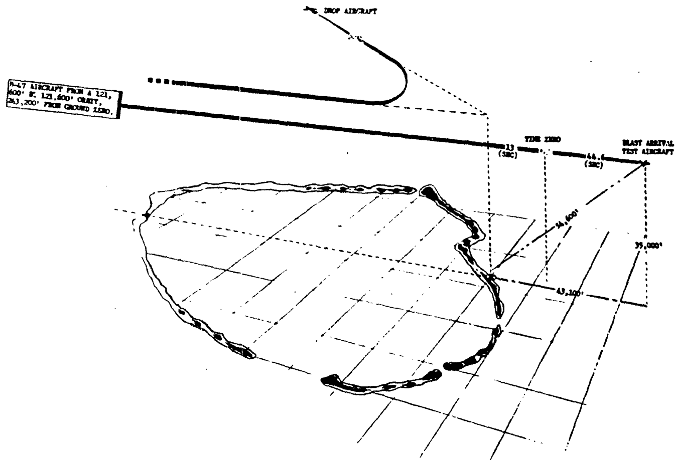
Fig. 2.22 Assigned Position and Flight Pattern of B-47B Aircraft for King Shot
