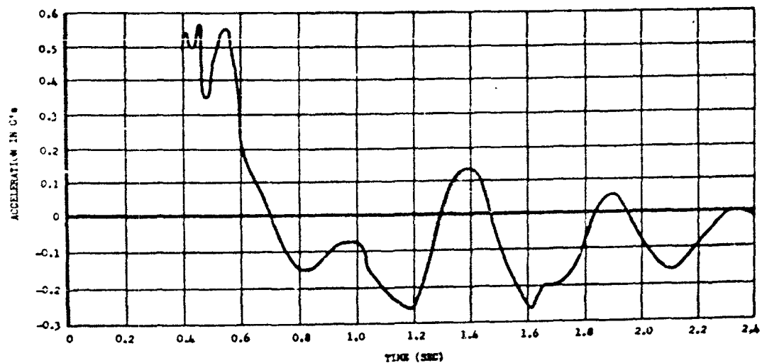
Fig. 3.9 Vertical Acceleration versus Time after Shock Arrival, B-36D Tail, Fuselage Station 1770, Mike Shot
