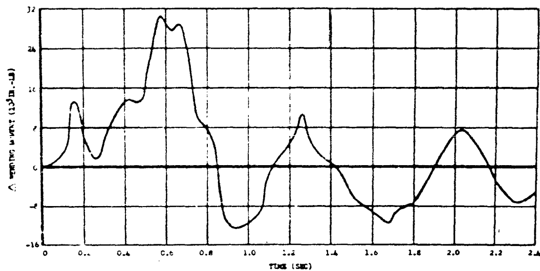
Fig. 3.5 Wing bending versus Time after Shock Arrival, Left Wing Station 604, B-36D, Mike Shot
