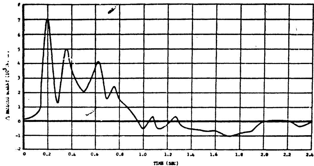
Fig. 3.6 Wing Bending versus Time after Shock Arrival, Left Wing Station 1062, B-36D, Mike Shot
