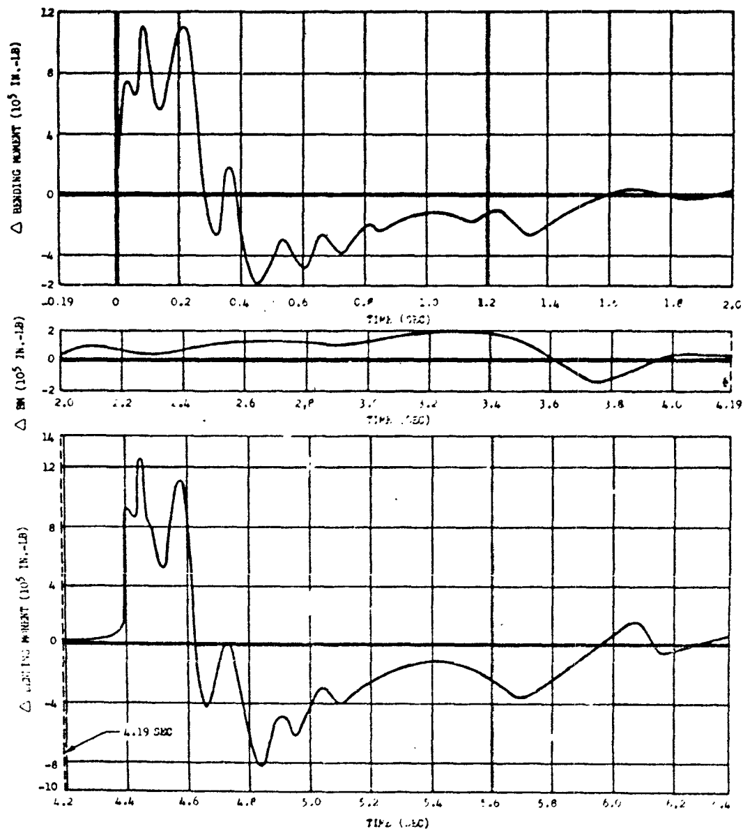
Fig. 5.6 Stabilizer Bending versus Time after Shock Arrival, Left Horizontal Stabilizer Station 62, B-36D, Shot 9
