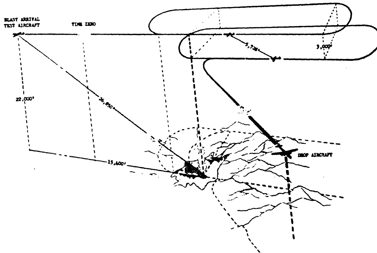
Fig. 2.20 Assigned Position and Flight Pattern of B-36D Aircraft for Shot 9
