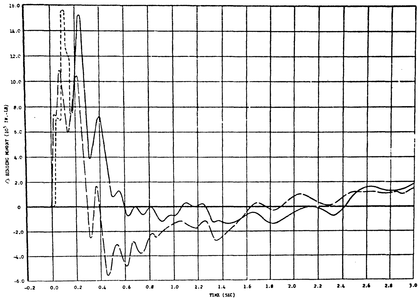
Fig. 6.2 Comparison of Bending Measurements made at Station 62 of the Left Horizontal Stabilizer, B-36D during Mike and Shot 9
