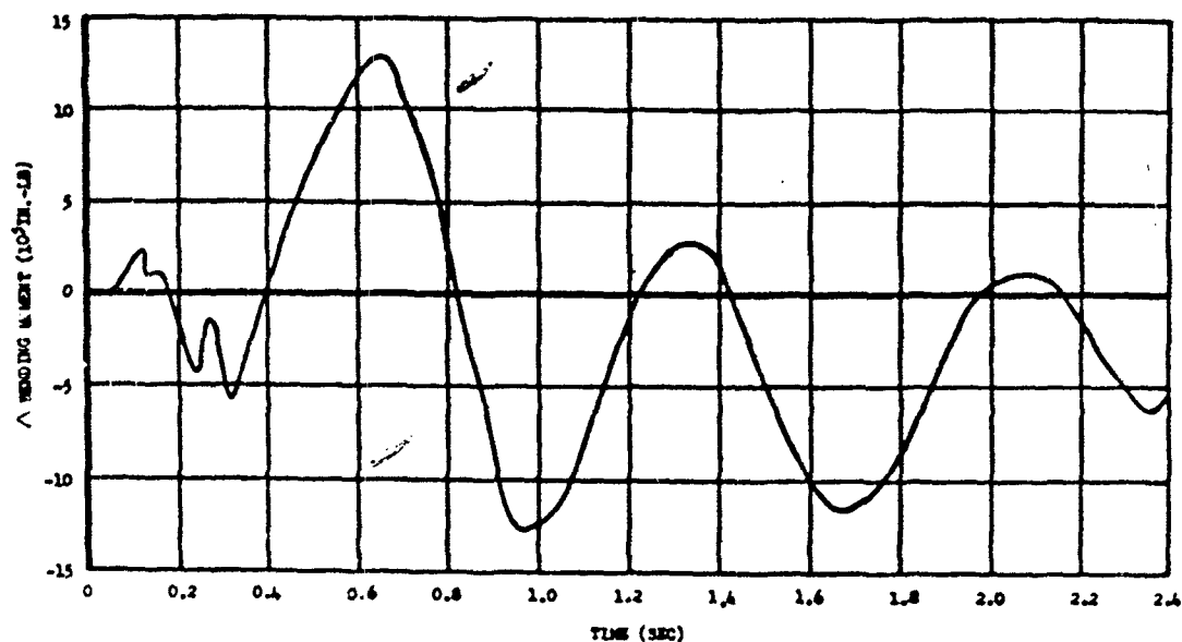
Fig. 4.2 Wing Bending versus Time after Shock Arrival, Left Wing Station 390, E-36D, King Shot
