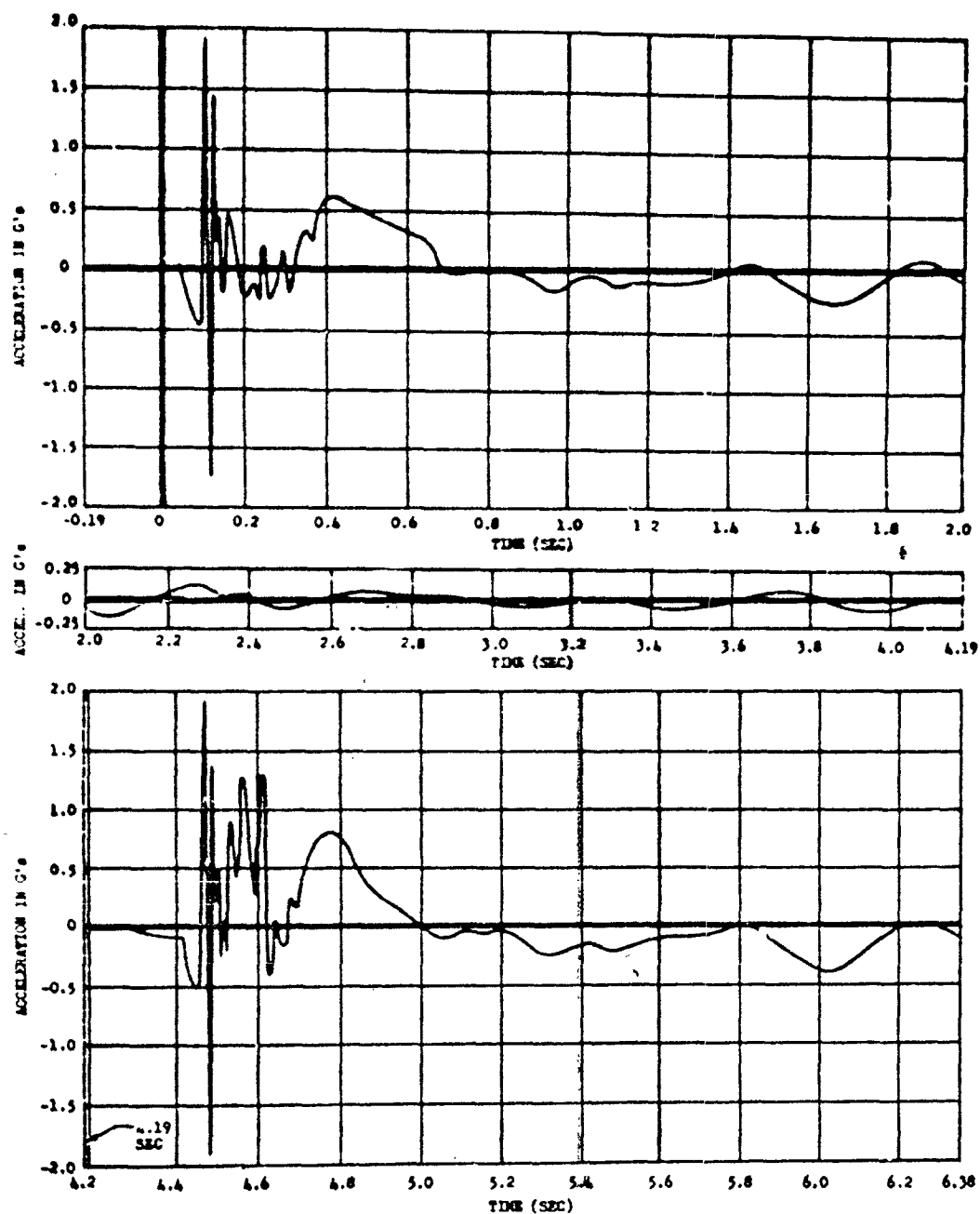
Fig. 5.12 Vertical Acceleration versus Time after Shock Arrival, B-36D Nose, Fuselage Station 212, Shot 9
