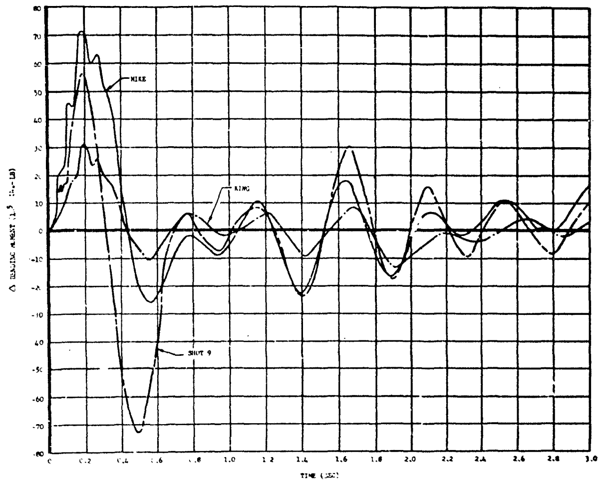
Fig. 6.3 Comparison of Fuselage Bending Measurements made at Station 1040 on the B-36D during Mike, King and Shot 9
