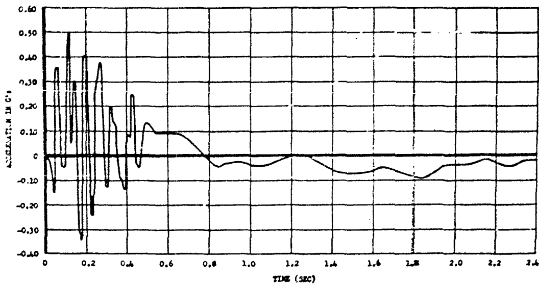
Fig. 4.11 Vertical Acceleration versus Time after Shock Arrival, B-36D Center of Gravity, Fuselage Station 907 (Right Side), King Shot
