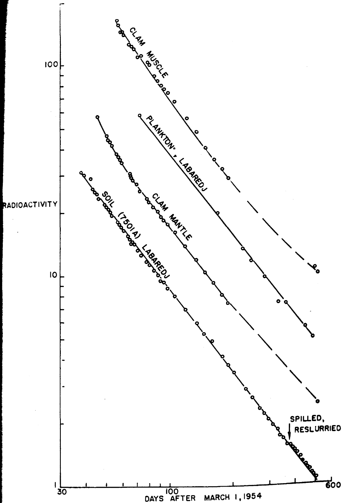
FIG. 12 LOG-LOG PLOTS OF RONGELAP DECAY SAMPLES OF MARCH 26, 1954: PLANKTON FROM LABAREDJ; MUSCLE AND MANTLE OF GIANT CLAM, HIPPOPUS, FROM KABELLE; AND SOIL ON WHICH DECAY CORRECTION FACTORS WERE BASED
