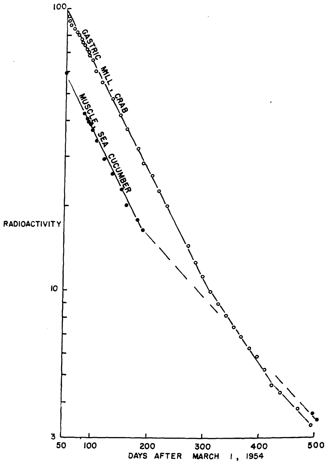
FIG. II SEMI-LOG PLOTS OF DECAY CURVES OF GASTRIC MILL OF CRAB, GRAPSUS GRAPSUS , AND MUSCLE OF SEA CUCUMBER, HOLOTHURIA ATRA COLLECTED MARCH 26, 1954 AT KABELLE
