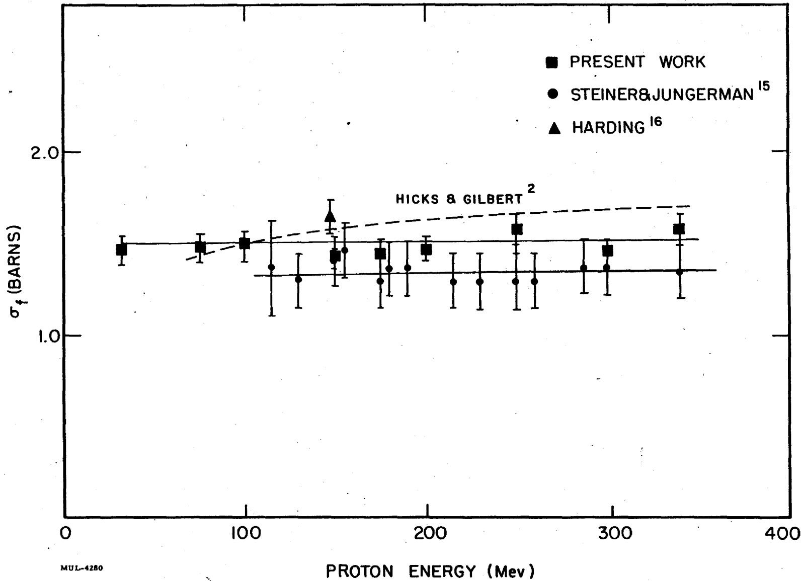
Fig. 3. Fission cross section of U^{238} bombarded with protons of various energies.
