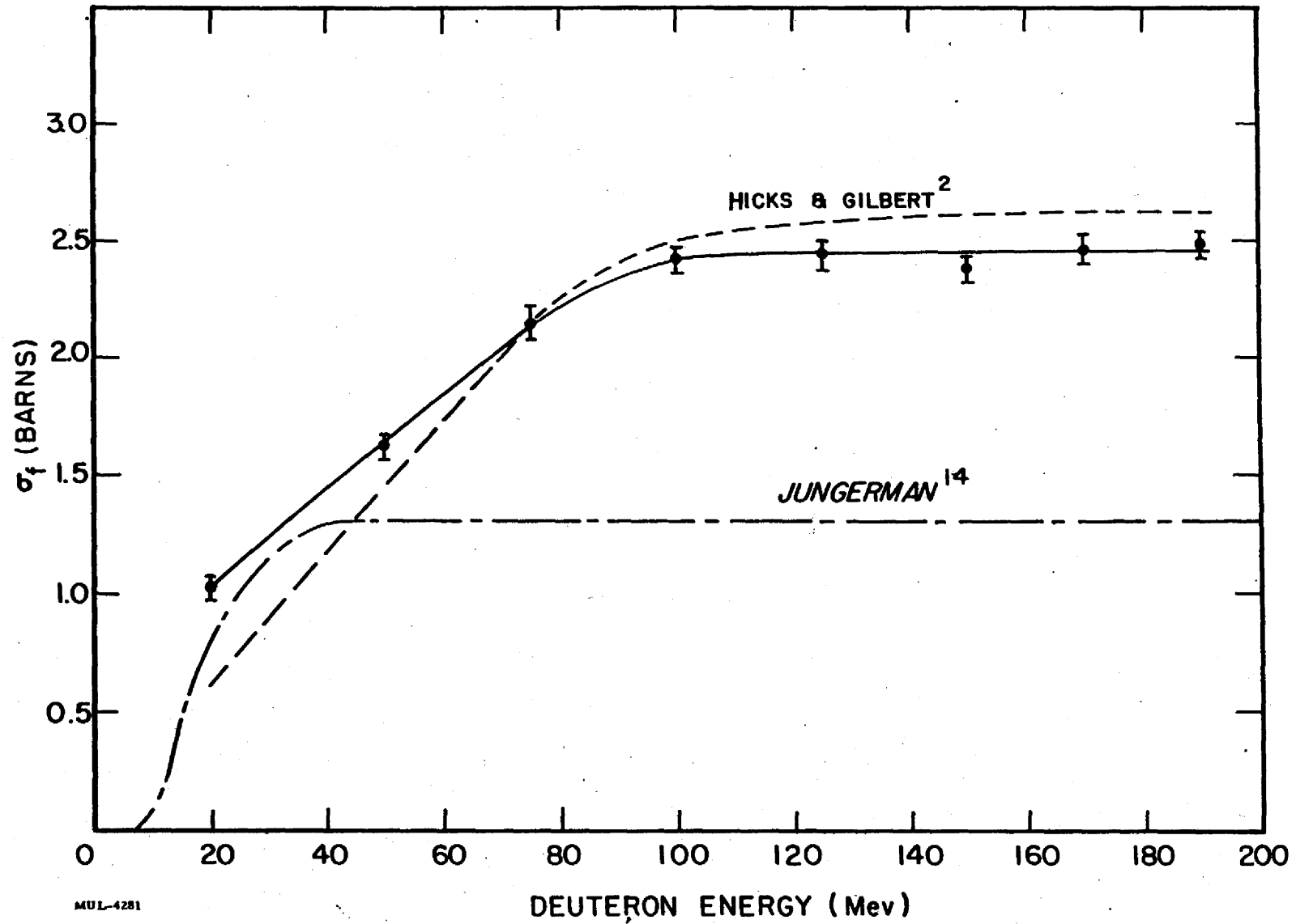
Fig. 4. Fission cross section of U^{238} bombarded with deuterons of various energies.
