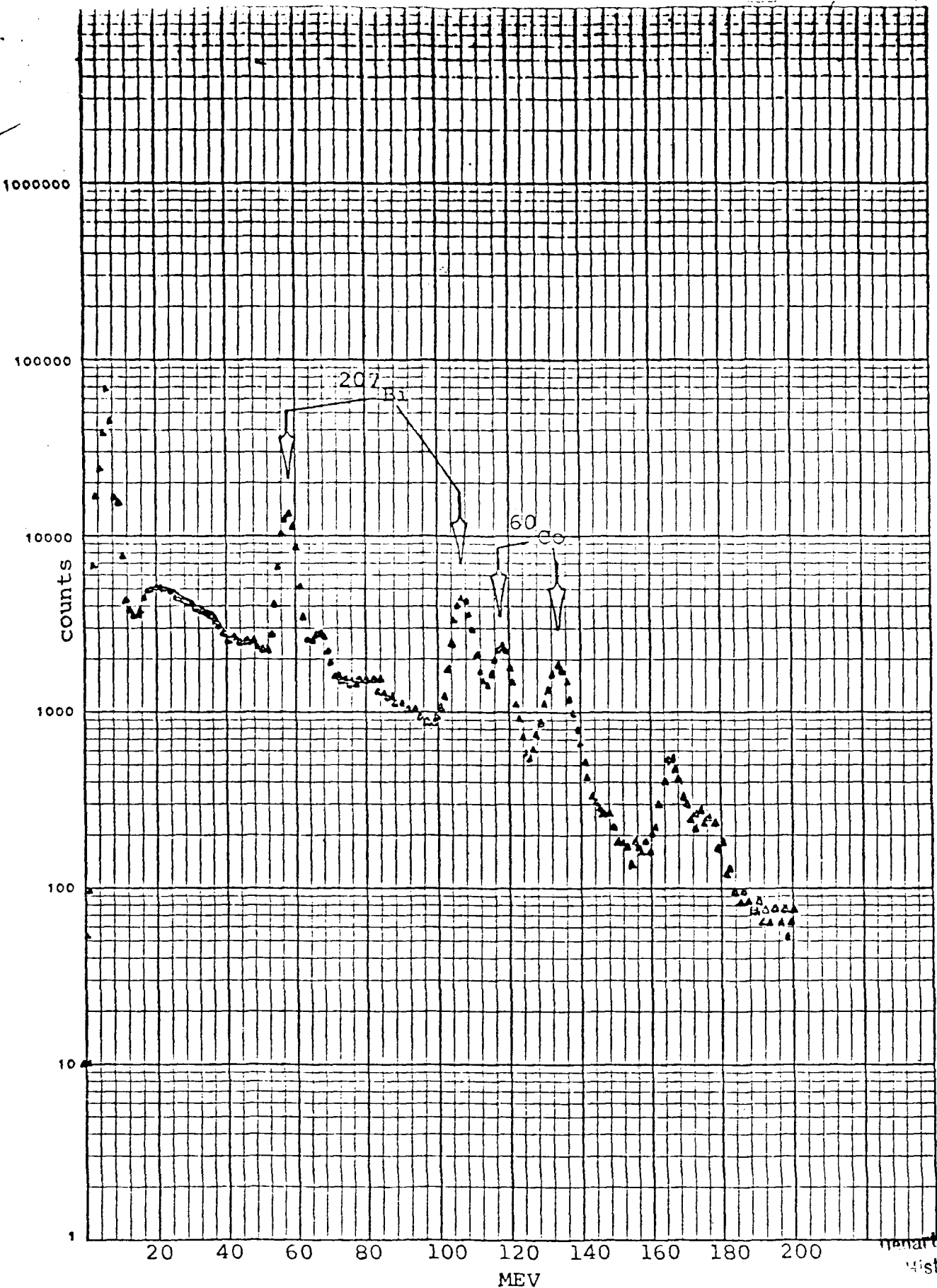
Fig. 1. Gamma-ray spectrum of sediment from Bravo Crater collected at a water depth of 160 feet, August, 1969.
