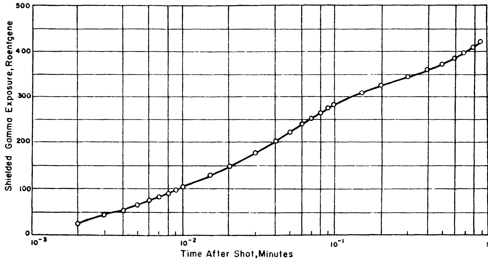
Figure 3.26 Shielded initial exposure versus time for Shot Zuni; Station 220.09C, range 7,000 feet. For unshielded exposure multiply by 1.2.
