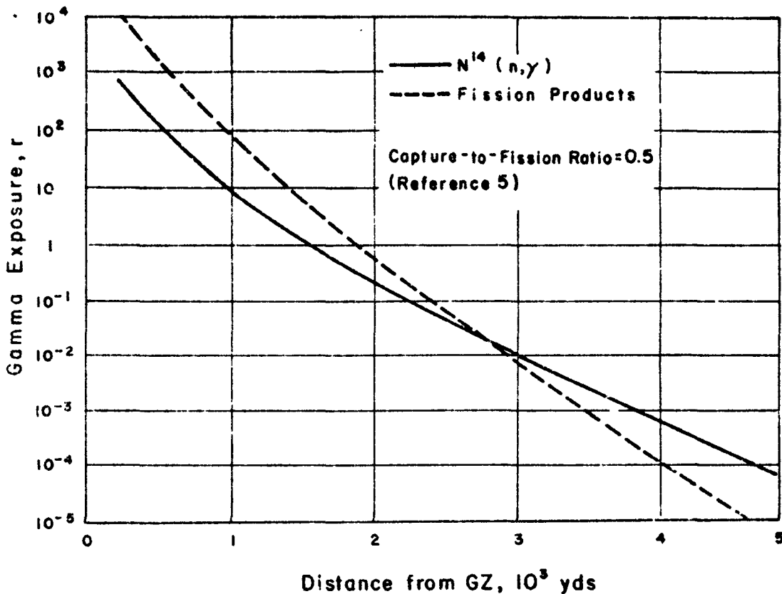
Figure 1.1 Graph of gamma exposure versus distance for a one kt surface burst. This illustration shows the contribution from fission-product gammas.
