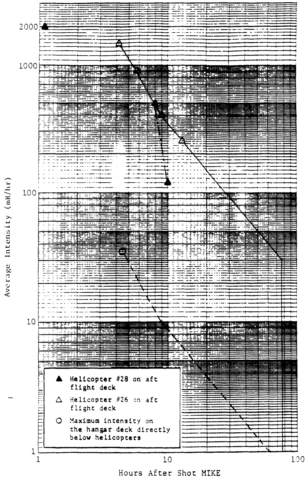
Figure 1. Intensity on aft flight deck and hangar deck of USS RENOVVA (CVE-114) 1-4 November 1952.
