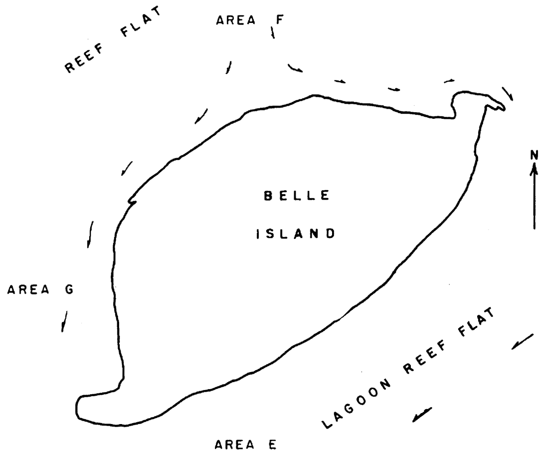
Fig. 1. Map of the north reef and islands of Eniwetok Atoll (top) with an enlarged map of Belle Island (bottom) showing typical current patterns. The wind rose indicates prevailing winds.
