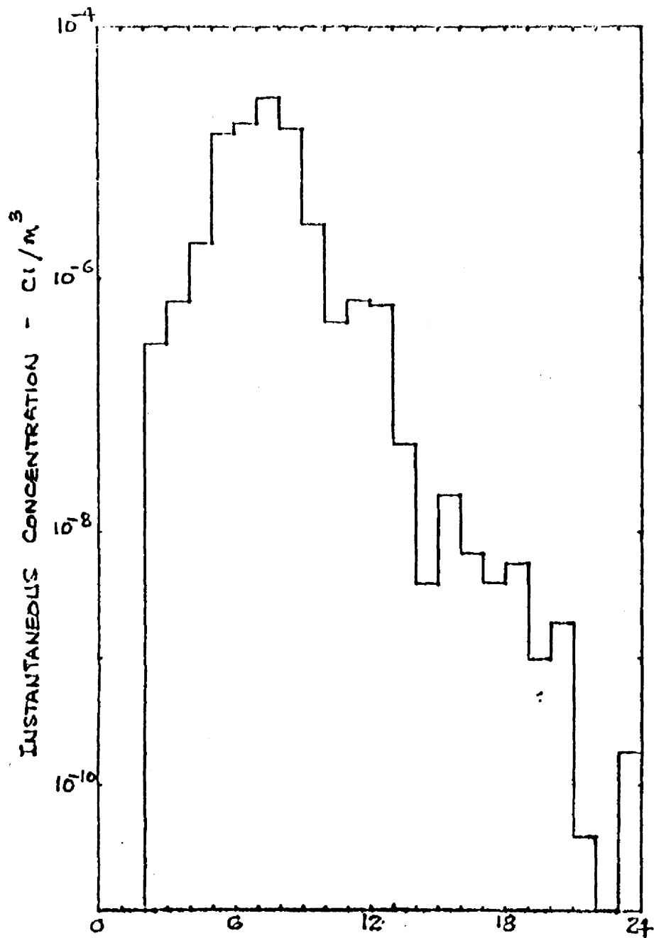
Figure 3c. Same as Fig. 3a, except nuclide is iodine-133.
