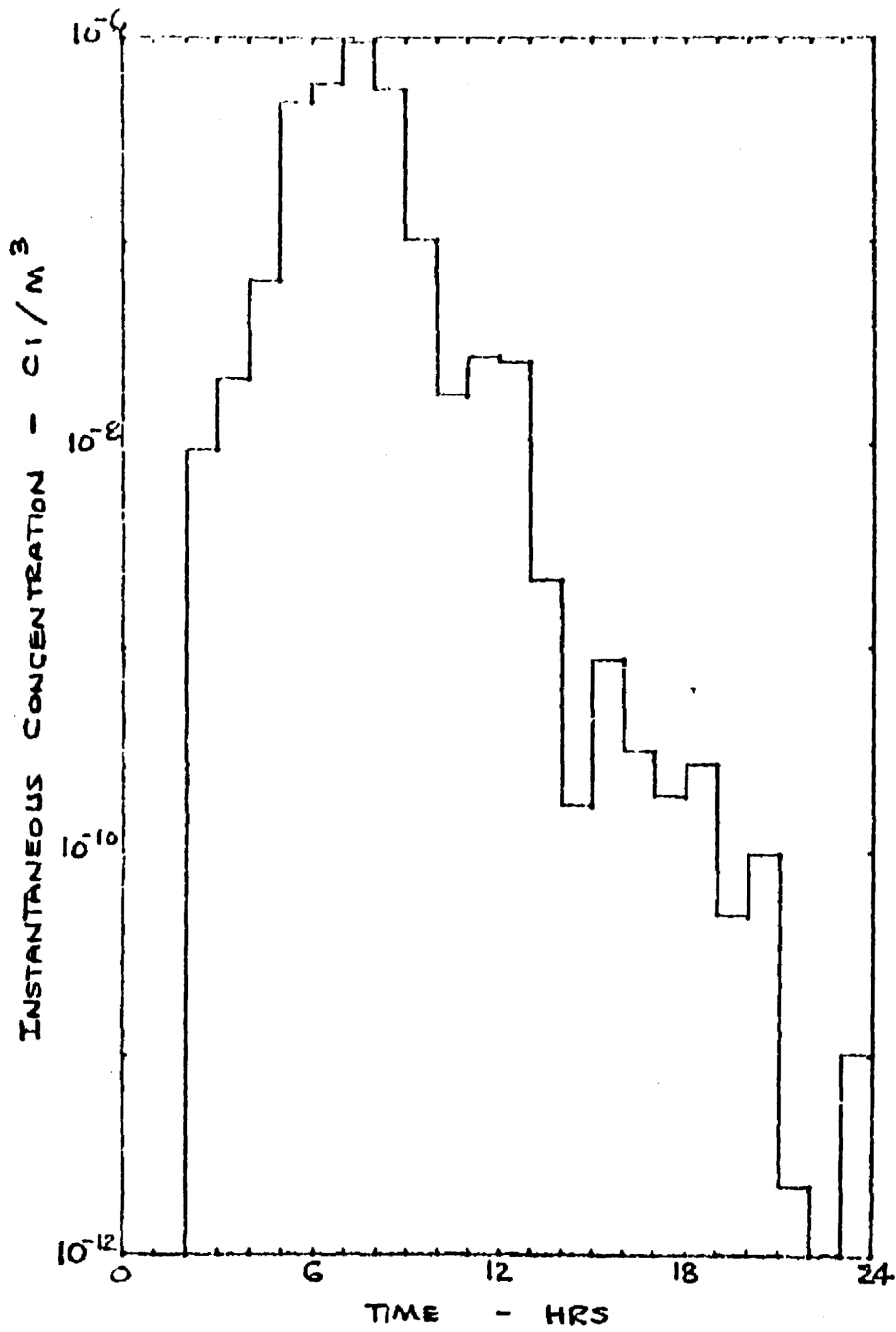
Figure 3b. Same as Fig. 3a, except nuclide is iodine-131.
