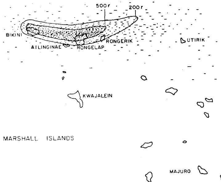
FIGURE 2. Map of fallout area, Marshall Islands, March 1954.
