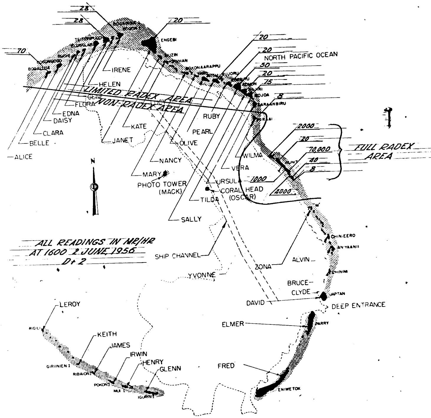
Fig. 0-5 RadSafe Survey, D + 2
