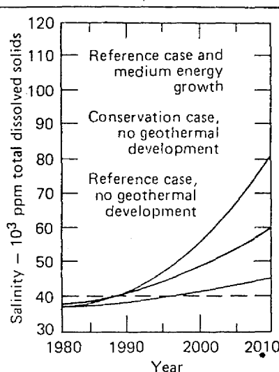
Fig. 3 Salinity of the Salton Sea predicted for three cases: existing irrigation efficiencies (reference case), improved efficiencies (conservation case), and a reference case with growth in geothermal energy-generating capacity of 100 MW/yr and the use of agricultural waste waters for cooling. Predictions are based on normal hydrologic conditions and average evapotranspiration from crops. Toxic effects on fish reproduction are expected when the concentration of total dissolved solids exceeds 40 000 ppm (dashed line).
