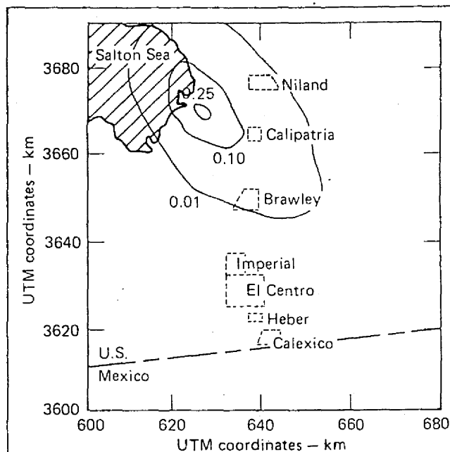
Fig. 2 Isopleth plot showing estimates of how much of the time the California air-quality standard for hydrogen sulfide ( 42 \mu\text{g}/\text{m}^3 averaged over one hour) would be exceeded in the Imperial Valley, assuming a geothermal production capacity of 3000 MW. (Along a 1.0 isopleth, the standard is exceeded all the time, along a 0.25 isopleth the standard is exceeded one-fourth of the time, etc.) To prevent violations of the hydrogen sulfide standard at that level of energy development, facilities in the Salton Sea and Brawley resource areas would have to reduce emissions by approximately 82%.
