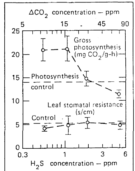
Fig. 2 Photosynthesis rates ( \text{mg CO}_2/\text{g-h} ) and stomatal resistance (s/cm) in lettuce exposed (for 3 h at 30°C and high light) to a mixture of gases similar to that emitted by geothermal power plants. Geothermal emissions actually stimulate photosynthesis at low concentrations because the additional carbon dioxide and hydrogen sulfide provide essential elements for carbohydrate and amino acid production. The first significant decrease in photosynthesis occurs when hydrogen sulfide exceeds about 3 ppm in this mixture.
