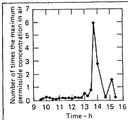
Fig. 5 The TAMS system was fielded and tested at the Rockwell Hanford Operation plutonium-recovery facility's Z-plant (in Richland, Washington) during the summer of 1978. In these tests, it demonstrated a sensitivity 100 times that of any commercially available alpha-measurement system. Shown here is the combined concentration of plutonium-238, plutonium-239, and americium-241 in the sampled stack exhaust while a high-efficiency air particulate filter was being changed on July 10, 1978. Clearly, a low-level release is taking place. Normal dilution factors for this stack are such that a stack concentration of 50 times the maximum permissible concentration is reduced to below 2.5 before it reaches man. Man can be exposed to 100 times the maximum permissible concentration in air for up to 160 hours before the maximum allowed body dose is approached.
