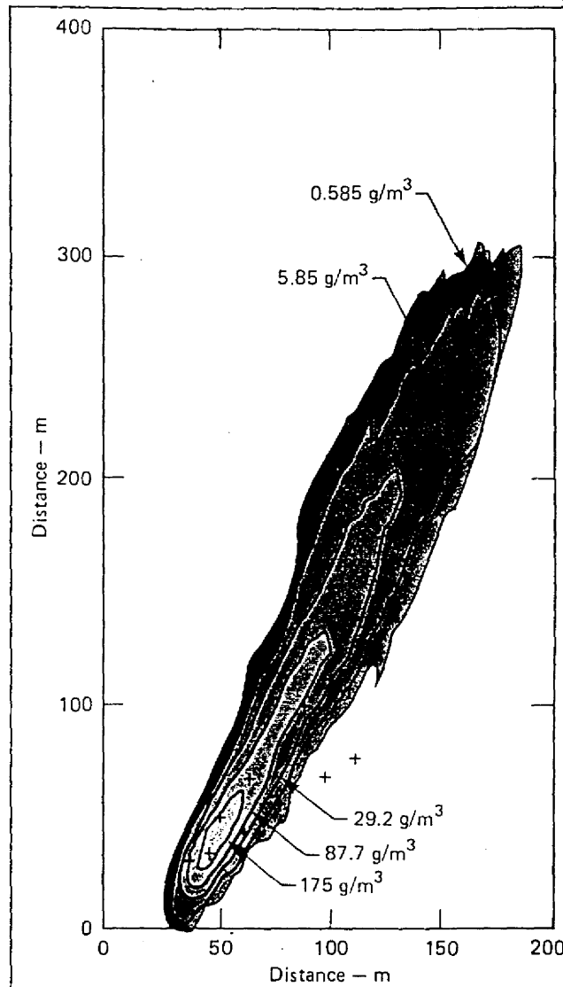
Fig. 2 Concentration isopleths calculated by the ATMAS code for the vapor plume 60 s after the start of the first 5-m 3 spill experiment. The lower flammability limit (33 g/m 3 at 300 K) eventually extended to about 380 m.
