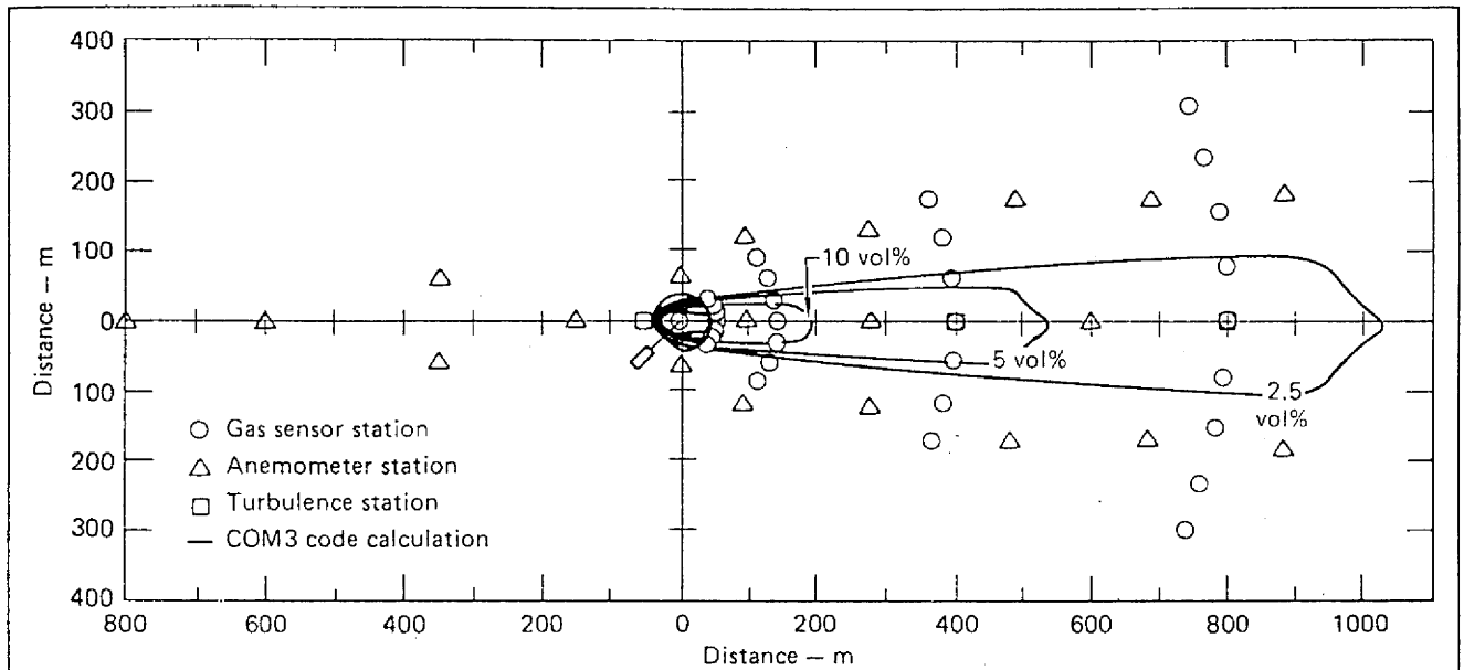
Fig. 6 Far-field dispersion array for 40-m 3 spill tests at China Lake, with calculated concentration contours for a 40-m 3 /min spill rate. Gas sensors, anemometers, and thermocouples are at elevations of 1, 3, and 8 m above the ground. Each of the instrument stations
