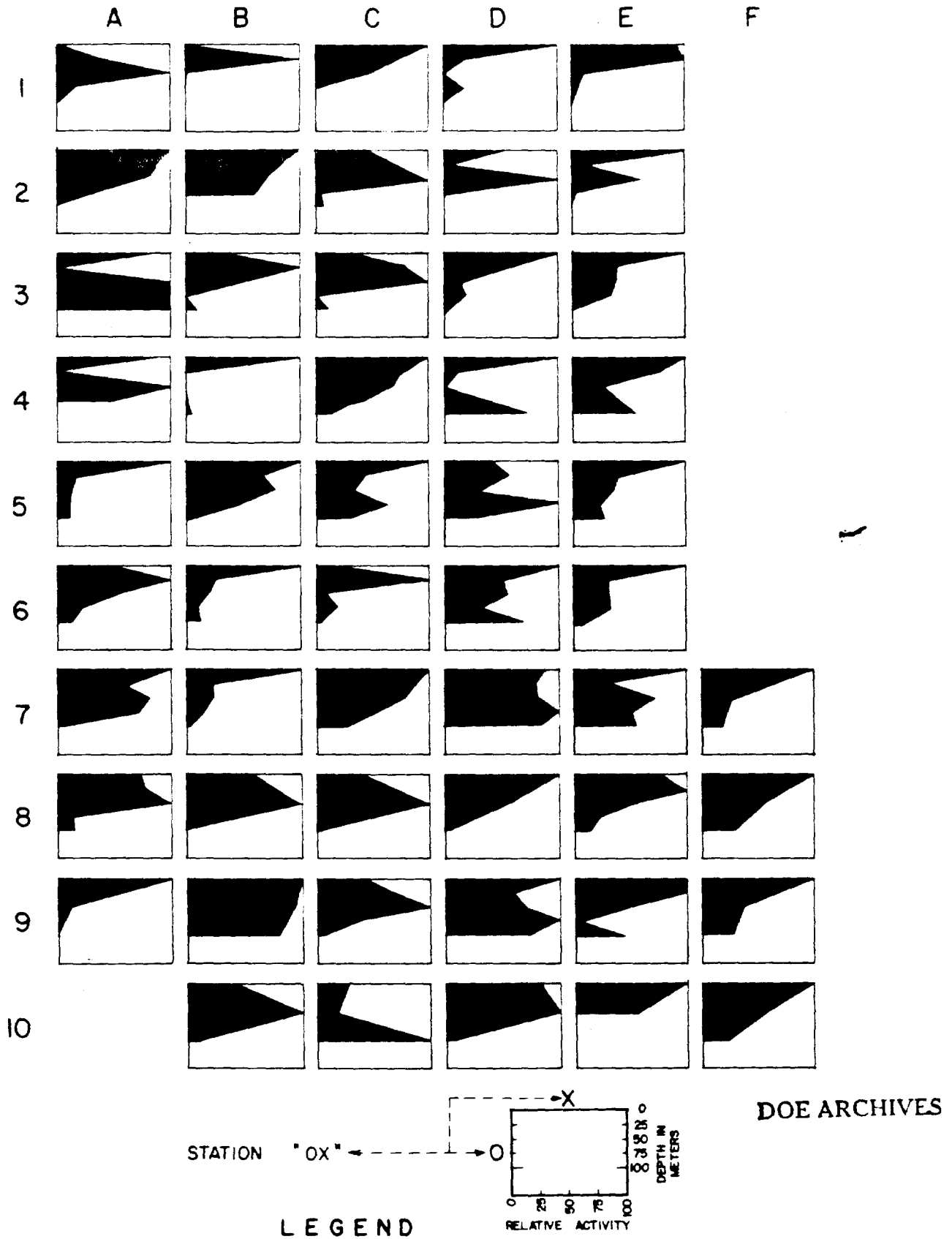
Fig. 9. Relative radioactivity of water (filter and filterable fraction, less K^{40} ) at each depth sampled. Maximum value at each station taken as 100. Walton samples.
