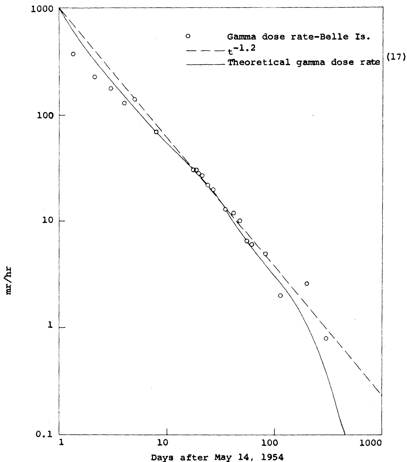
Figure 3. Gamma dose rates at three feet at Belle Island, Eniwetok Atoll, May 15, 1954 to March 21, 1955, compared with the slope of t^{-1.2} and the decay of fission products from the slow neutron fission of U^{235} (17)
